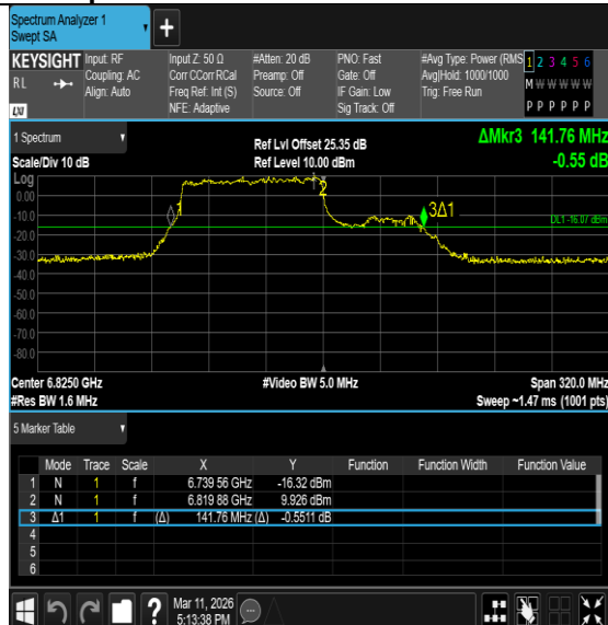
11BE160MIMO-Ant6-6825-996Tone-RU68-PASS
