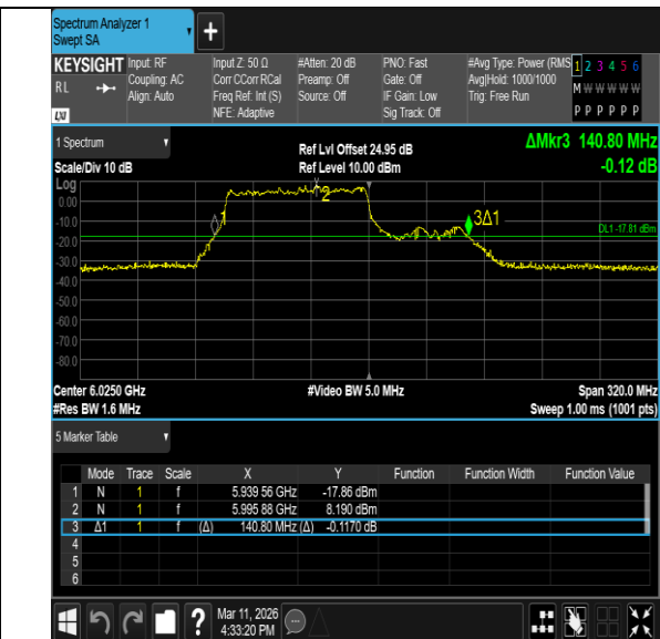
11BE160MIMO-Ant7-6025-996Tone-RU68-PASS
