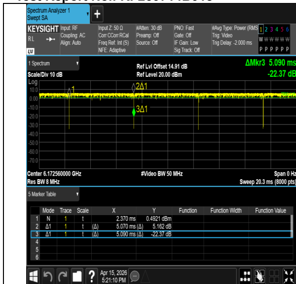
NTNV-11BE20MIMO-Ant6-6175-52Tone-RU40
