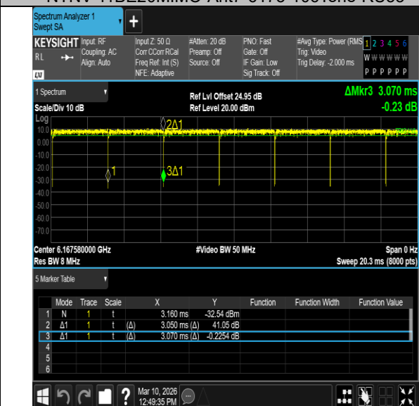
NTNV-11BE20MIMO-Ant7-6175-106Tone-RU53
