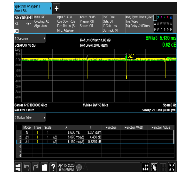
NTNV-11BE20MIMO-Ant7-6175-52Tone-RU40
