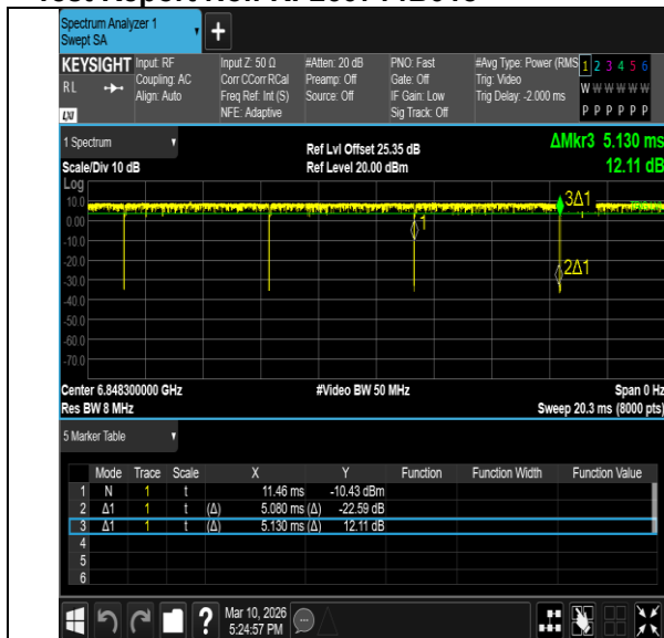
NTNV-11BE20MIMO-Ant6-6855-52Tone-RU38
