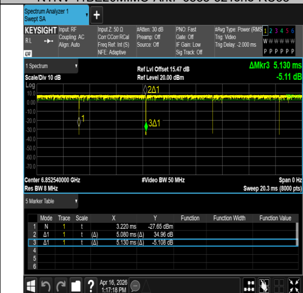
NTNV-11BE20MIMO-Ant7-6855-52Tone-RU40
