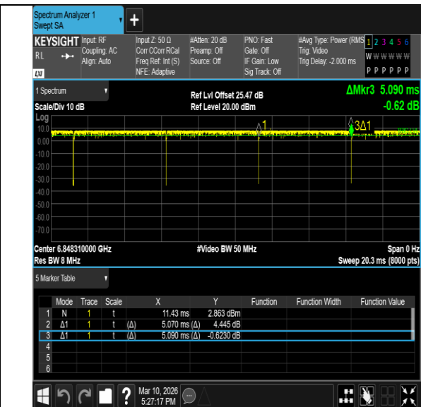
NTNV-11BE20MIMO-Ant7-6855-52Tone-RU38
