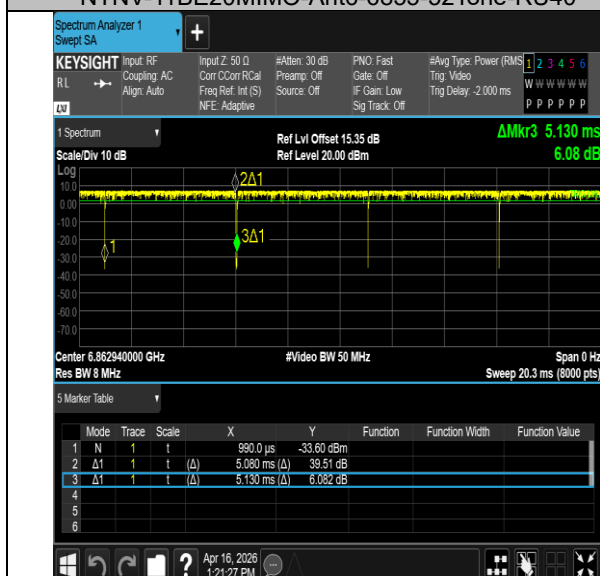
NTNV-11BE20MIMO-Ant6-6855-52Tone-RU40
