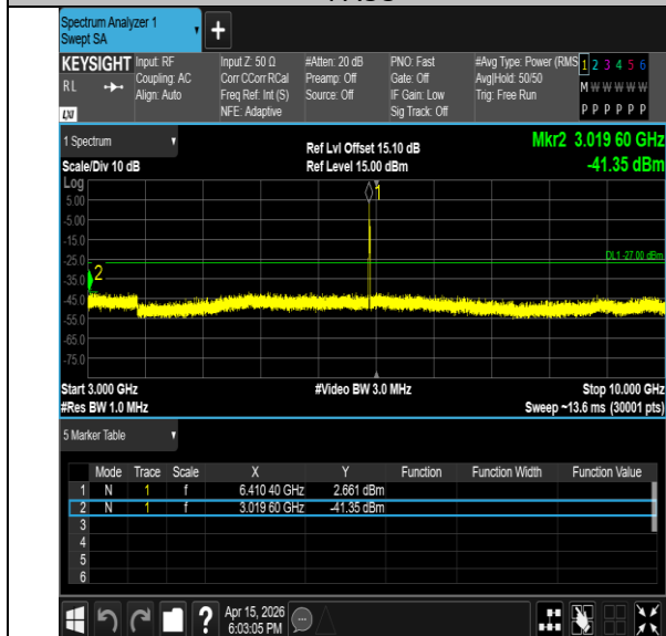
11BE20MIMO-Ant6-6415-52Tone-RU40-3000~10000-PASS
