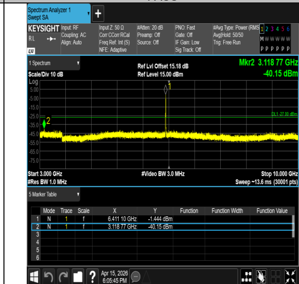
11BE20MIMO-Ant7-6415-52Tone-RU40-3000~10000-PASS
