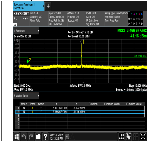
11BE20MIMO-Ant6-6415-52Tone-RU38-3000~10000-PASS
