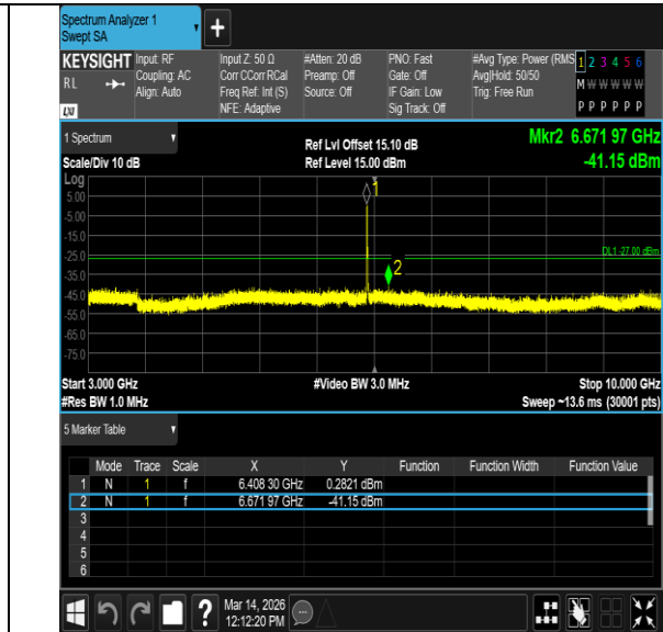
11BE20MIMO-Ant7-6415-52Tone-RU38-3000~10000-PASS
