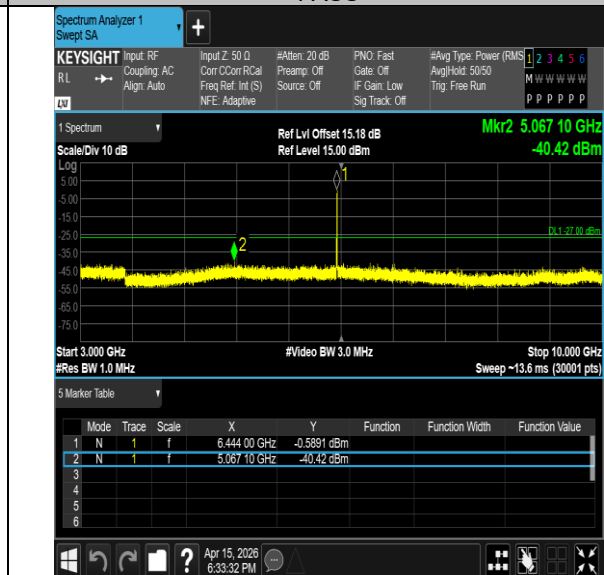
11BE20MIMO-Ant7-6435-52Tone-RU37-3000~10000-PASS
