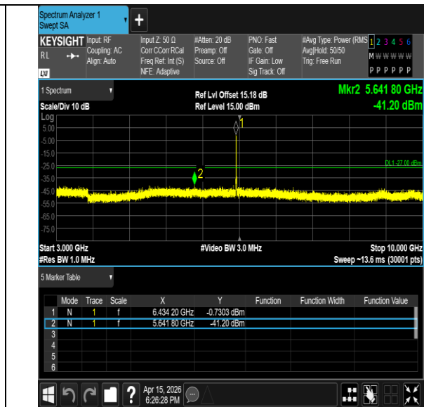
11BE20MIMO-Ant7-6435-26Tone-RU8-3000~10000-PASS
