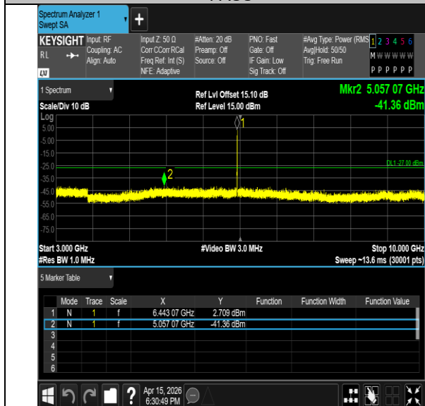
11BE20MIMO-Ant6-6435-52Tone-RU37-3000~10000-PASS
