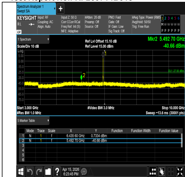
11BE20MIMO-Ant6-6435-26Tone-RU8-3000~10000-PASS
