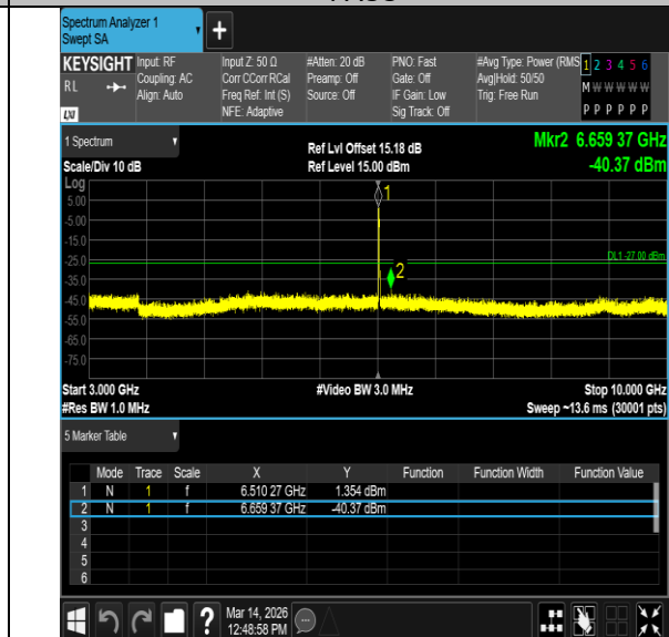
11BE20MIMO-Ant7-6515-106Tone-RU54-3000~10000-PASS
