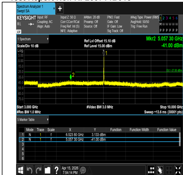
11BE20MIMO-Ant6-6515-106Tone-RU53-3000~10000-PASS
