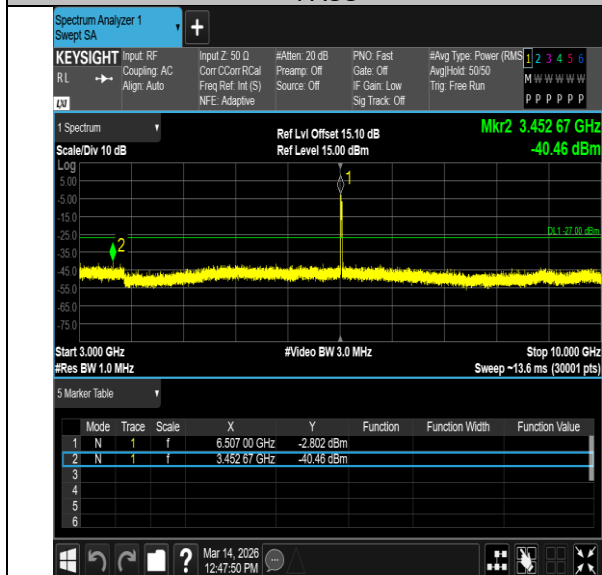
11BE20MIMO-Ant6-6515-106Tone-RU54-3000~10000-PASS
