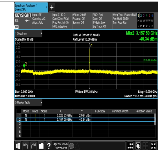
11BE20MIMO-Ant7-6515-106Tone-RU53-3000~10000-PASS
