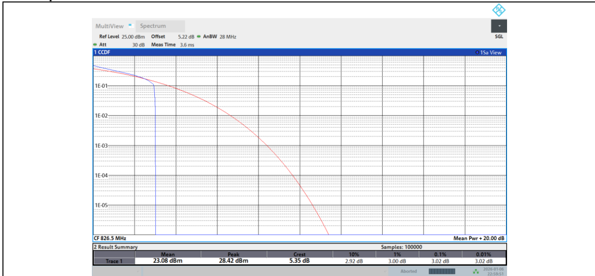
Band 26-5M-LOW-64QAM-1RB Low
