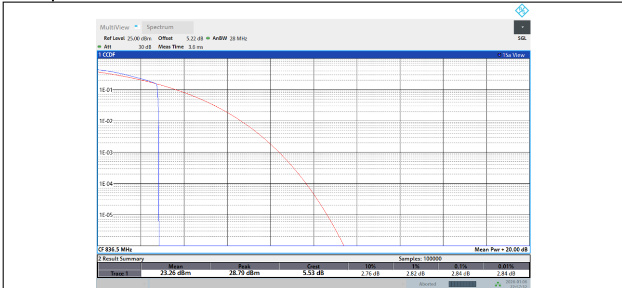
Band 26-3M-MID-64QAM-Full RB
