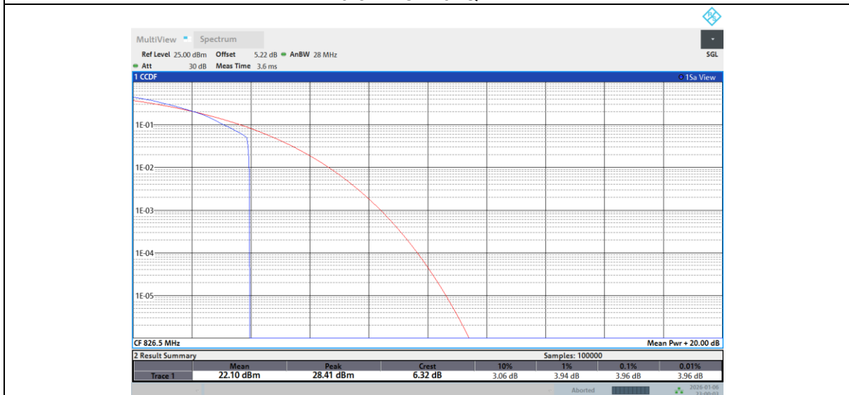
Band 26-5M-LOW-64QAM-Full RB
