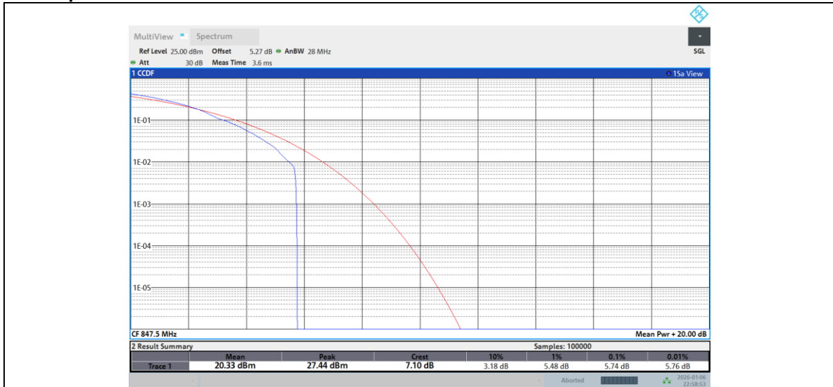
Band 26-3M-HIGH-256QAM-Full RB
