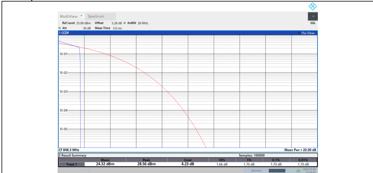
Band 26-1.4M-HIGH-QPSK-Full RB
