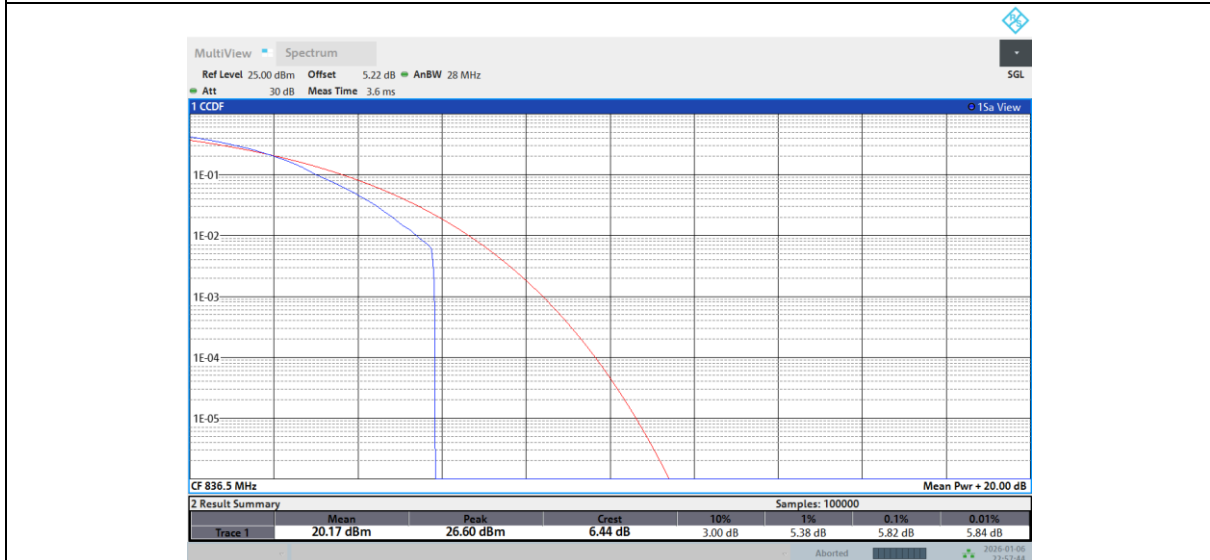
Band 26-3M-MID-256QAM-1RB Low
