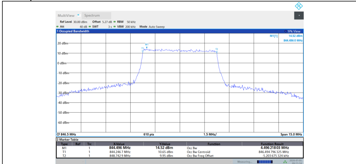
Band 26-5M-HIGH-256QAM-Full RB
