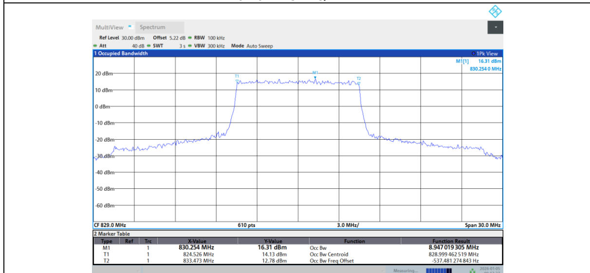
Band 26-10M-LOW-QPSK-Full RB
