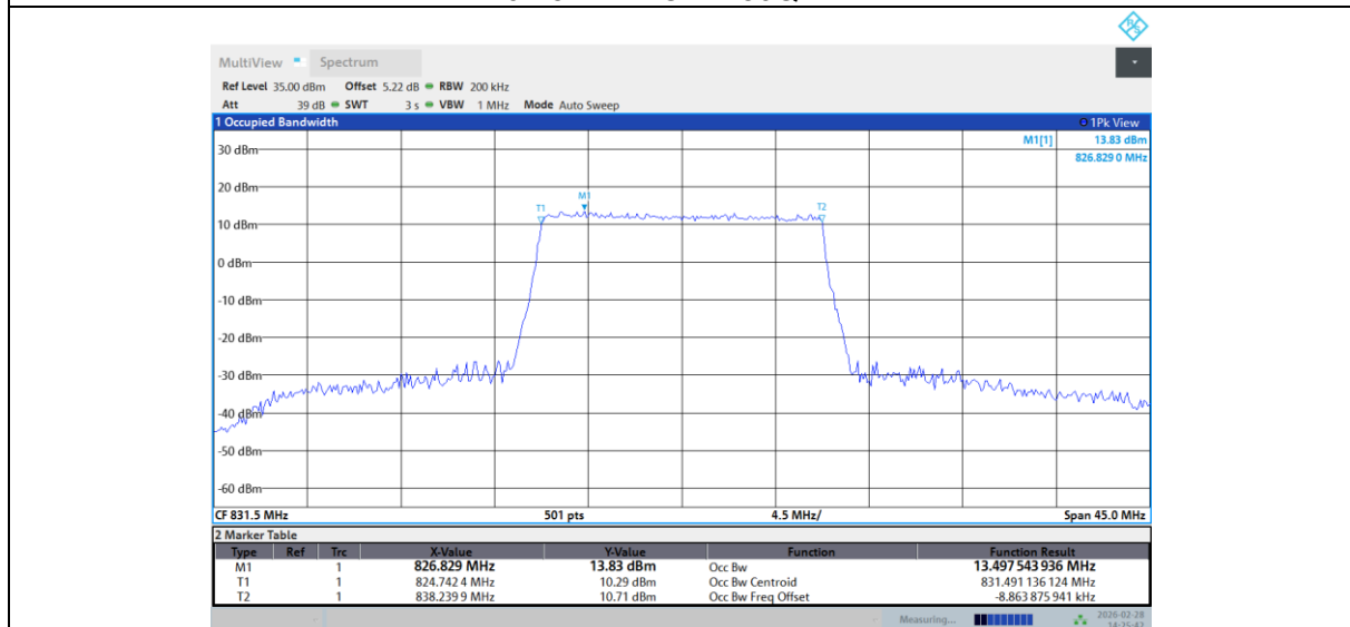
Band 26-15MHz-LOW-256QAM-Full RB
