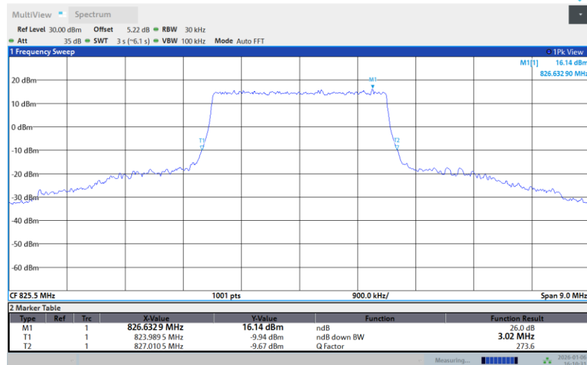
Band 26-3M-LOW-64QAM-Full RB
