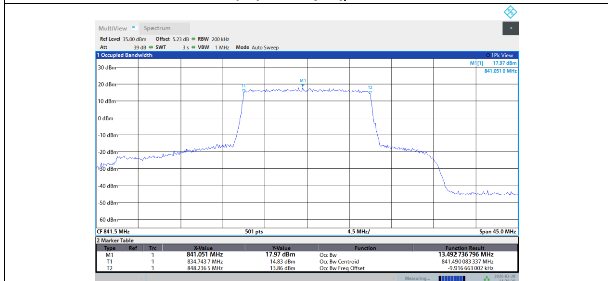
Band 26-15MHz-HIGH-QPSK-Full RB
