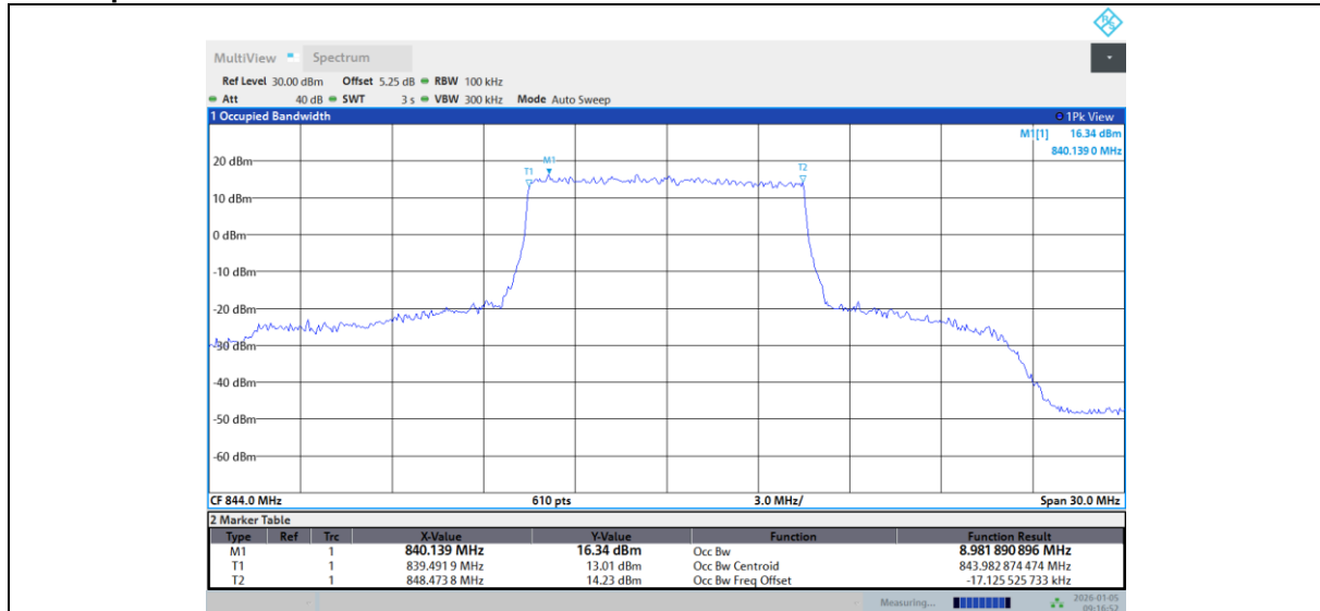
Band 26-10M-HIGH-16QAM-Full RB
