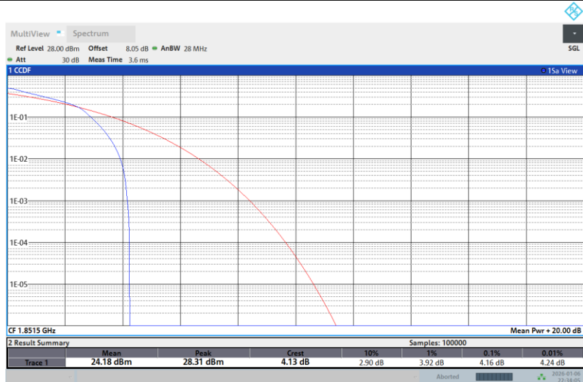
Band 25-3M-LOW-64QAM-1RB Low
