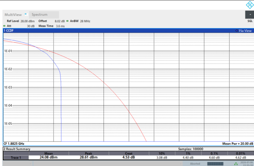
Band 25-3M-MID-64QAM-Full RB
