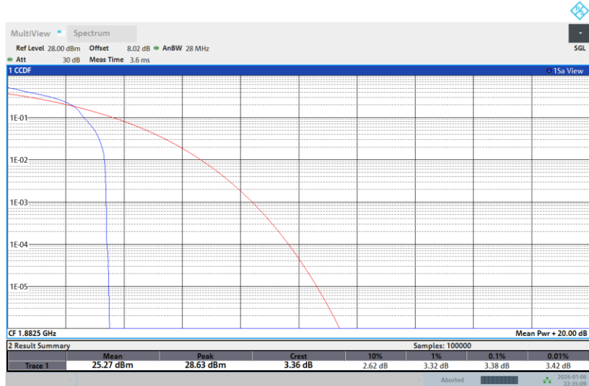
Band 25-3M-MID-16QAM-Full RB
