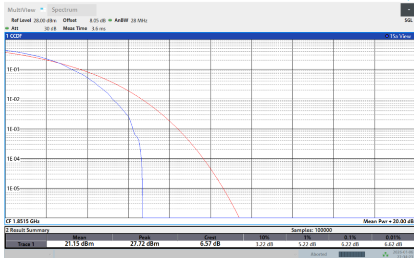
Band 25-3M-LOW-256QAM-Full RB
