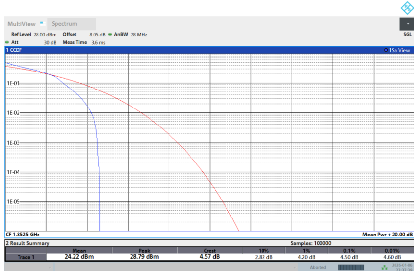
Band 25-5M-LOW-64QAM-1RB Low
