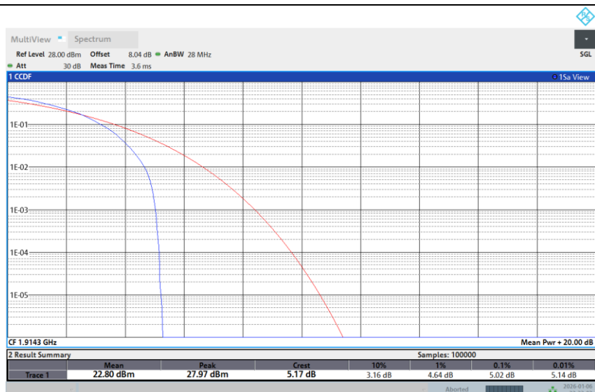
Band 25-1.4M-HIGH-256QAM-1RB Low
