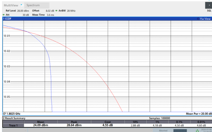
Band 25-5M-MID-64QAM-1RB Low
