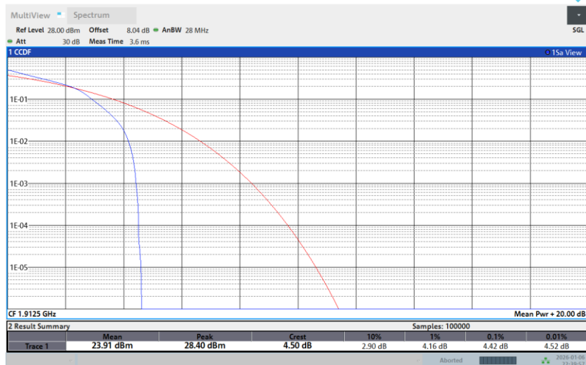
Band 25-5M-HIGH-64QAM-1RB Low
