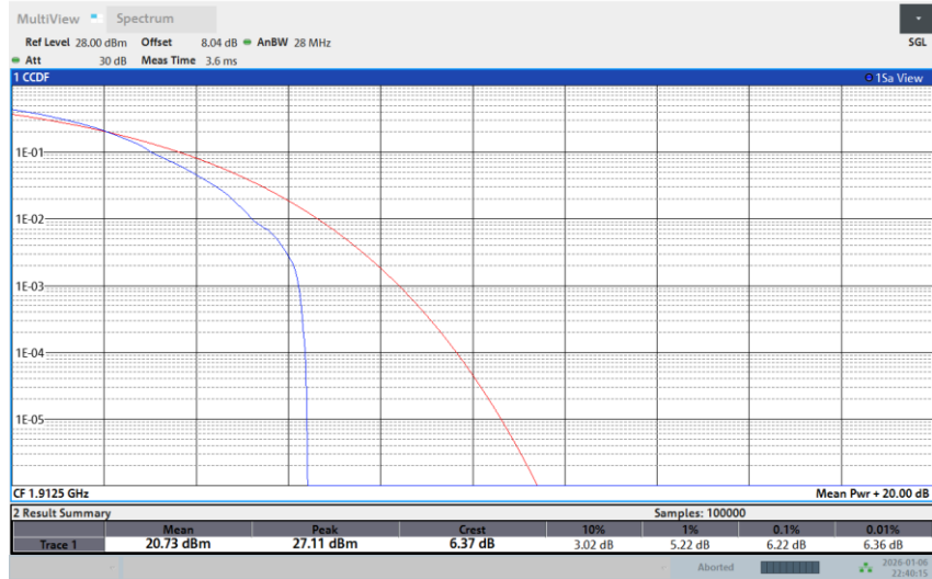
Band 25-5M-HIGH-256QAM-Full RB
