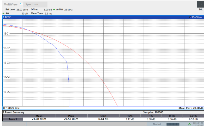
Band 25-5M-LOW-256QAM-Full RB
