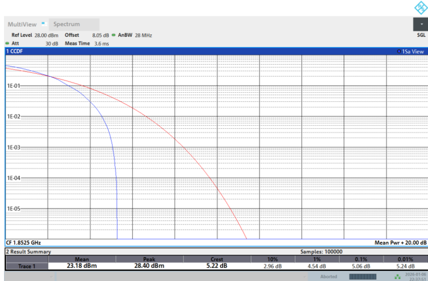
Band 25-5M-LOW-256QAM-1RB Low
