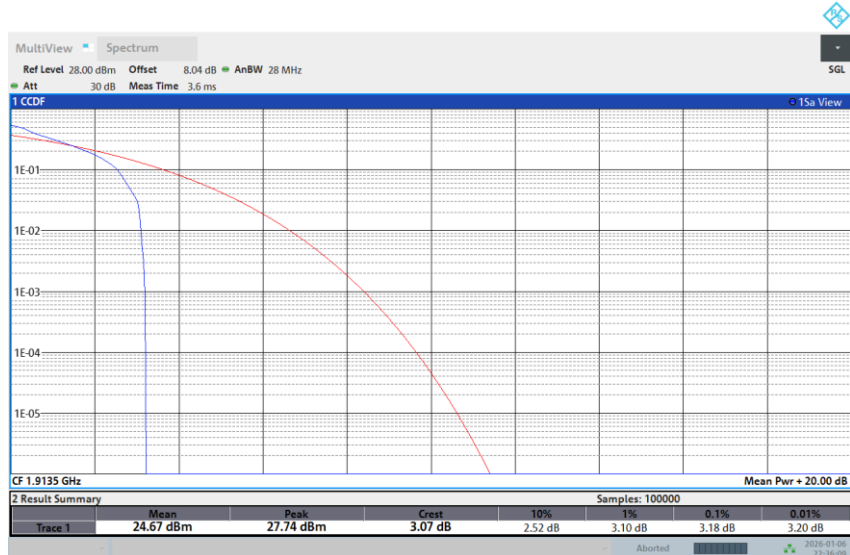
Band 25-3M-HIGH-QPSK-Full RB
