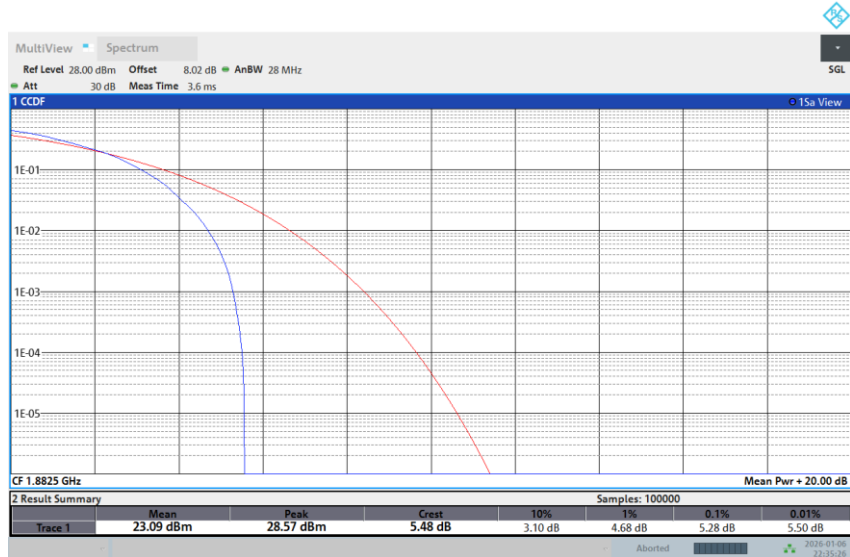
Band 25-3M-MID-256QAM-1RB Low
