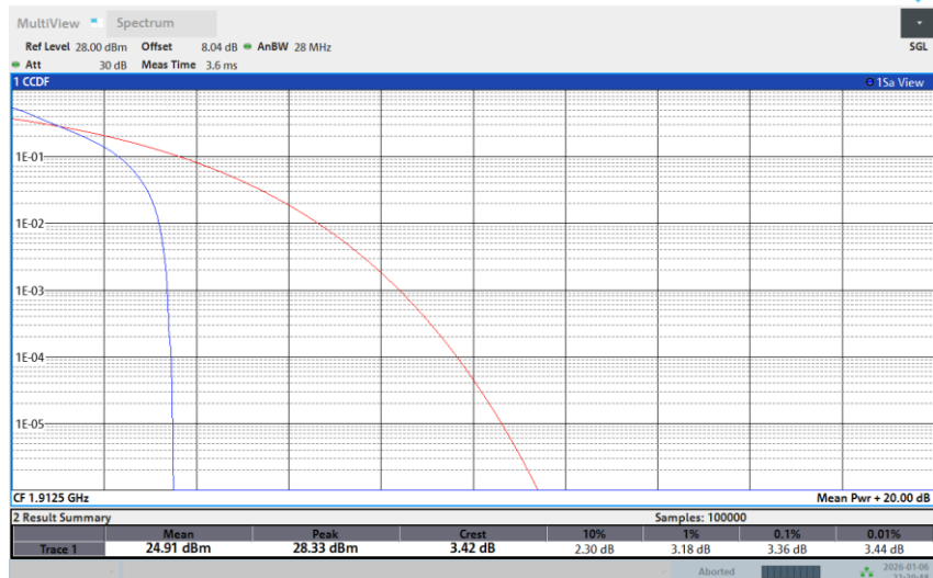
Band 25-5M-HIGH-16QAM-1RB Low
