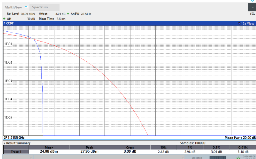
Band 25-3M-HIGH-16QAM-Full RB
