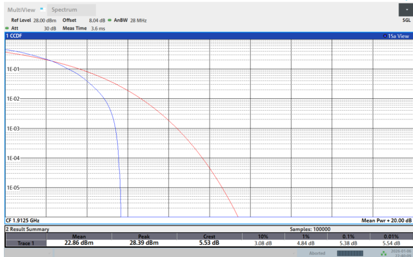
Band 25-5M-HIGH-256QAM-1RB Low
