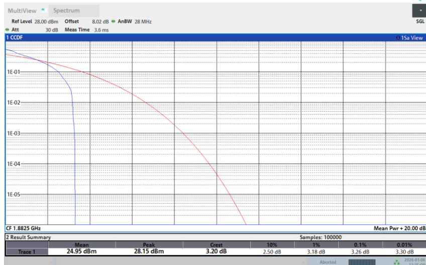
Band 25-3M-MID-QPSK-Full RB
