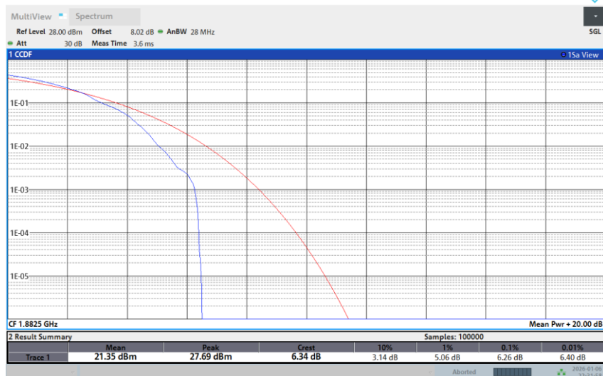
Band 25-1.4M-MID-256QAM-Full RB
