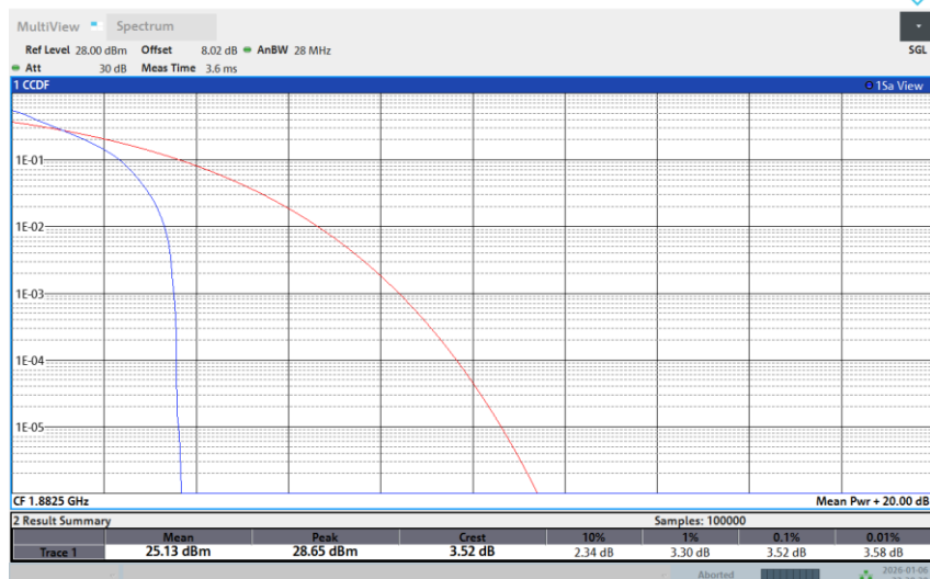
Band 25-5M-MID-16QAM-1RB Low
