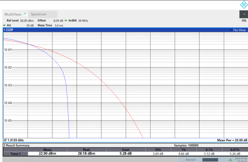
Band 25-3M-HIGH-256QAM-1RB Low
