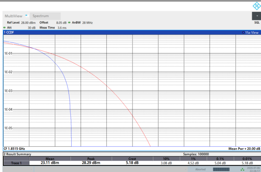
Band 25-3M-LOW-256QAM-1RB Low
