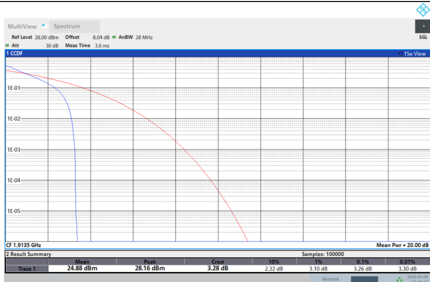
Band 25-3M-HIGH-16QAM-1RB Low
