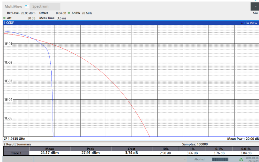
Band 25-3M-HIGH-64QAM-Full RB
