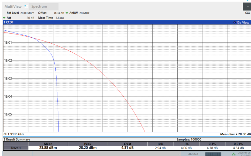
Band 25-3M-HIGH-64QAM-1RB Low
