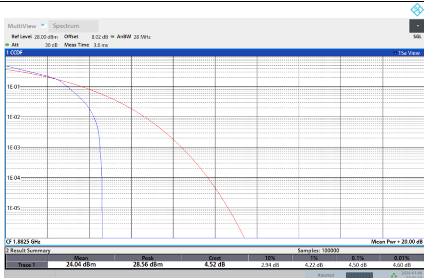
Band 25-3M-MID-64QAM-1RB Low
