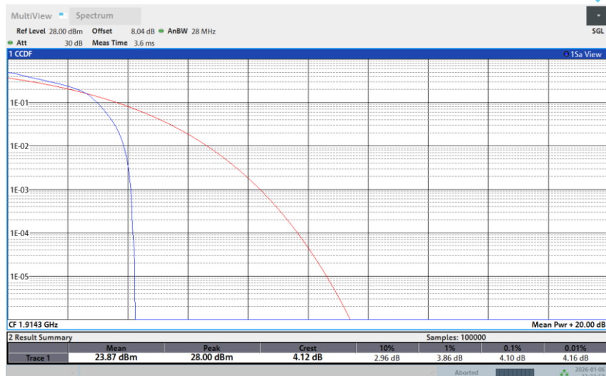
Band 25-1.4M-HIGH-64QAM-1RB Low
