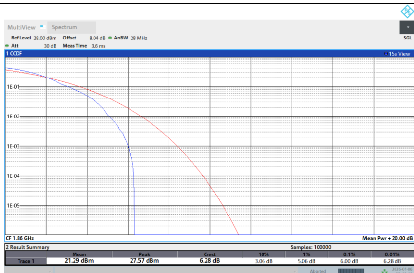
Band 25-20M-LOW-256QAM-Full RB
