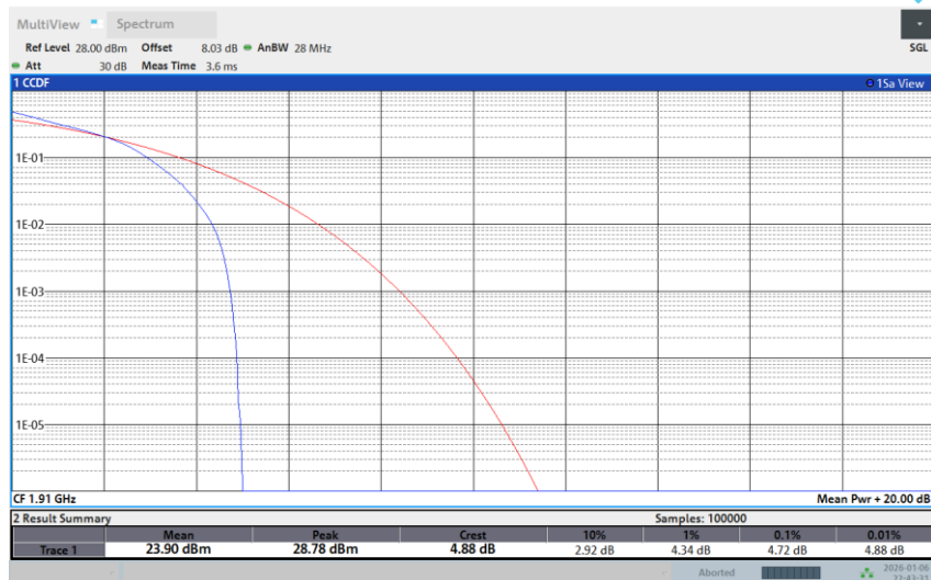
Band 25-10M-HIGH-64QAM-1RB Low
