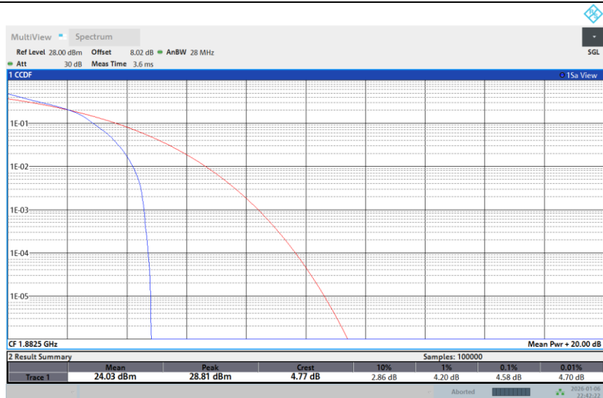
Band 25-10M-MID-64QAM-1RB Low
