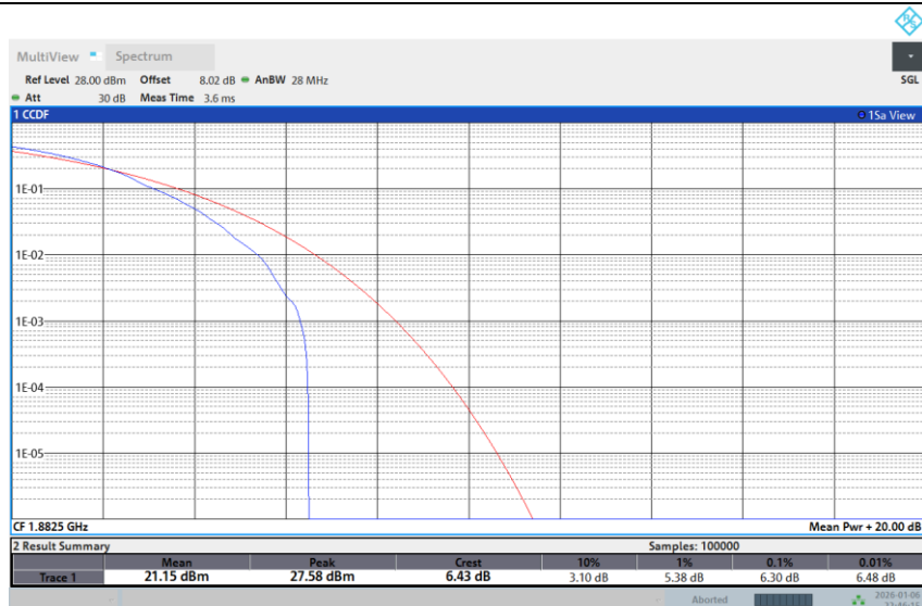
Band 25-15M-MID-256QAM-Full RB
