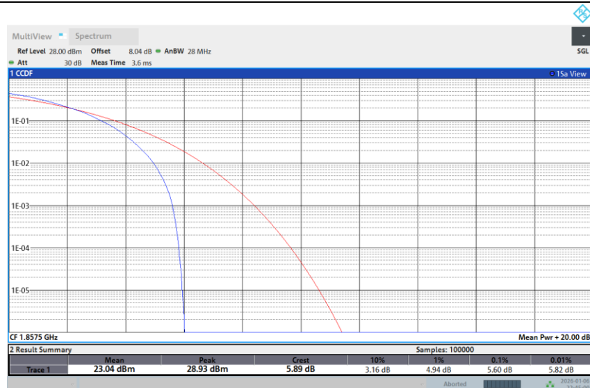
Band 25-15M-LOW-256QAM-1RB Low
