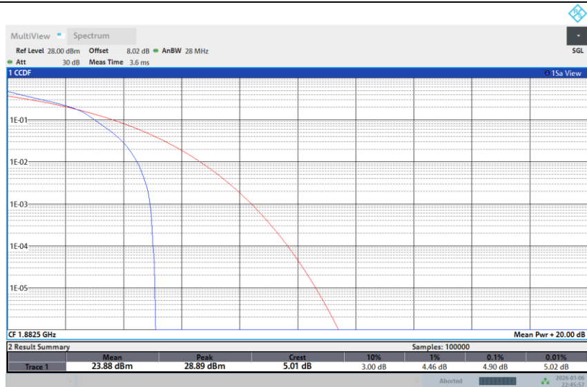
Band 25-15M-MID-64QAM-1RB Low
