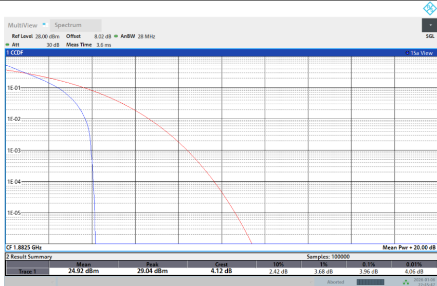
Band 25-15M-MID-16QAM-1RB Low
