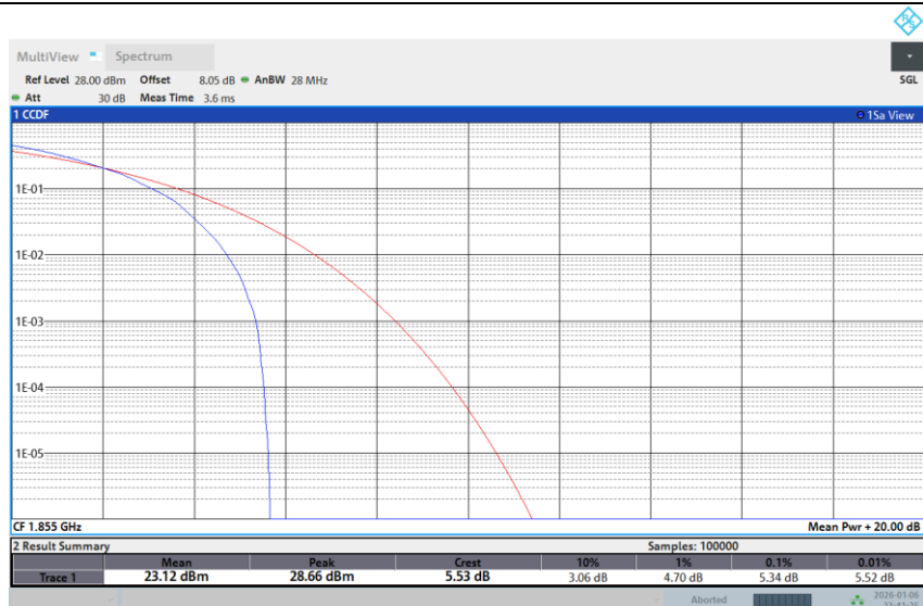
Band 25-10M-LOW-256QAM-1RB Low
