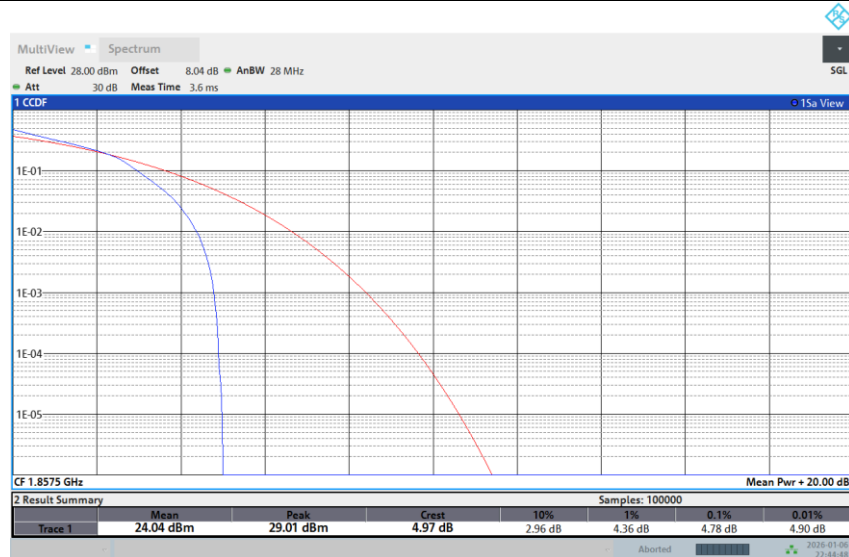
Band 25-15M-LOW-64QAM-1RB Low
