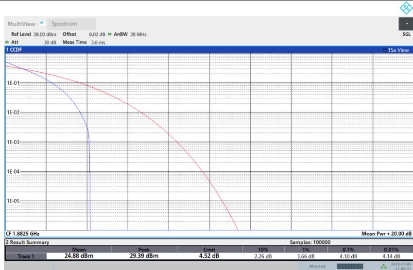
Band 25-20M-MID-16QAM-1RB Low
