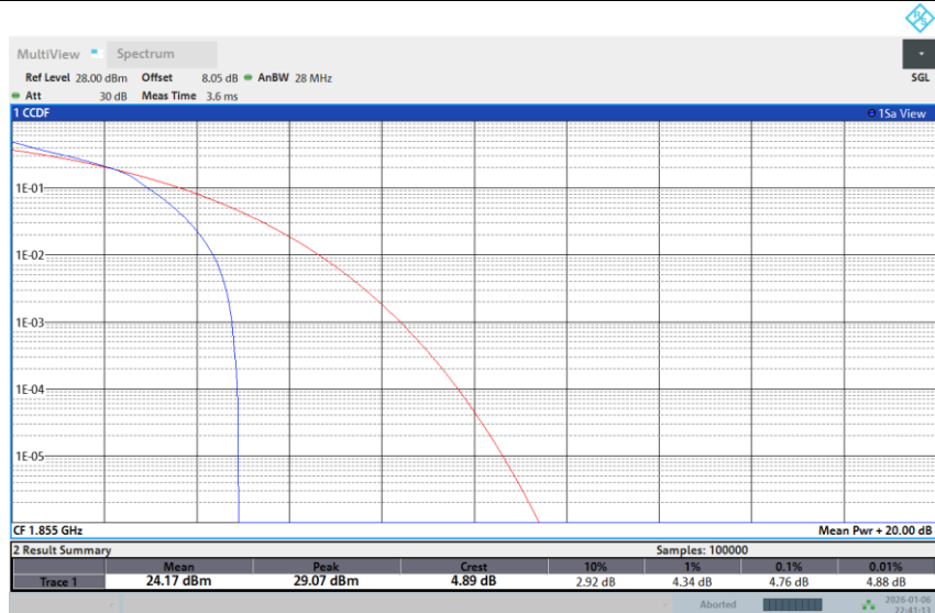
Band 25-10M-LOW-64QAM-1RB Low
