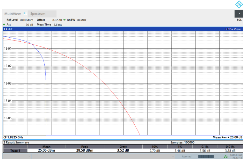
Band 25-10M-MID-16QAM-Full RB
