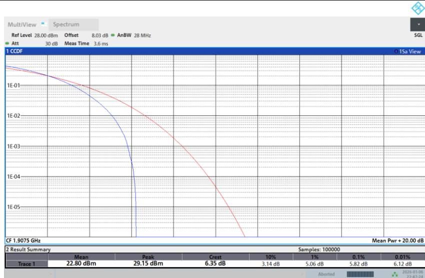
Band 25-15M-HIGH-256QAM-1RB Low
