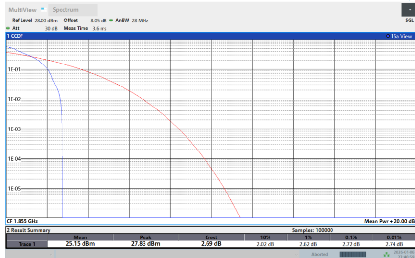
Band 25-10M-LOW-QPSK-Full RB
