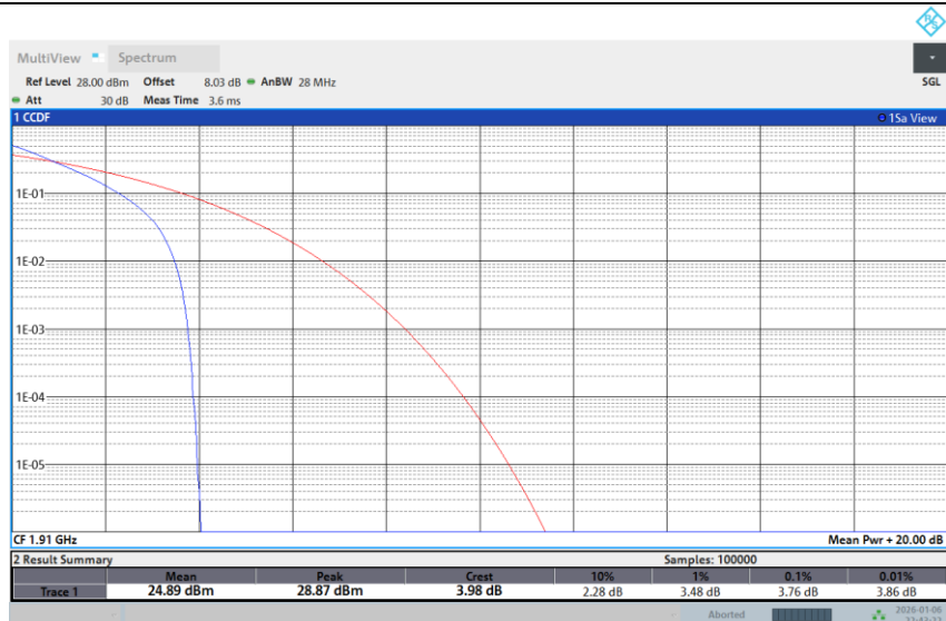
Band 25-10M-HIGH-16QAM-1RB Low
