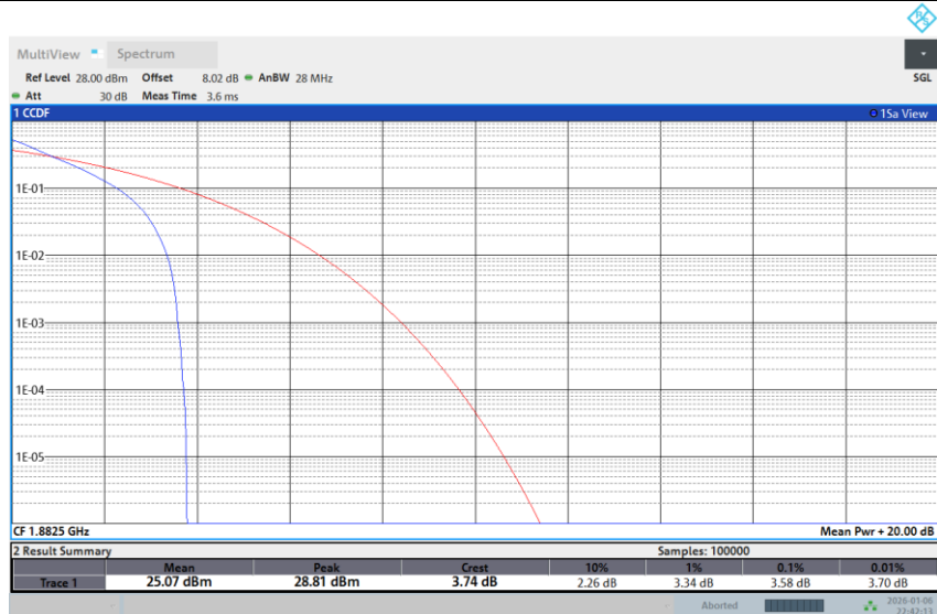
Band 25-10M-MID-16QAM-1RB Low
