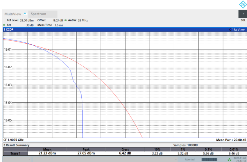
Band 25-15M-HIGH-256QAM-Full RB
