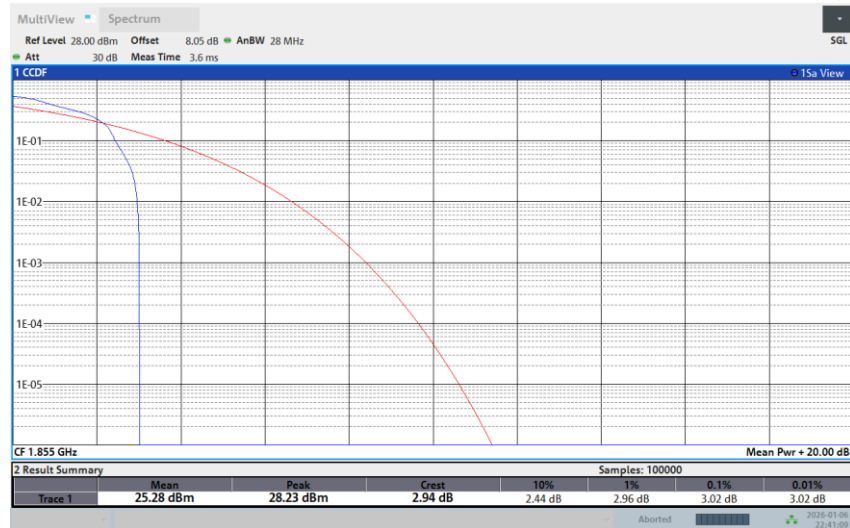
Band 25-10M-LOW-16QAM-Full RB
