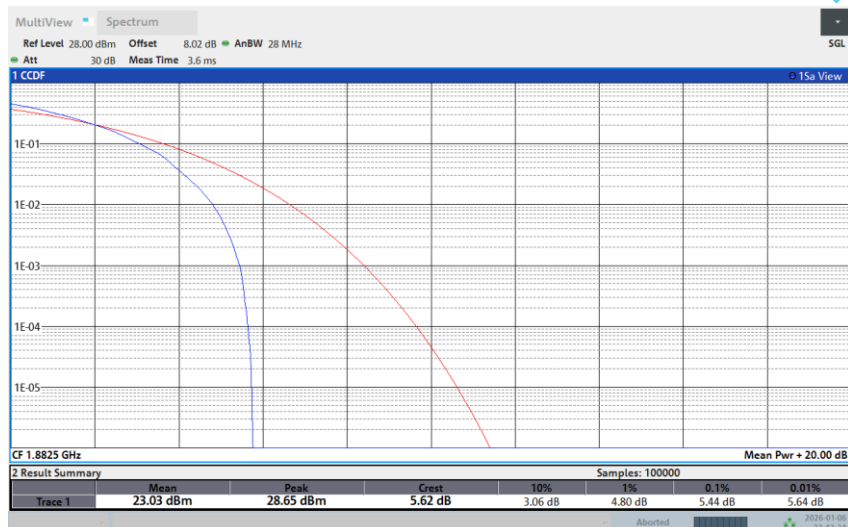
Band 25-10M-MID-256QAM-1RB Low
