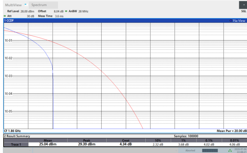
Band 25-20M-LOW-16QAM-1RB Low
