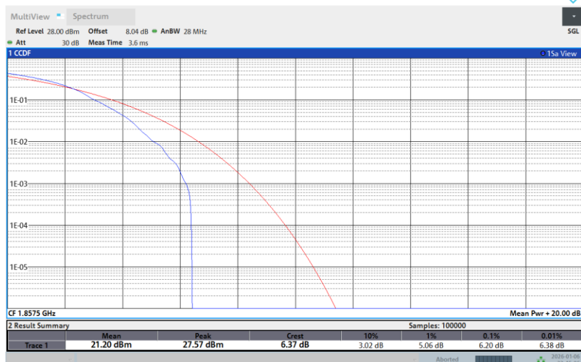
Band 25-15M-LOW-256QAM-Full RB
