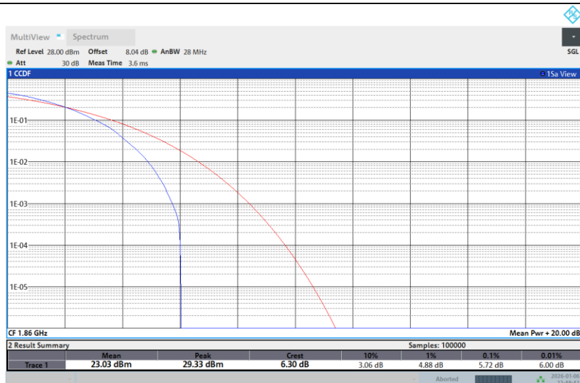
Band 25-20M-LOW-256QAM-1RB Low
