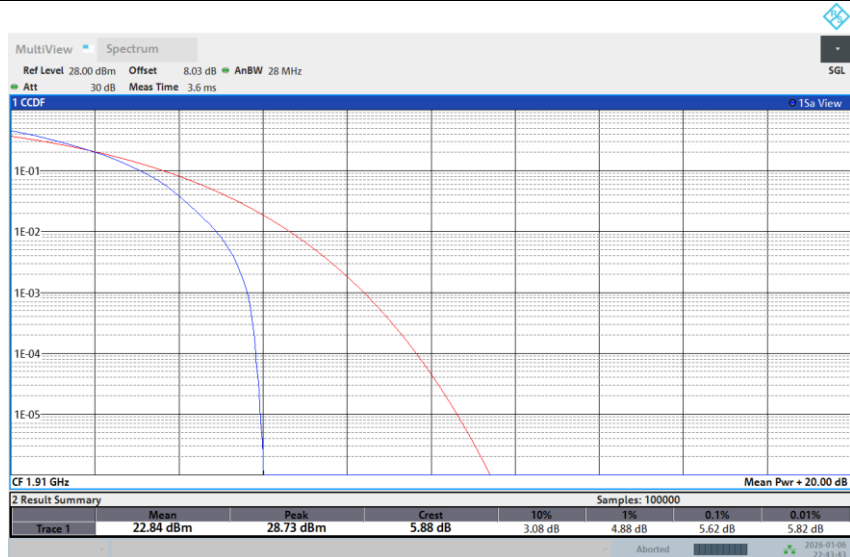
Band 25-10M-HIGH-256QAM-1RB Low
