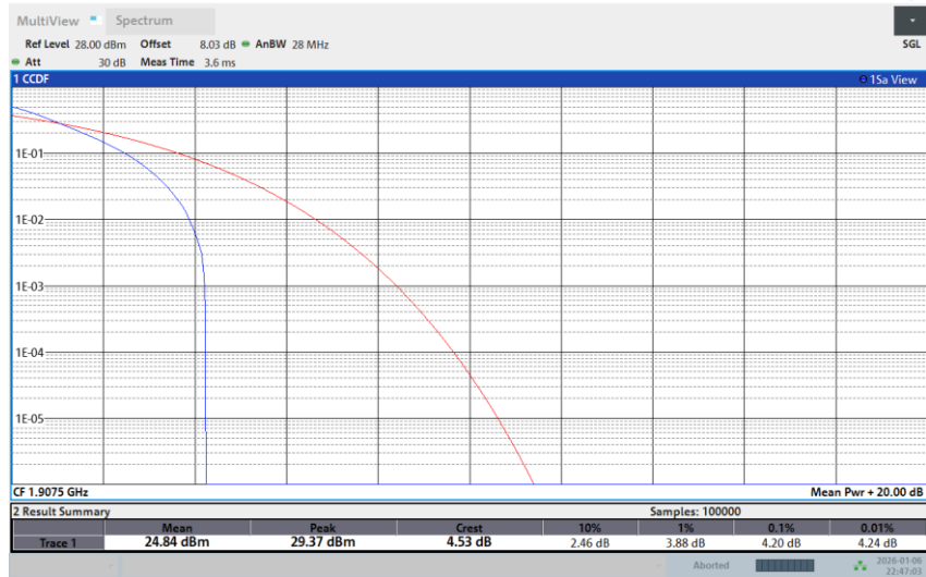
Band 25-15M-HIGH-16QAM-1RB Low
