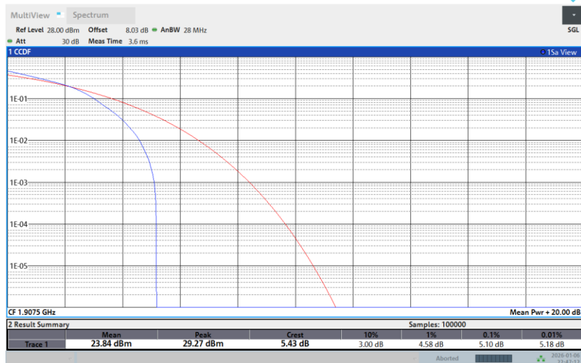
Band 25-15M-HIGH-64QAM-1RB Low
