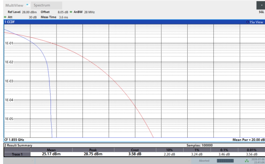
Band 25-10M-LOW-16QAM-1RB Low
