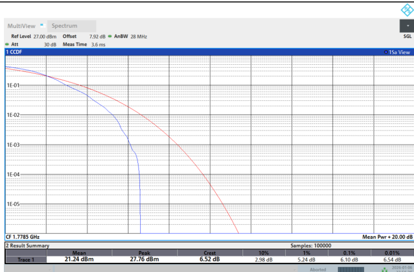
Band 66-3M-HIGH-256QAM-Full RB
