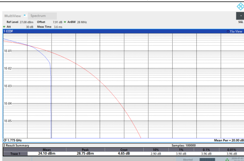
Band 66-10M-HIGH-64QAM-1RB Low
