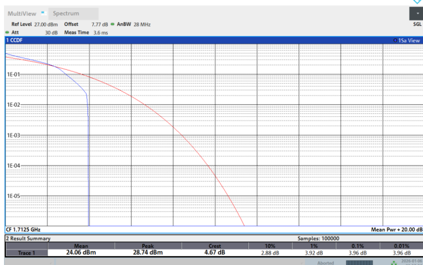
Band 66-5M-LOW-64QAM-1RB Low
