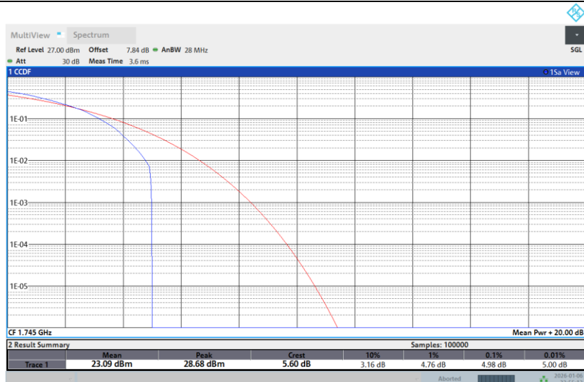
Band 66-3M-MID-256QAM-1RB Low
