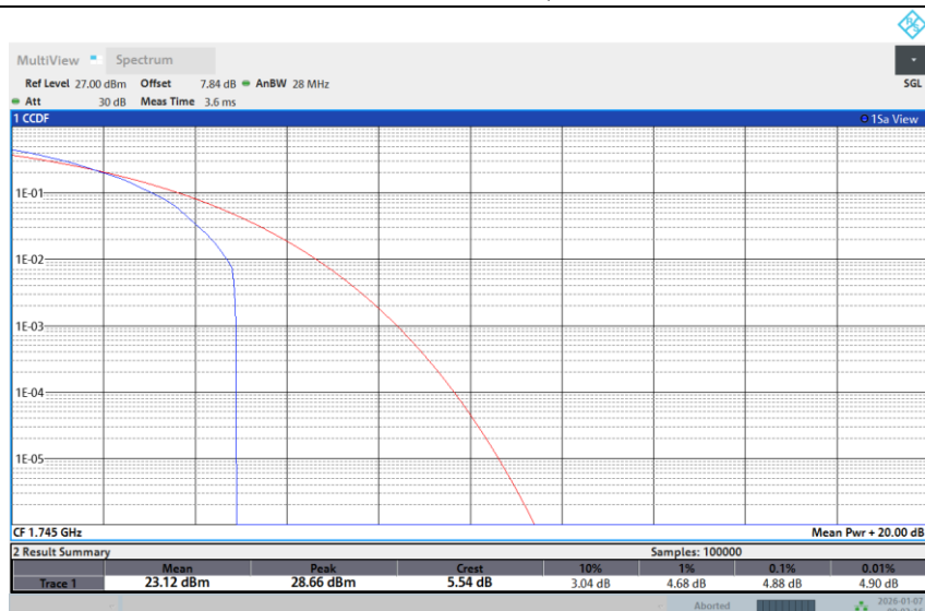
Band 66-10M-MID-256QAM-1RB Low
