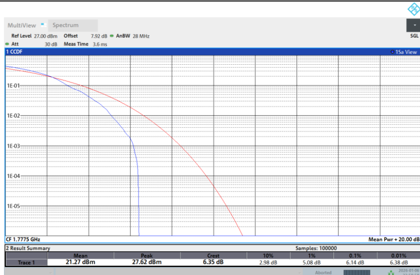
Band 66-5M-HIGH-256QAM-Full RB
