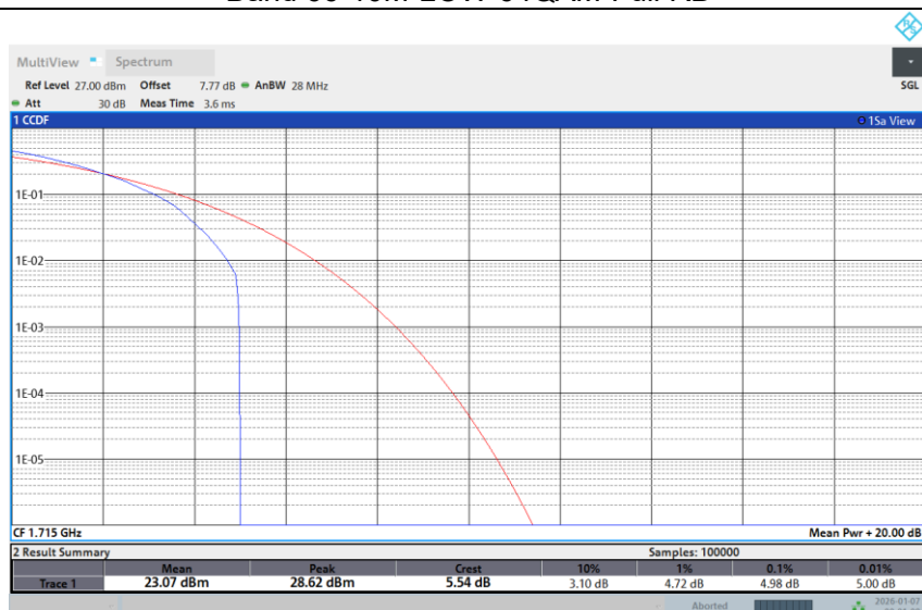
Band 66-10M-LOW-256QAM-1RB Low
