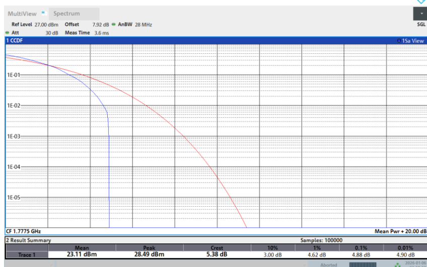
Band 66-5M-HIGH-256QAM-1RB Low
