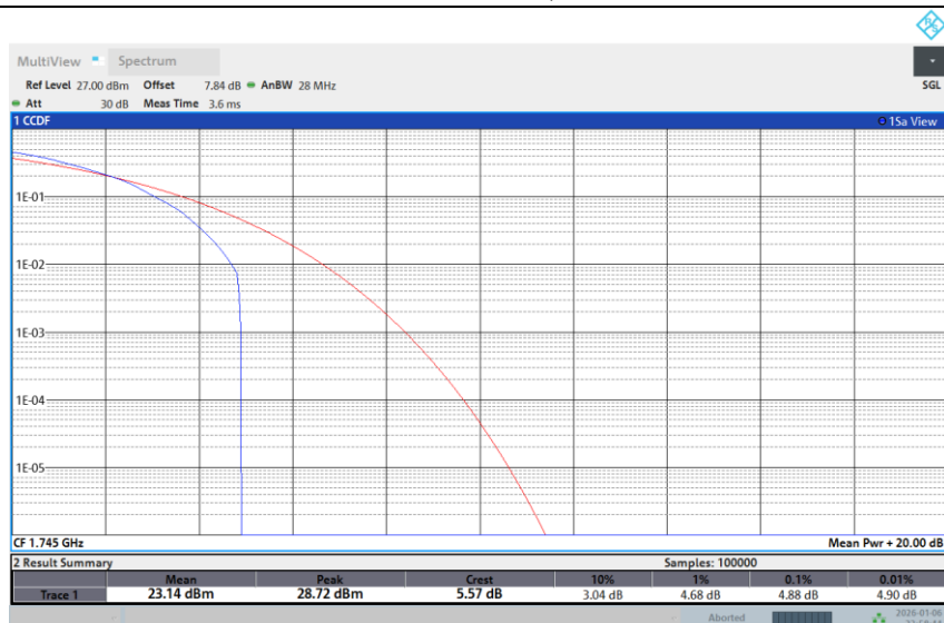
Band 66-5M-MID-256QAM-1RB Low
