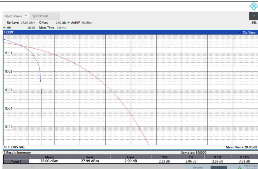
Band 66-3M-HIGH-QPSK-Full RB
