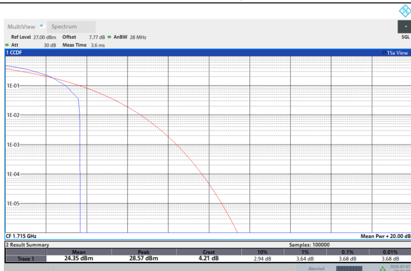
Band 66-10M-LOW-64QAM-Full RB
