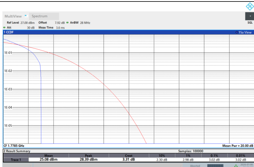
Band 66-3M-HIGH-16QAM-1RB Low
