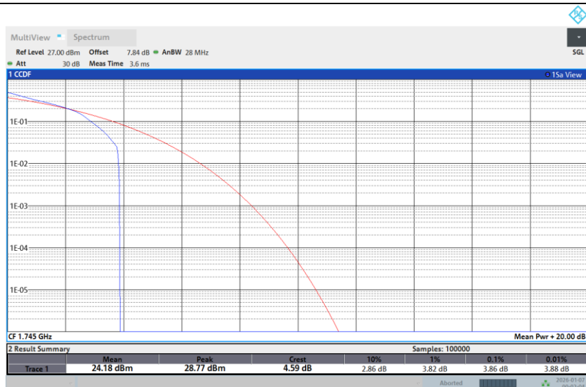
Band 66-10M-MID-64QAM-1RB Low
