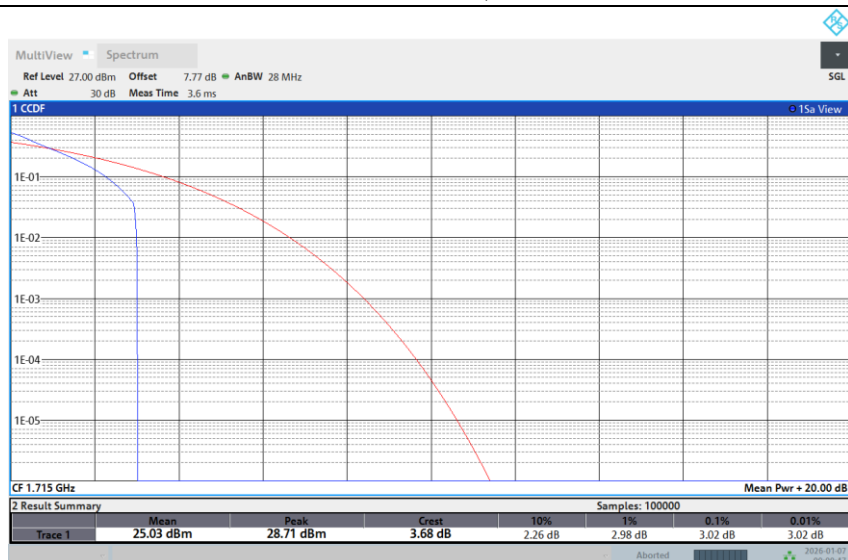
Band 66-10M-LOW-16QAM-1RB Low
