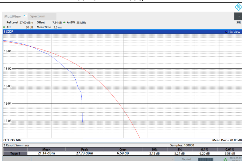
Band 66-10M-MID-256QAM-Full RB
