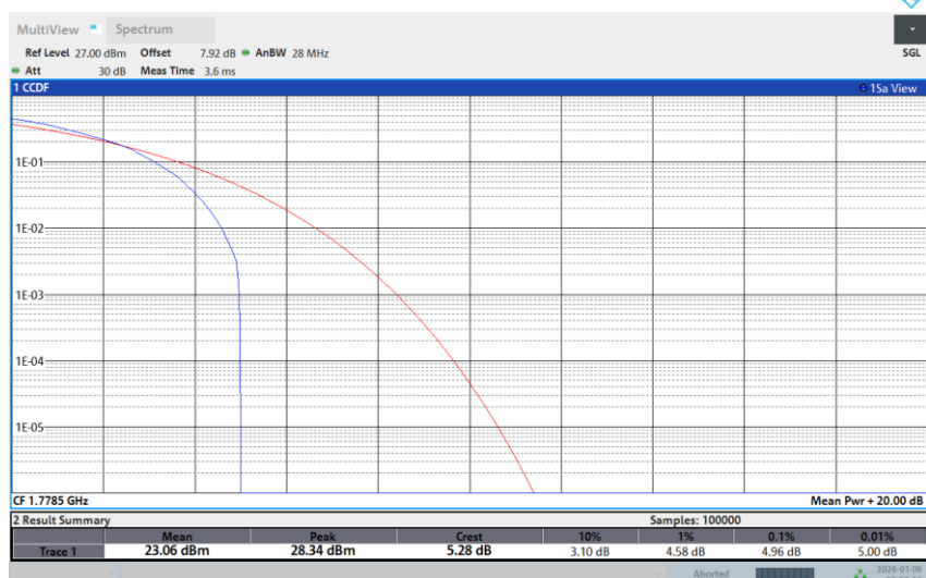
Band 66-3M-HIGH-256QAM-1RB Low
