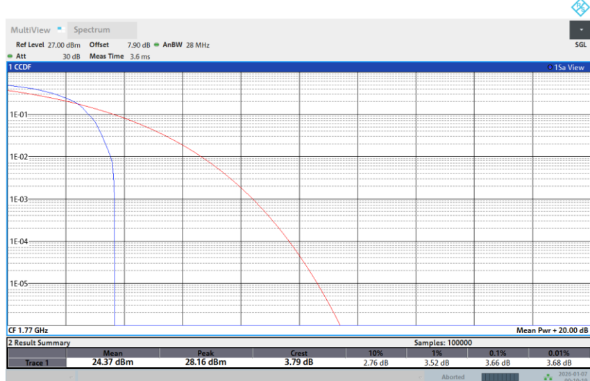
Band 66-20M-HIGH-64QAM-Full RB
