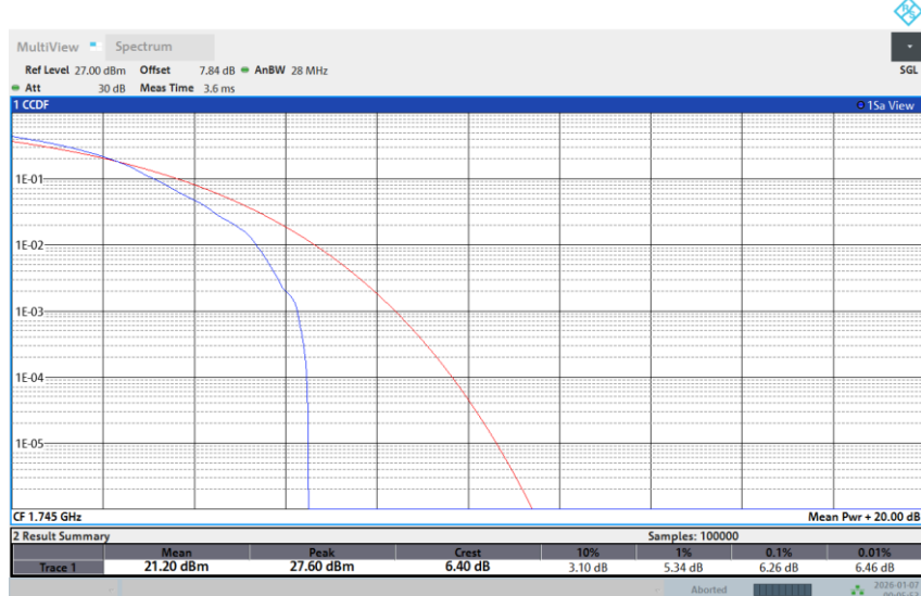
Band 66-15M-MID-256QAM-Full RB
