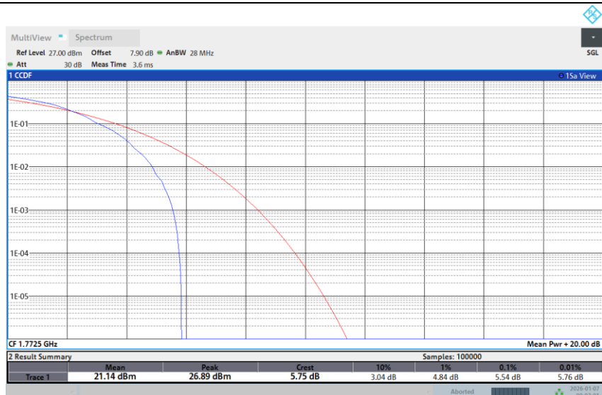
Band 66-15M-HIGH-256QAM-Full RB
