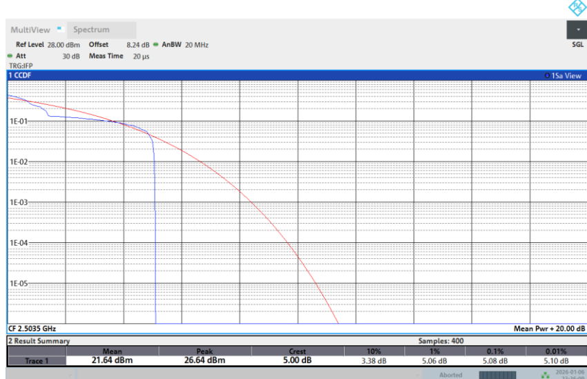
Band 41-15M-LOW-64QAM-Full RB
