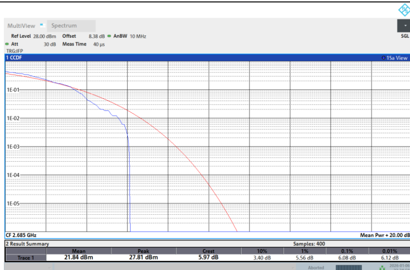
Band 41-10M-HIGH-256QAM-1RB Low
