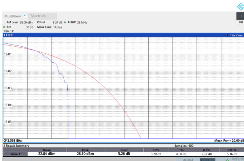
Band 41-20M-MID-64QAM-1RB Low
