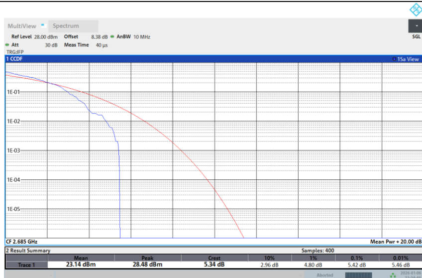
Band 41-10M-HIGH-64QAM-1RB Low
