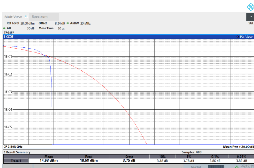
Band 41-15M-MID-256QAM-Full RB
