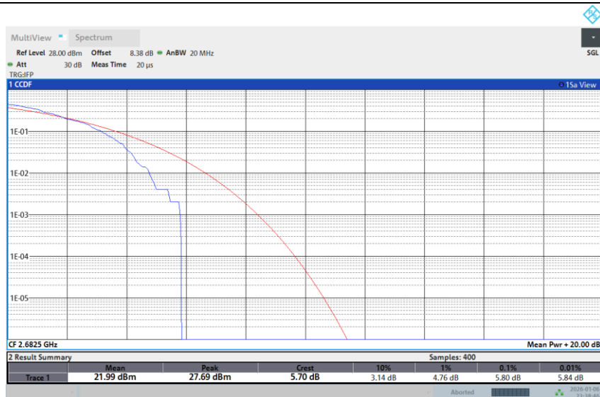
Band 41-15M-HIGH-256QAM-1RB Low
