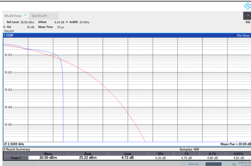
Band 41-15M-LOW-256QAM-Full RB
