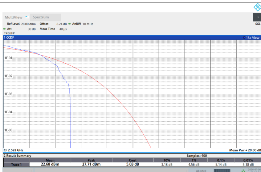
Band 41-10M-MID-64QAM-1RB Low
