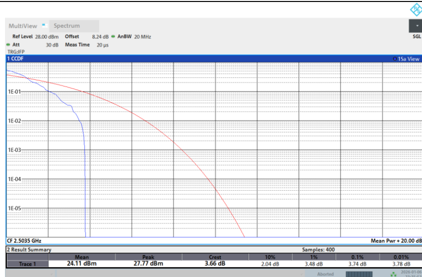
Band 41-15M-LOW-16QAM-1RB Low
