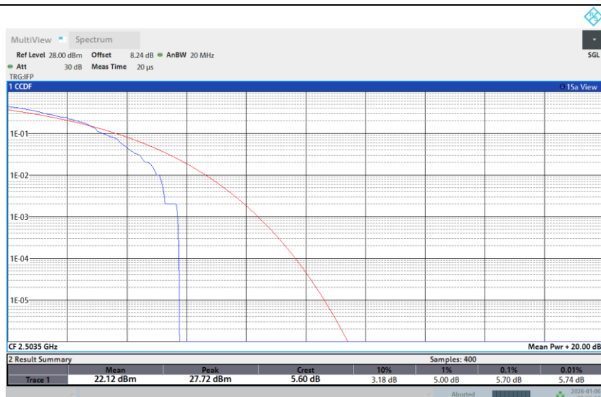
Band 41-15M-LOW-256QAM-1RB Low
