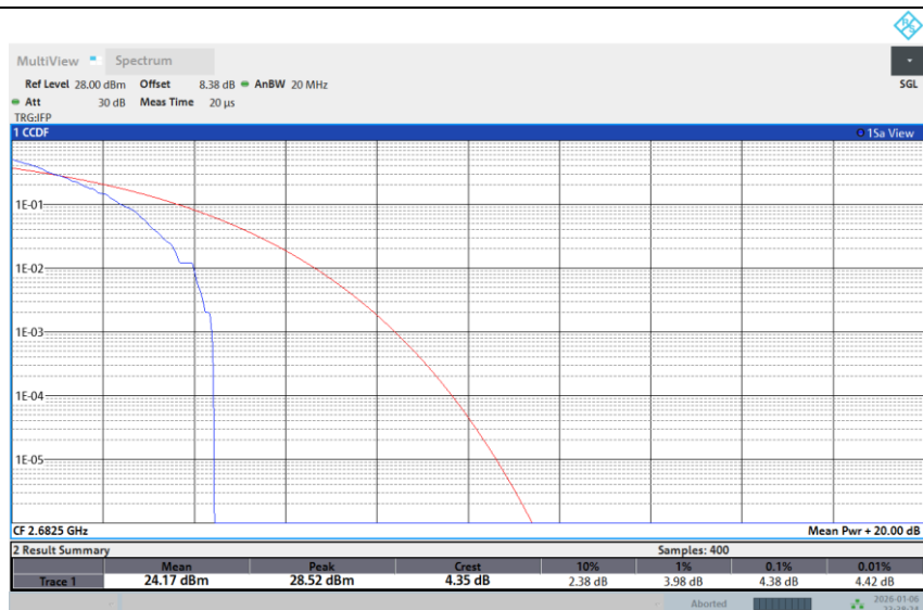
Band 41-15M-HIGH-16QAM-1RB Low
