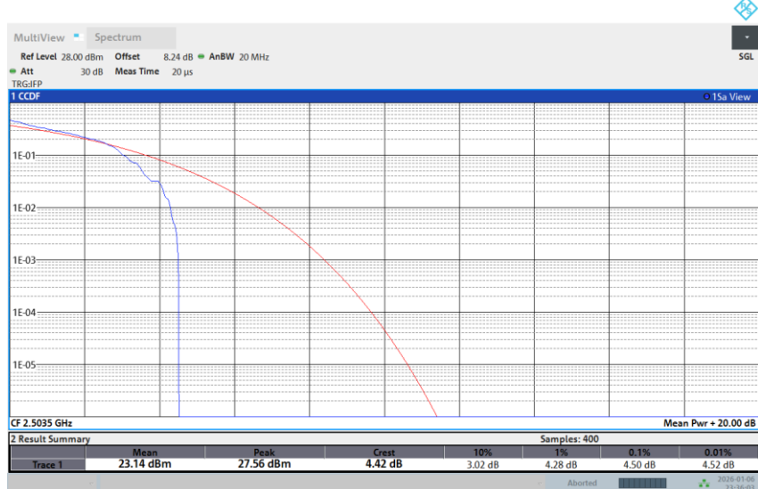
Band 41-15M-LOW-64QAM-1RB Low
