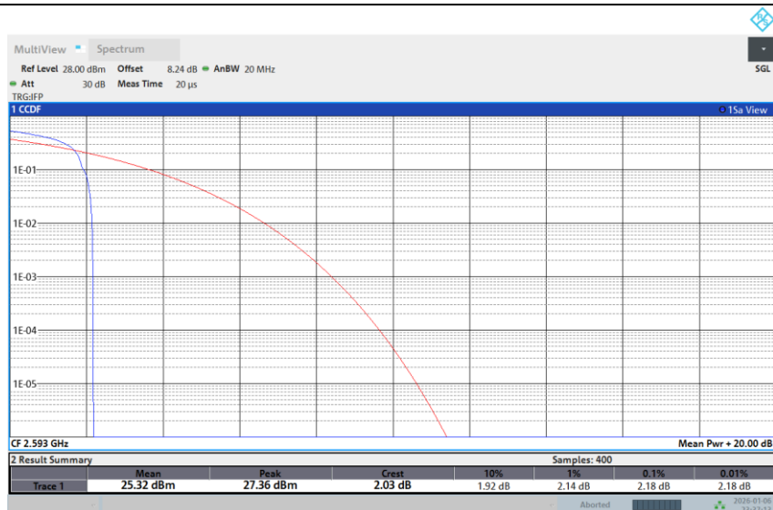
Band 41-15M-MID-16QAM-Full RB
