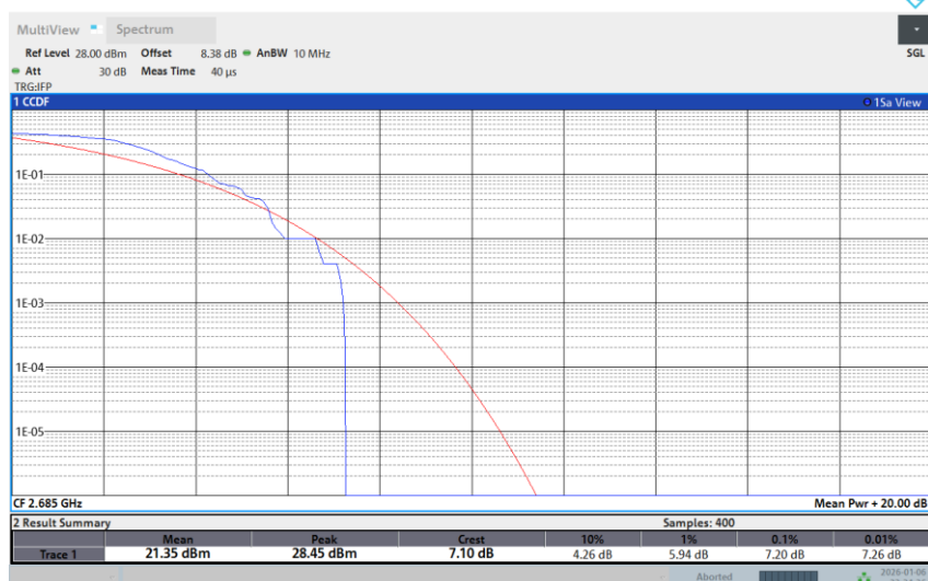
Band 41-10M-HIGH-16QAM-1RB Low
