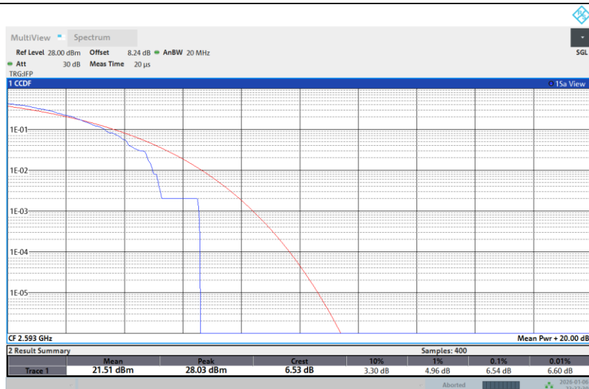
Band 41-15M-MID-256QAM-1RB Low
