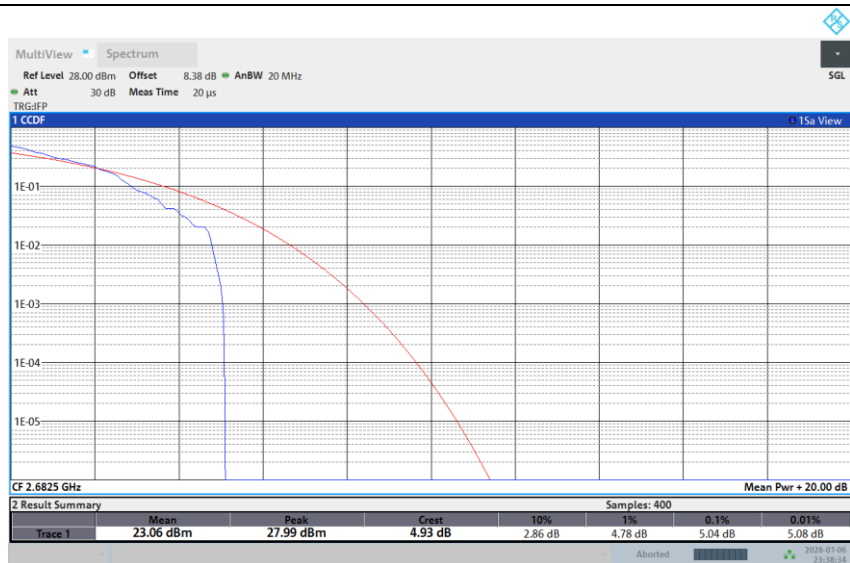
Band 41-15M-HIGH-64QAM-1RB Low
