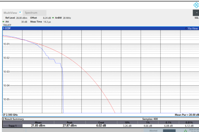
Band 41-20M-MID-256QAM-1RB Low
