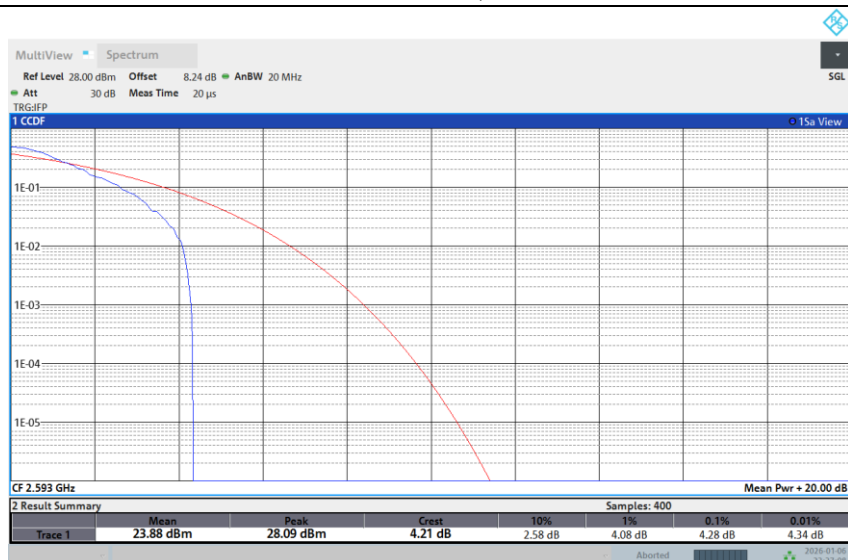
Band 41-15M-MID-16QAM-1RB Low
