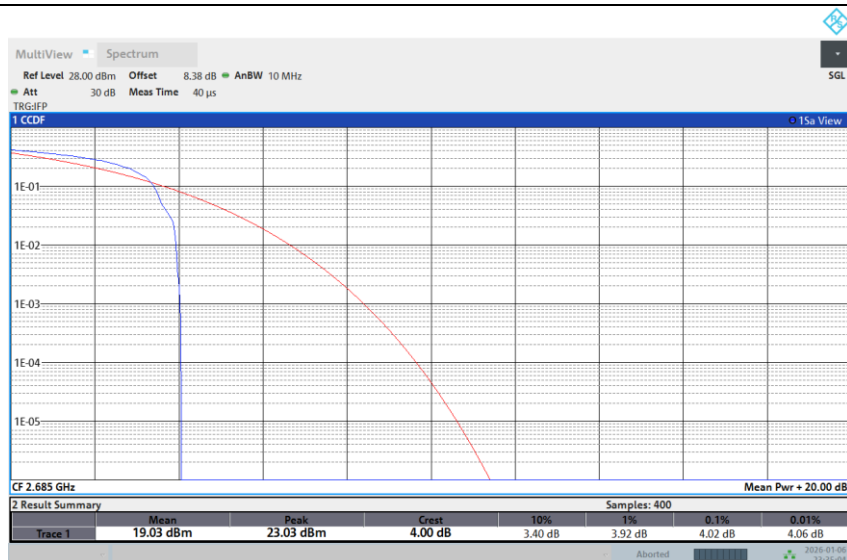
Band 41-10M-HIGH-256QAM-Full RB
