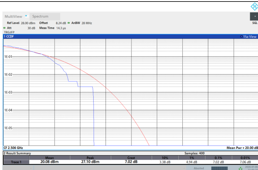
Band 41-20M-MID-QPSK-1RB Low
