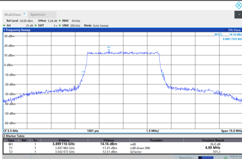
Band 42-5M-MID-16QAM-Full RB
