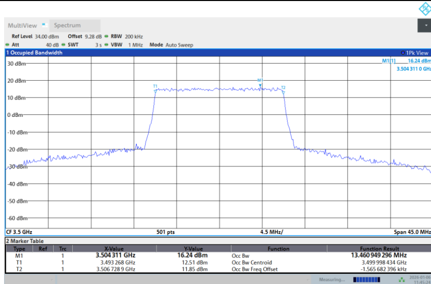
Band 42-15M-MID-16QAM-Full RB
