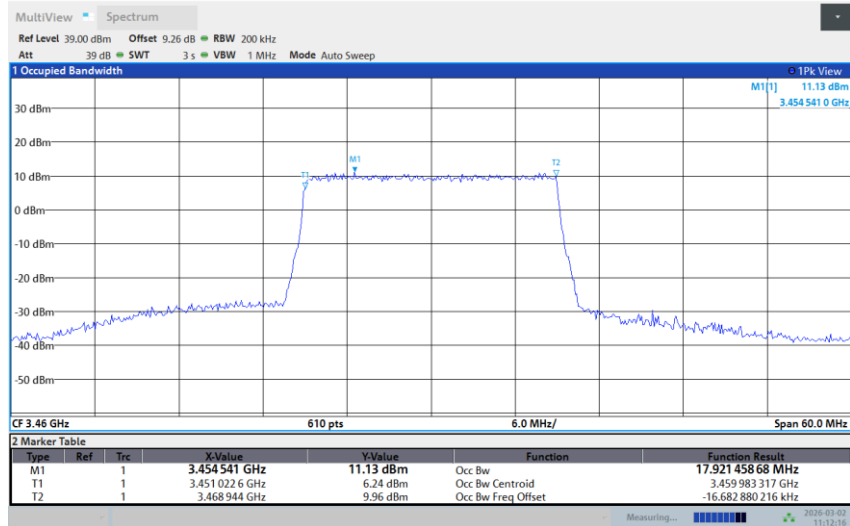
Band 42-20M-MID-QPSK-Full RB
