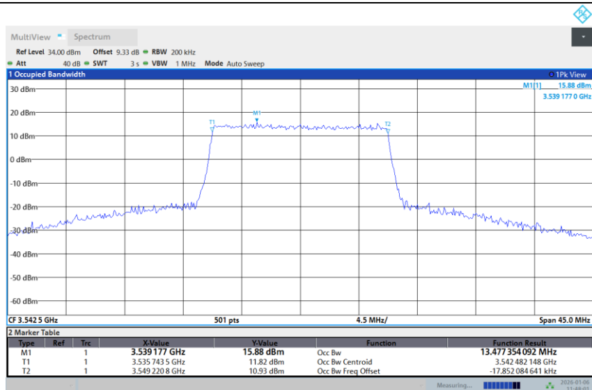
Band 42-15M-HIGH-64QAM-Full RB
