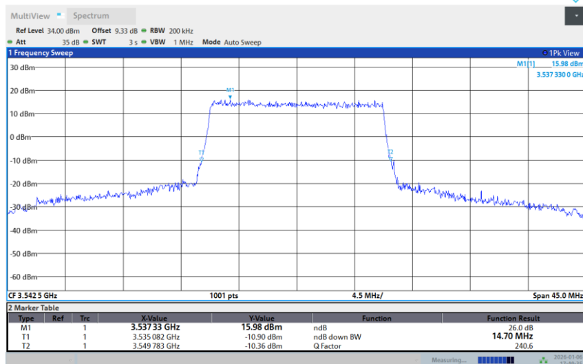
Band 42-15M-HIGH-16QAM-Full RB
