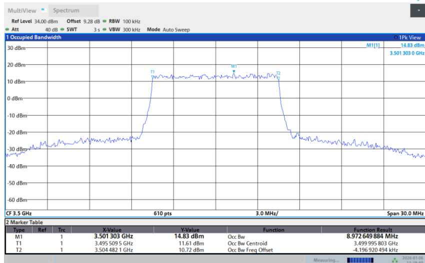
Band 42-10M-MID-16QAM-Full RB
