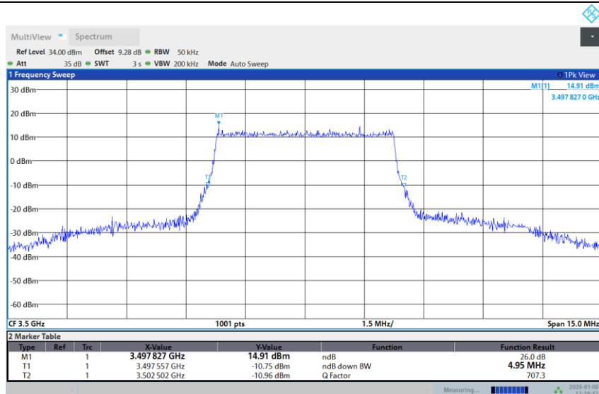
Band 42-5M-MID-64QAM-Full RB
