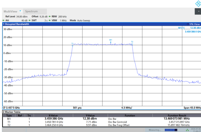
Band 42-15M-MID-QPSK-Full RB
