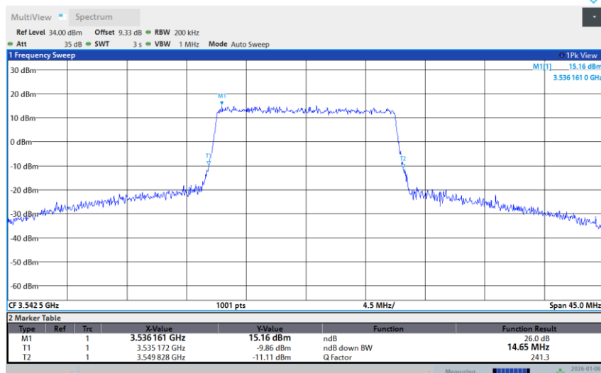
Band 42-15M-HIGH-64QAM-Full RB
