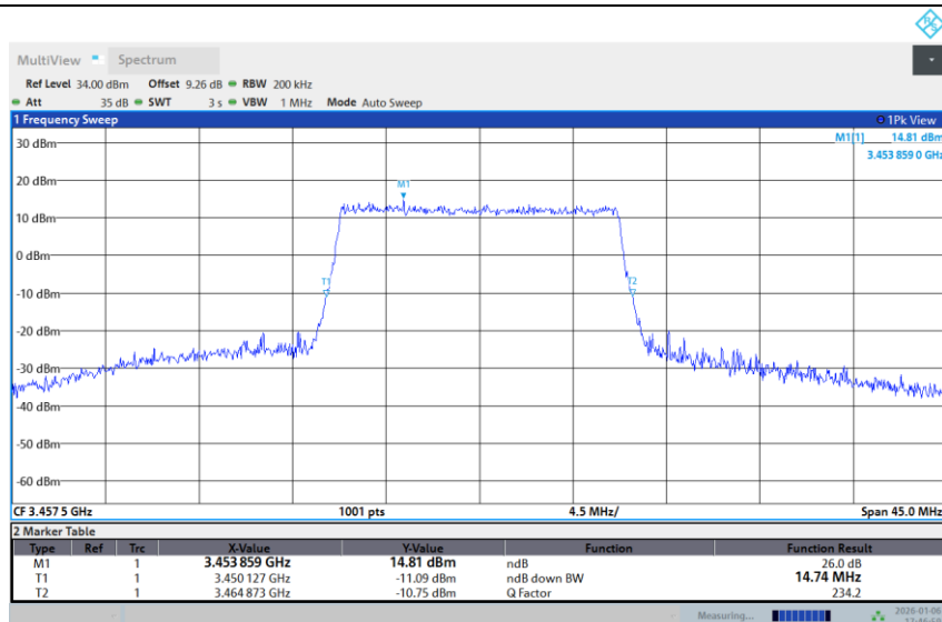
Band 42-15M-LOW-256QAM-Full RB
