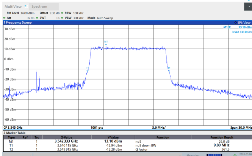
Band 42-10M-HIGH-256QAM-Full RB
