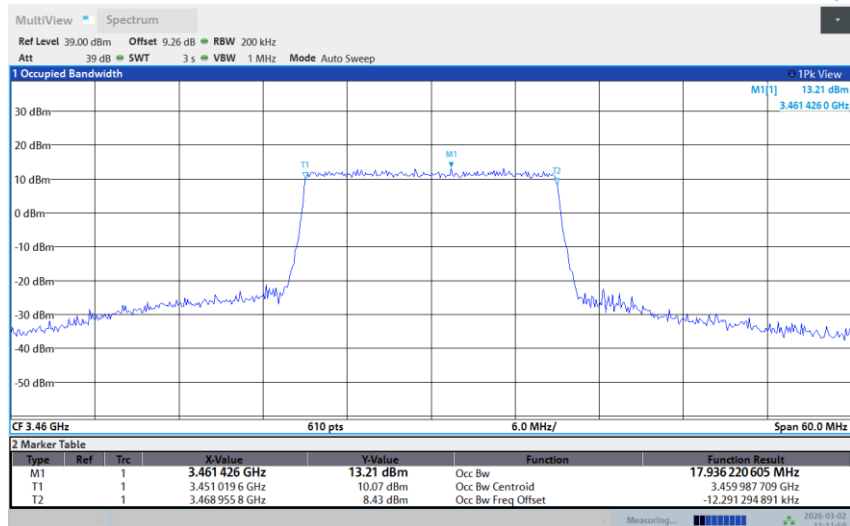
Band 42-20M-LOW-256QAM-Full RB
