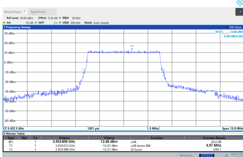
Band 42-5M-LOW-256QAM-Full RB
