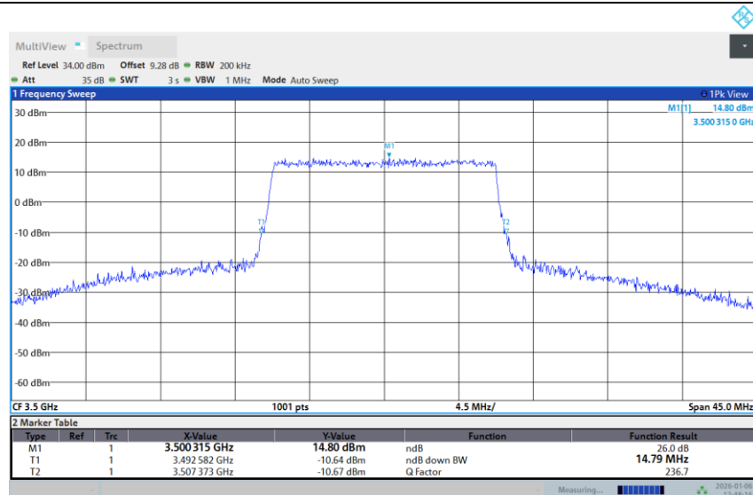
Band 42-15M-MID-64QAM-Full RB
