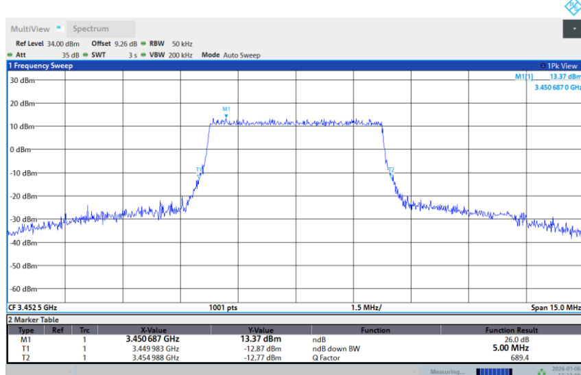
Band 42-5M-LOW-64QAM-Full RB
