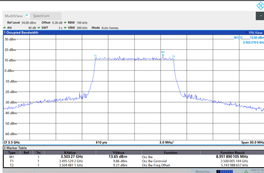
Band 42-10M-MID-256QAM-Full RB
