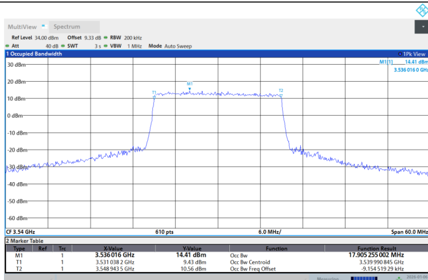
Band 42-20M-HIGH-64QAM-Full RB
