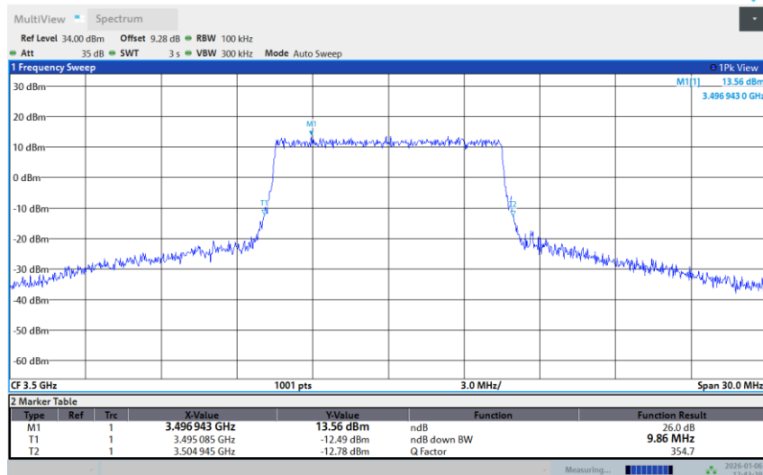
Band 42-10M-MID-64QAM-Full RB
