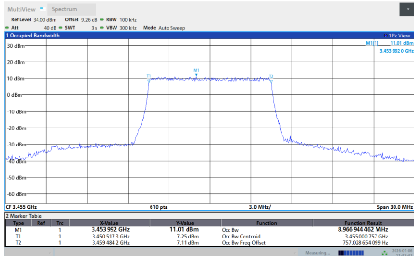
Band 42-10M-MID-QPSK-Full RB
