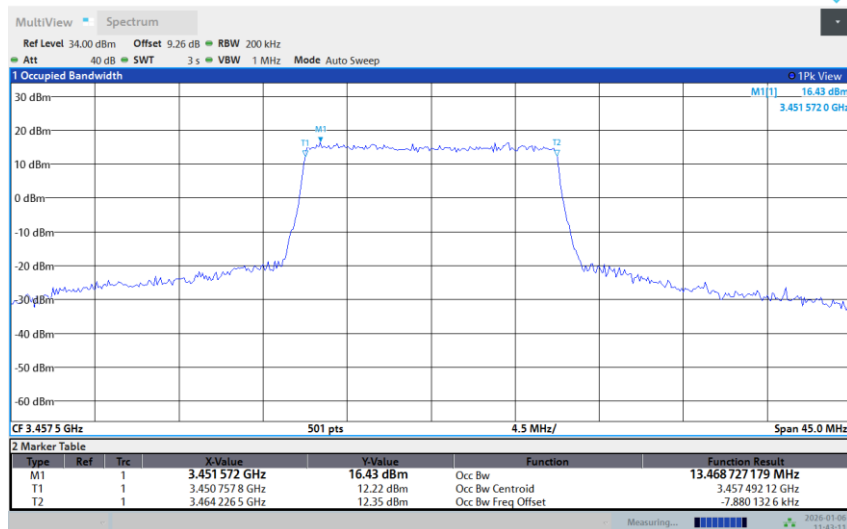
Band 42-15M-LOW-16QAM-Full RB
