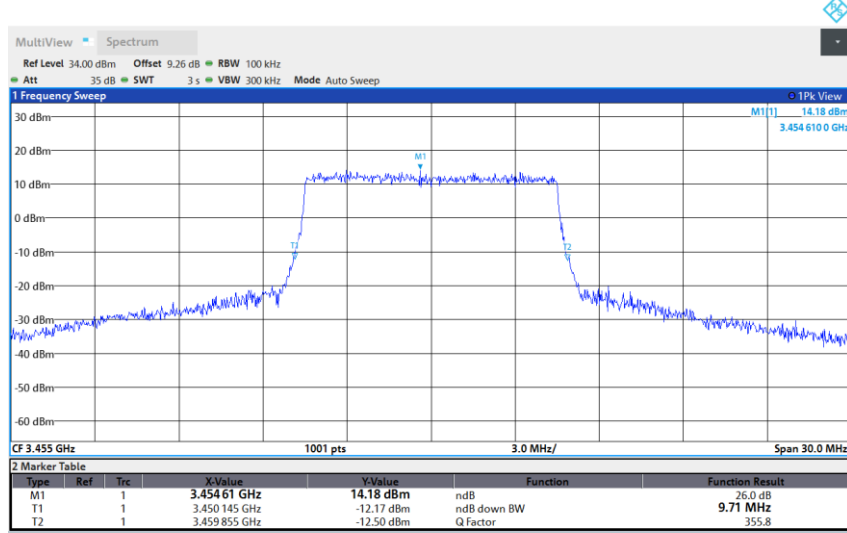
Band 42-10M-LOW-64QAM-Full RB
