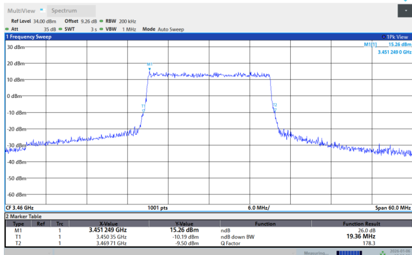
Band 42-20M-LOW-16QAM-Full RB
