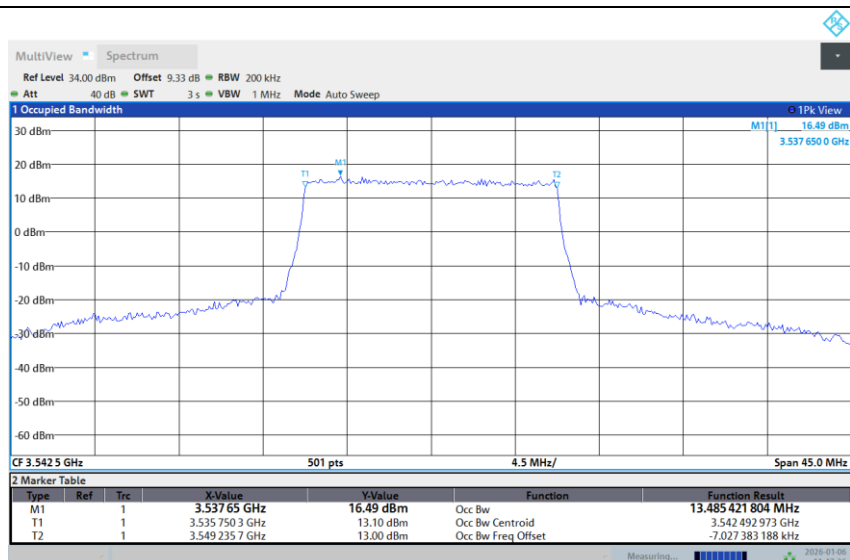
Band 42-15M-HIGH-16QAM-Full RB
