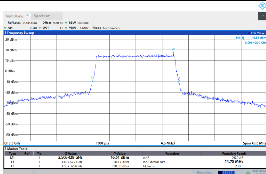
Band 42-15M-MID-16QAM-Full RB
