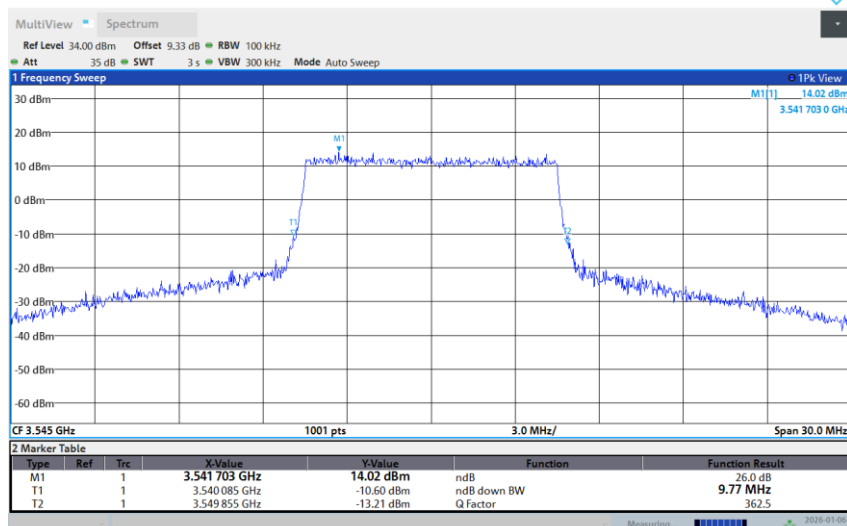
Band 42-10M-HIGH-64QAM-Full RB
