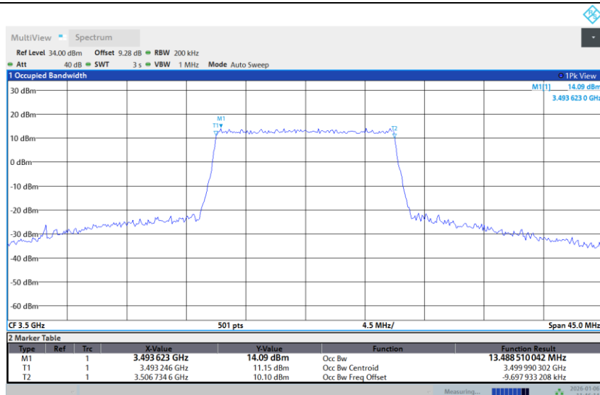
Band 42-15M-MID-256QAM-Full RB
