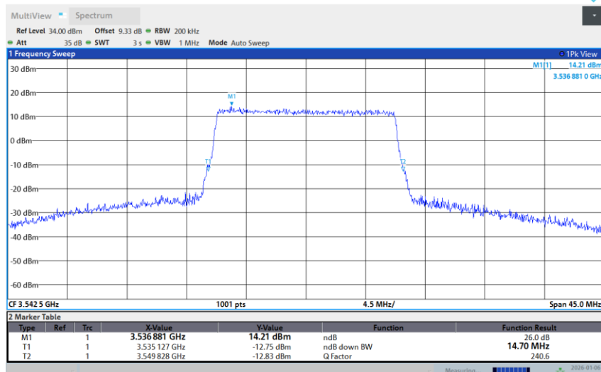
Band 42-15M-HIGH-256QAM-Full RB
