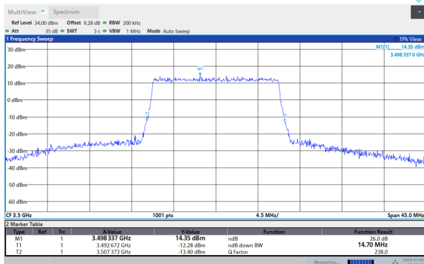
Band 42-15M-MID-256QAM-Full RB
