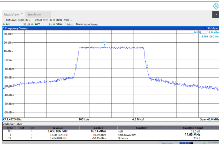
Band 42-15M-LOW-16QAM-Full RB
