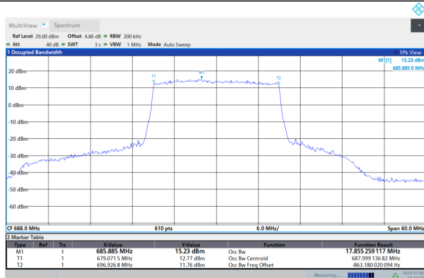
Band 71-20M-HIGH-16QAM-Full RB
