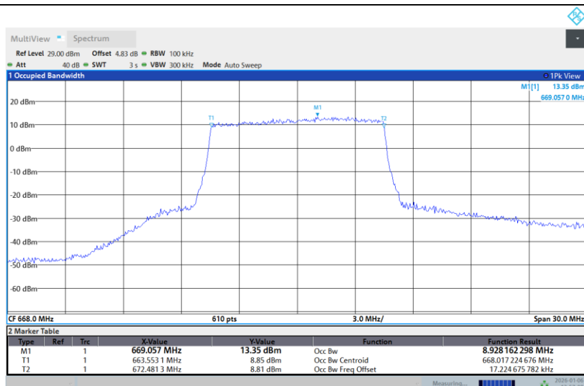
Band 71-10M-LOW-256QAM-Full RB
