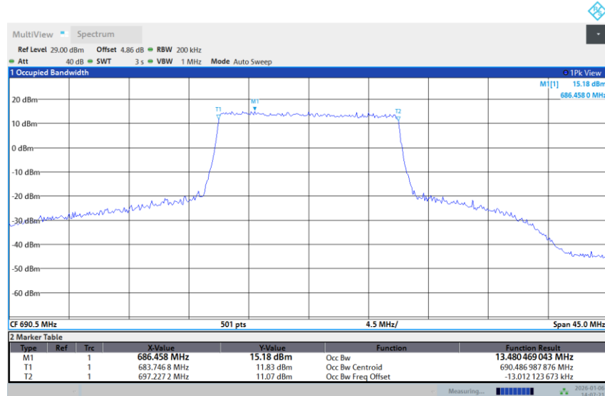
Band 71-15M-HIGH-64QAM-Full RB
