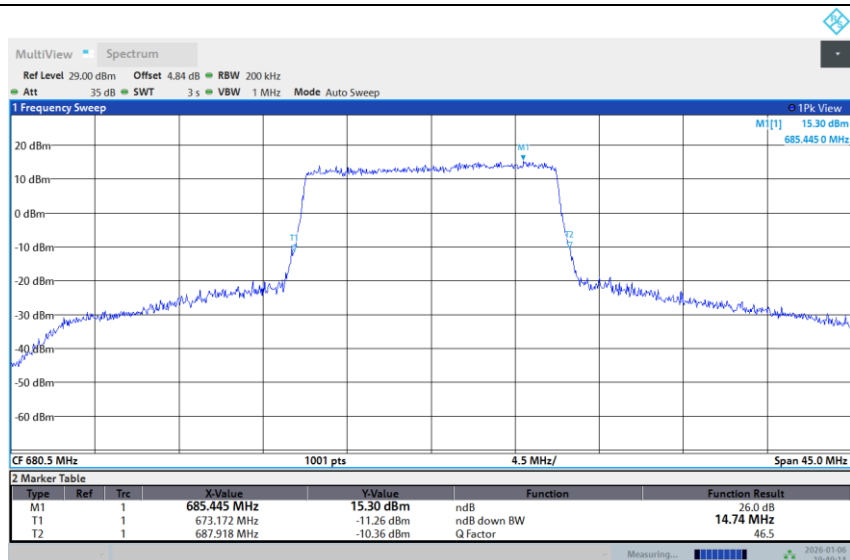
Band 71-15M-MID-64QAM-Full RB
