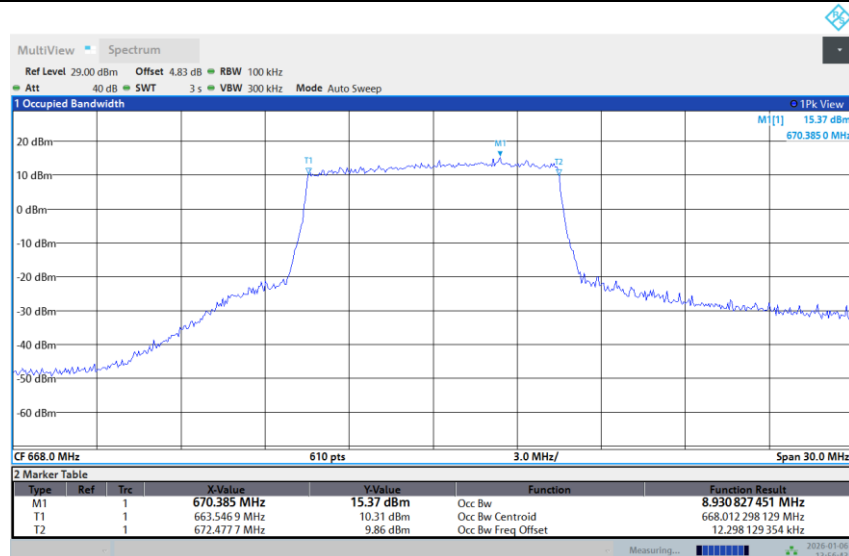
Band 71-10M-LOW-64QAM-Full RB
