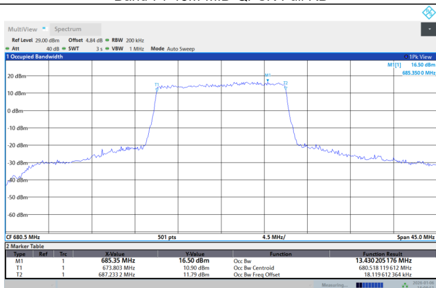
Band 71-15M-MID-16QAM-Full RB
