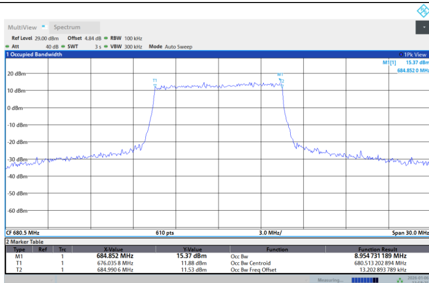
Band 71-10M-MID-16QAM-Full RB
