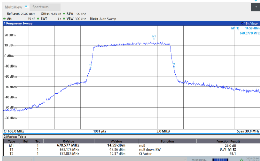
Band 71-10M-LOW-256QAM-Full RB
