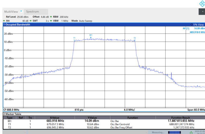
Band 71-20M-HIGH-64QAM-Full RB
