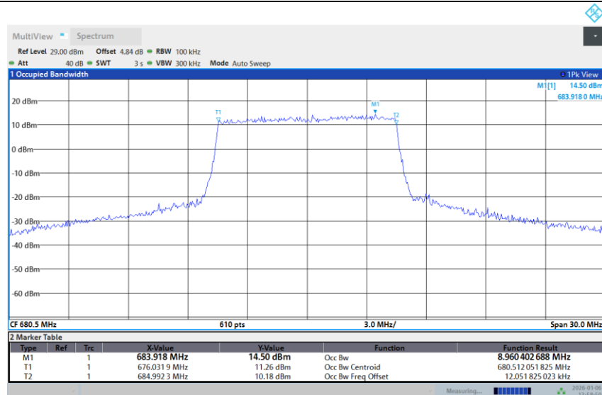
Band 71-10M-MID-64QAM-Full RB
