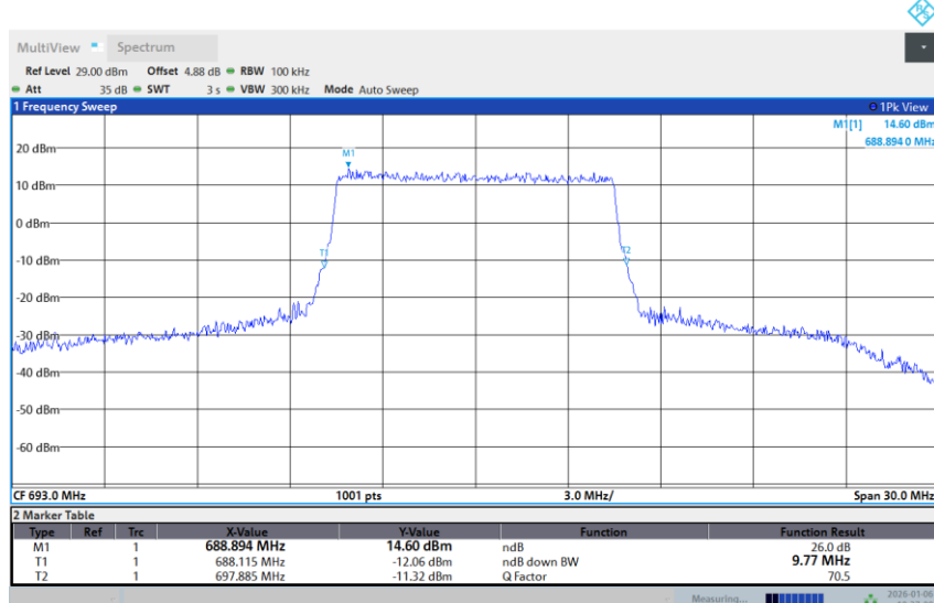
Band 71-10M-HIGH-16QAM-Full RB
