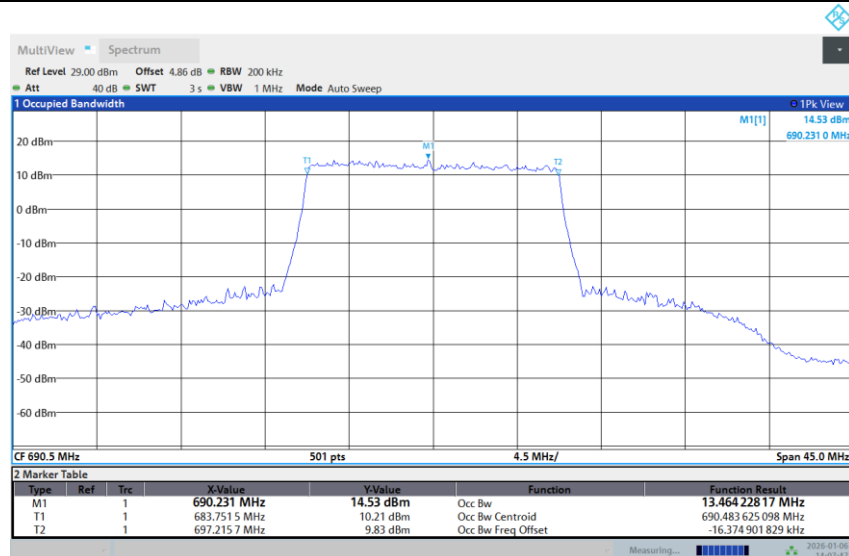
Band 71-15M-HIGH-256QAM-Full RB
