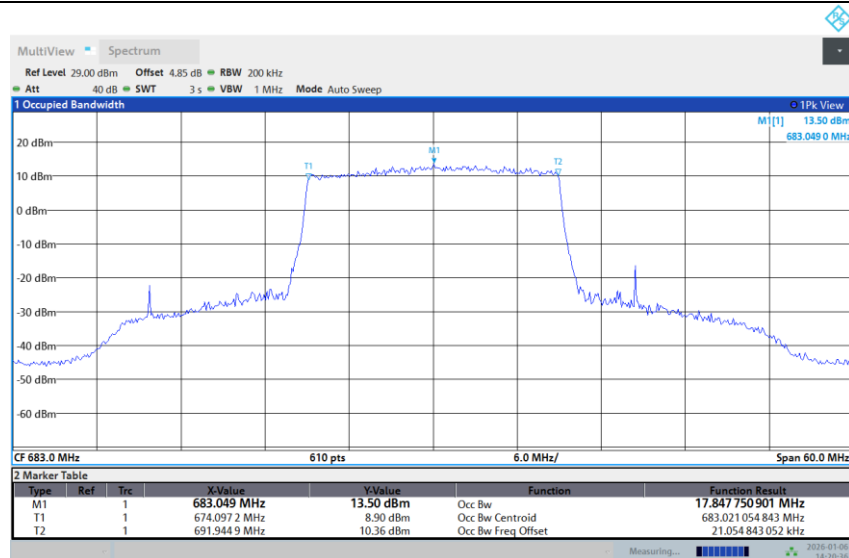
Band 71-20M-MID-256QAM-Full RB
