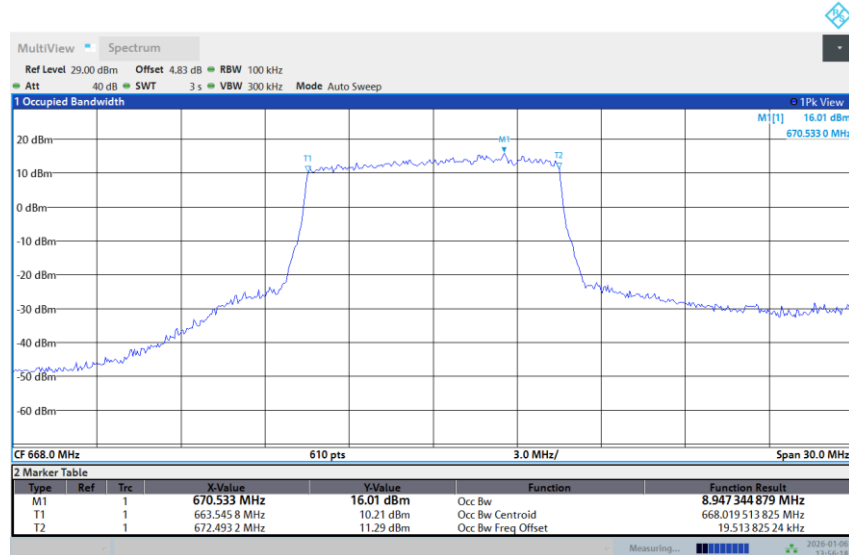
Band 71-10M-LOW-16QAM-Full RB
