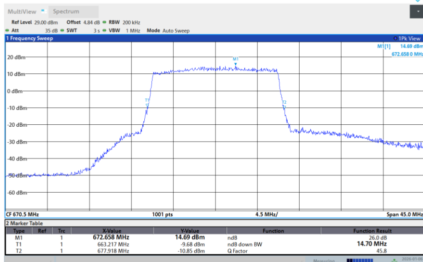
Band 71-15M-LOW-256QAM-Full RB
