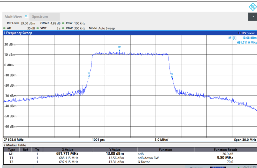
Band 71-10M-HIGH-256QAM-Full RB
