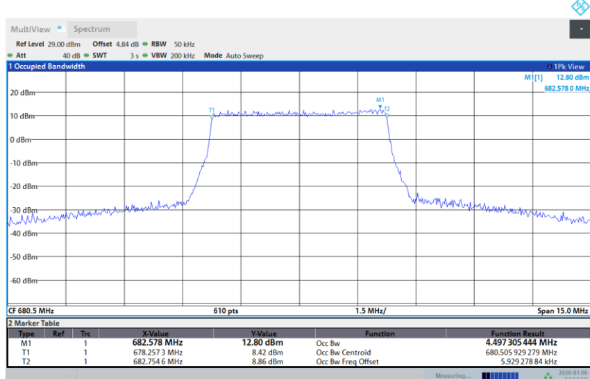
Band 71-5M-MID-256QAM-Full RB
