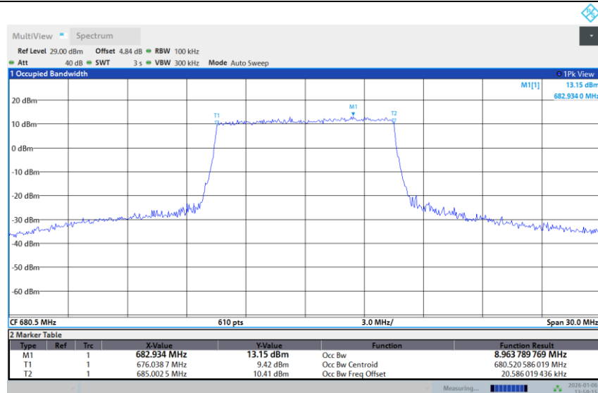
Band 71-10M-MID-256QAM-Full RB
