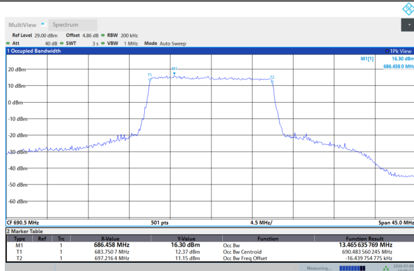
Band 71-15M-HIGH-16QAM-Full RB
