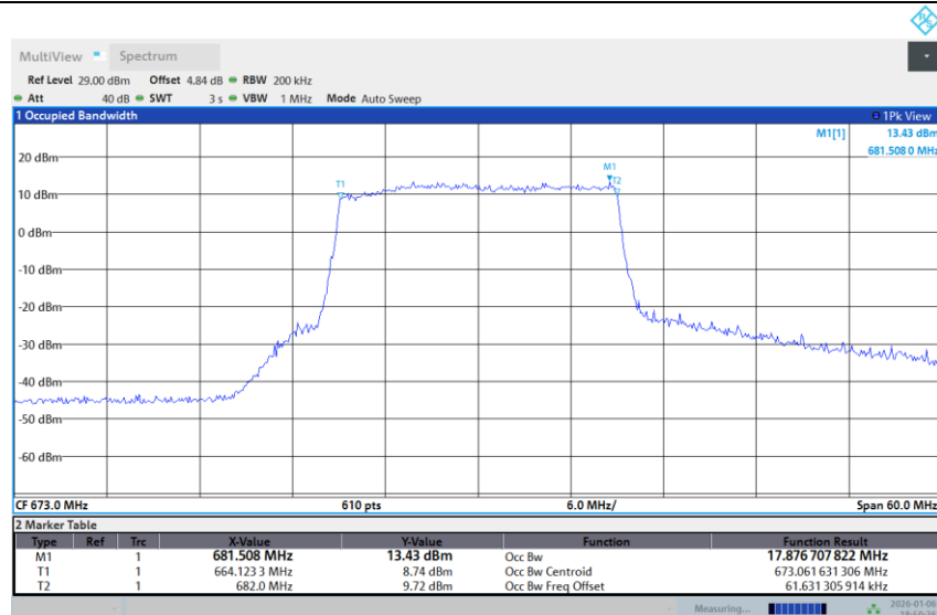
Band 71-20M-LOW-256QAM-Full RB
