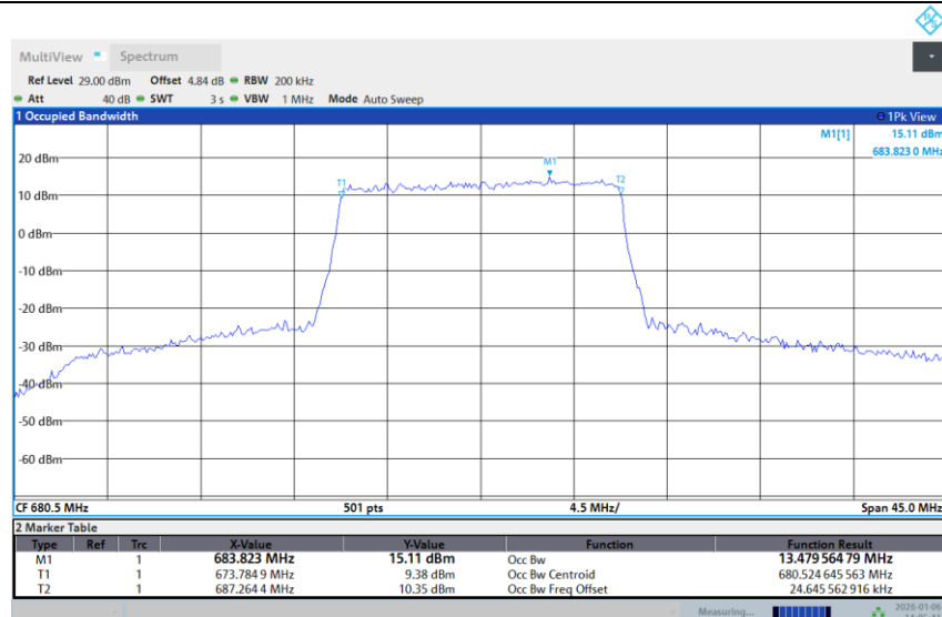
Band 71-15M-MID-256QAM-Full RB
