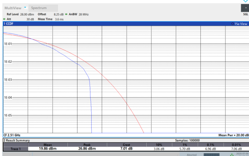
Band 7-20M-LOW-256QAM-Full RB
