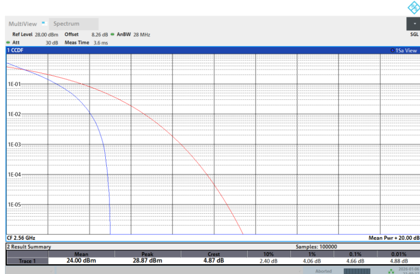
Band 7-20M-HIGH-16QAM-1RB Low
