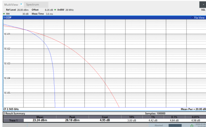
Band 7-10M-HIGH-64QAM-1RB Low
