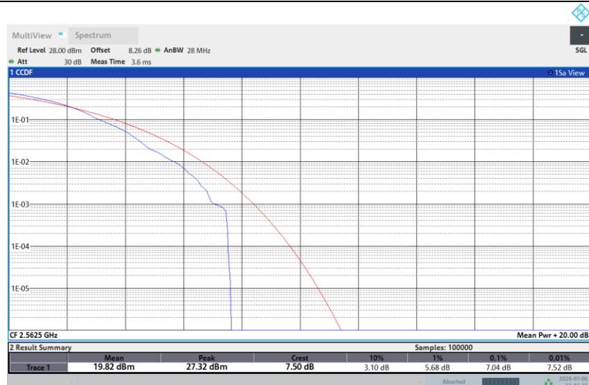
Band 7-15M-HIGH-256QAM-Full RB
