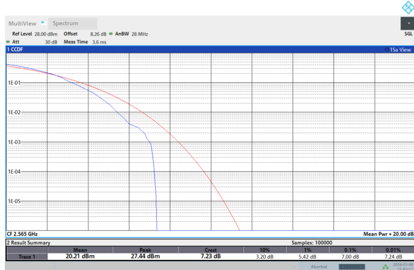
Band 7-10M-HIGH-256QAM-Full RB
