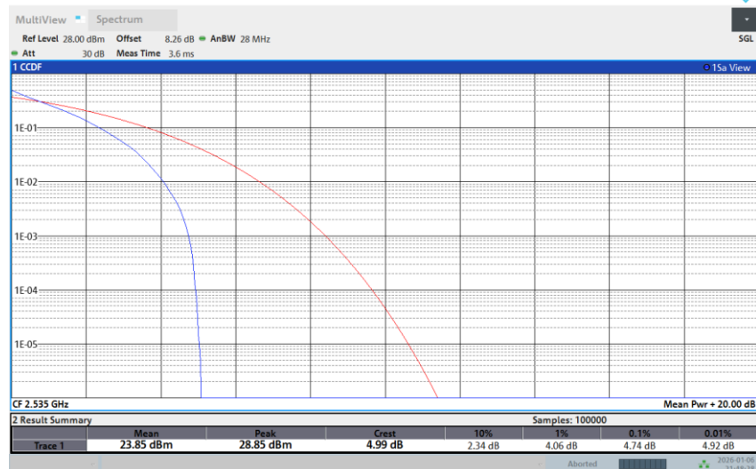
Band 7-20M-MID-16QAM-1RB Low
