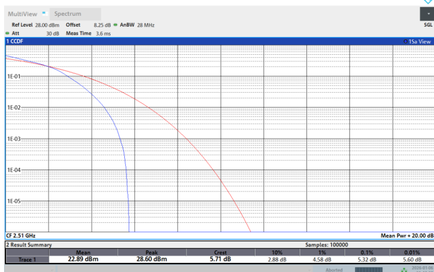
Band 7-20M-LOW-64QAM-1RB Low
