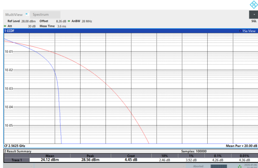
Band 7-15M-HIGH-16QAM-1RB Low
