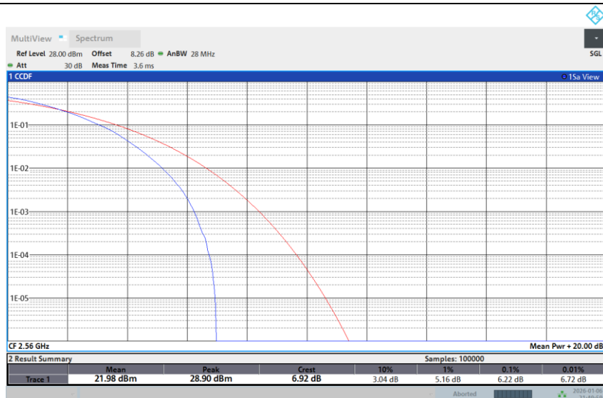
Band 7-20M-HIGH-256QAM-1RB Low
