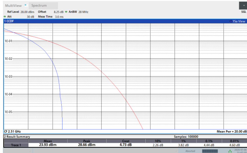
Band 7-20M-LOW-16QAM-1RB Low
