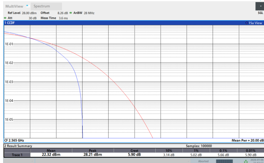
Band 7-10M-HIGH-256QAM-1RB Low
