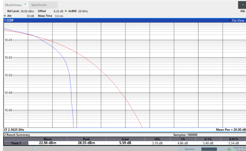
Band 7-15M-HIGH-64QAM-1RB Low
