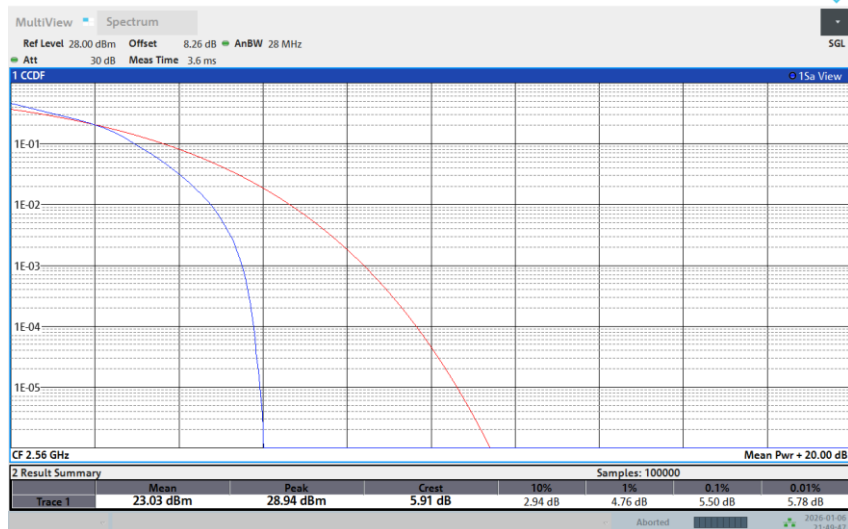
Band 7-20M-HIGH-64QAM-1RB Low
