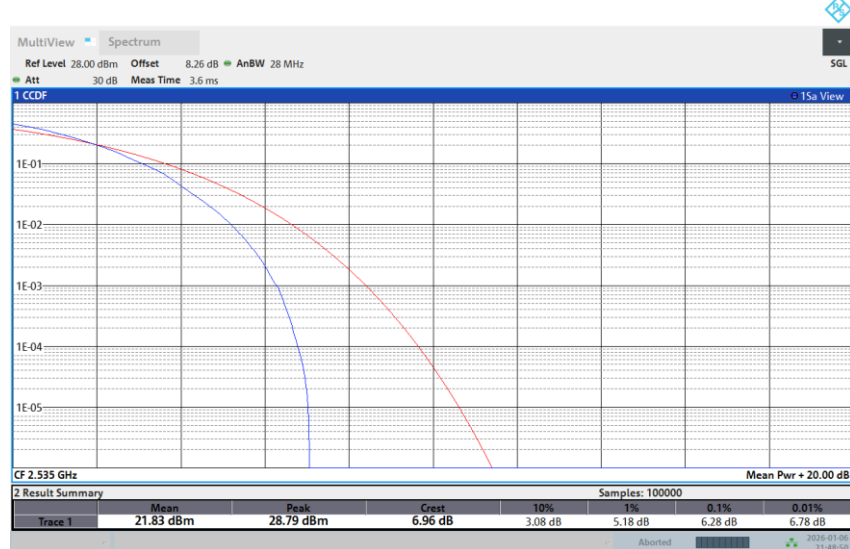
Band 7-20M-MID-256QAM-1RB Low
