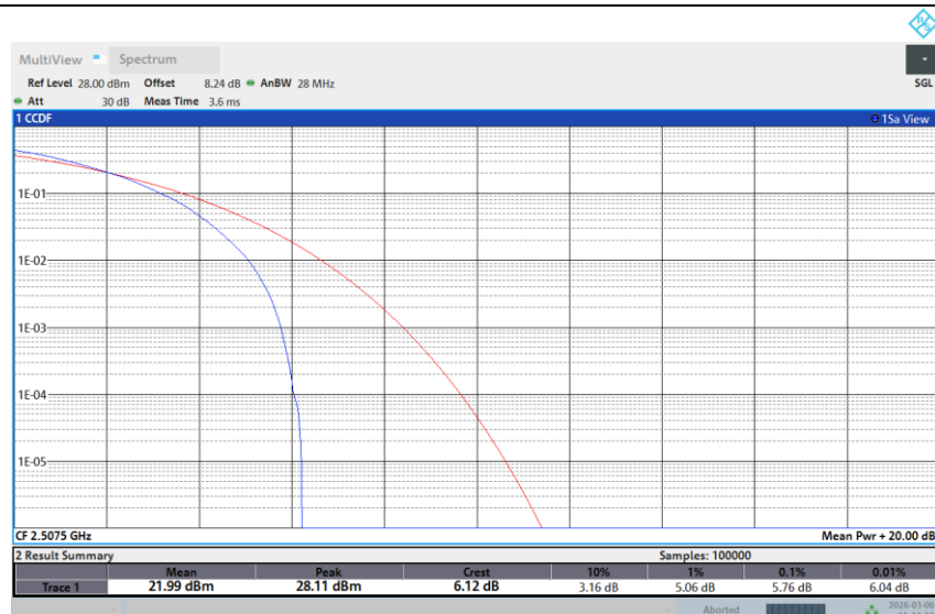
Band 7-15M-LOW-256QAM-1RB Low
