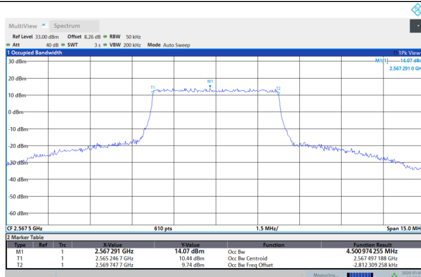
Band 7-5M-HIGH-256QAM-Full RB
