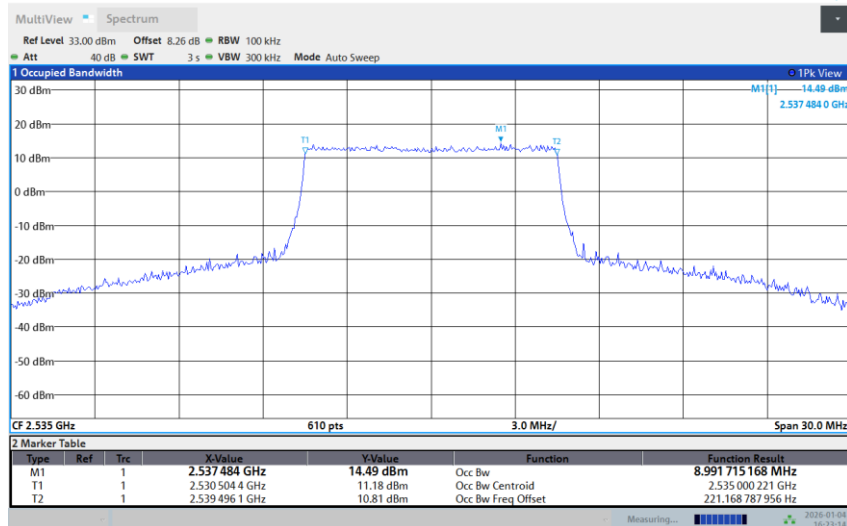
Band 7-10M-MID-256QAM-Full RB
