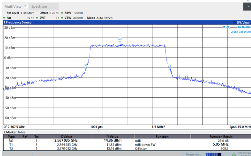
Band 7-5M-HIGH-256QAM-Full RB
