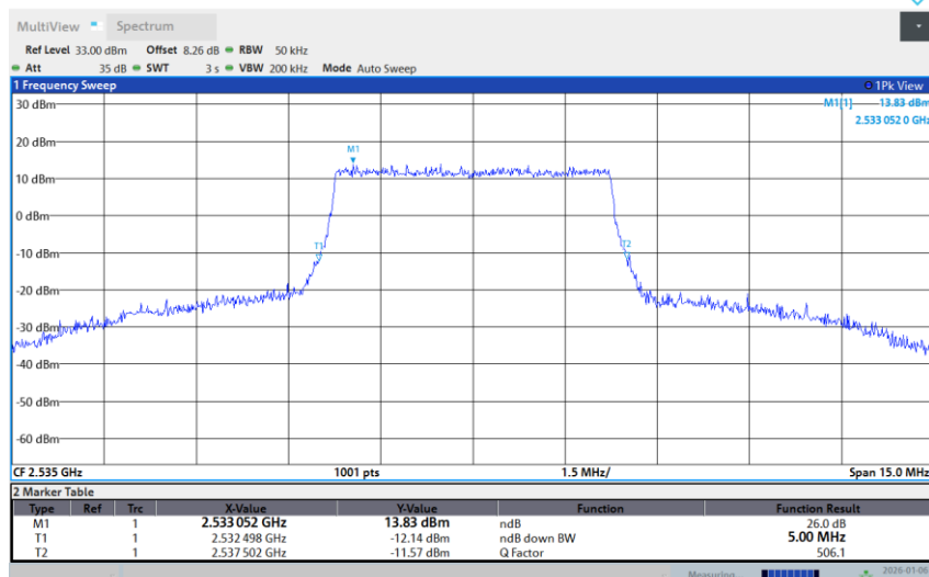
Band 7-5M-MID-256QAM-Full RB
