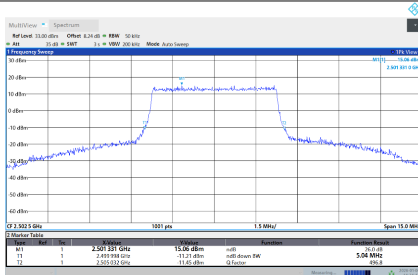
Band 7-5M-LOW-64QAM-Full RB
