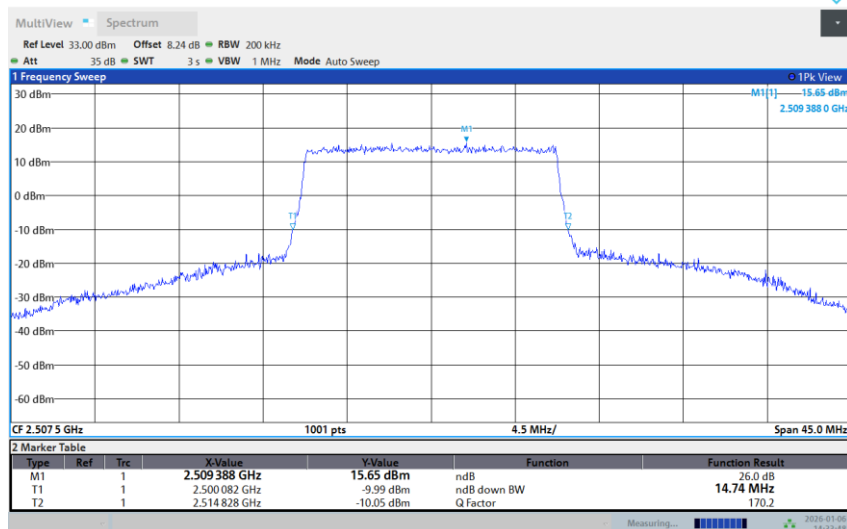
Band 7-15M-LOW-256QAM-Full RB
