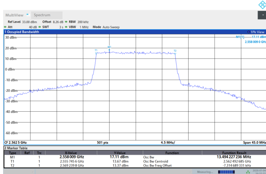
Band 7-15M-HIGH-64QAM-Full RB
