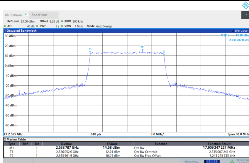
Band 7-20M-MID-256QAM-Full RB
