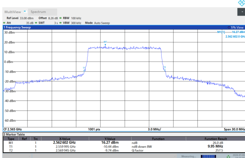
Band 7-10M-HIGH-16QAM-Full RB
