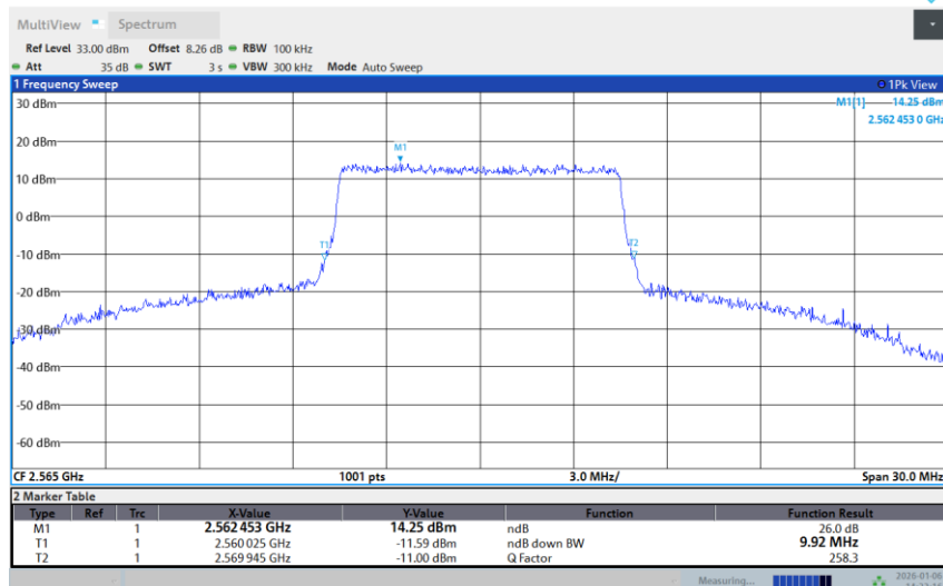
Band 7-10M-HIGH-256QAM-Full RB
