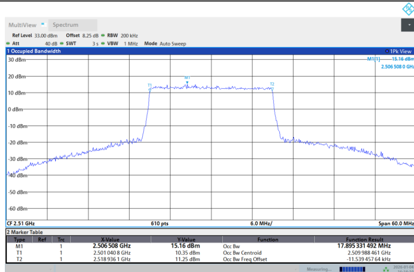
Band 7-20M-LOW-256QAM-Full RB
