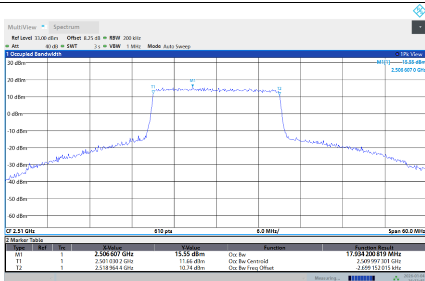
Band 7-20M-LOW-64QAM-Full RB
