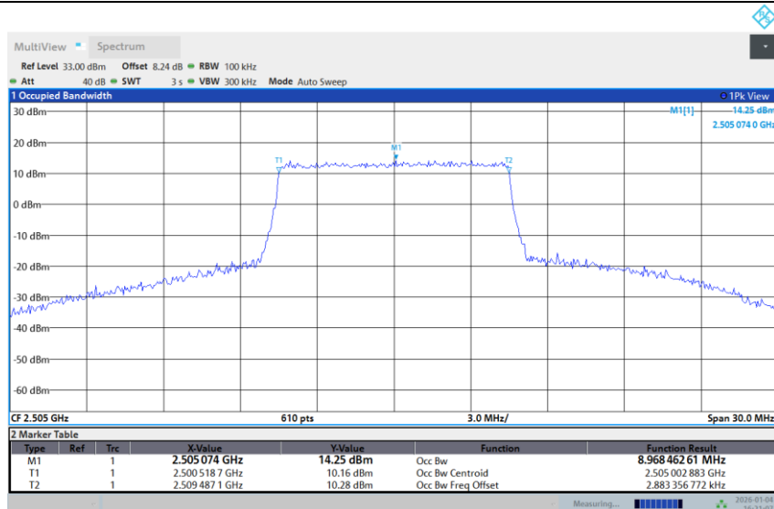
Band 7-10M-LOW-256QAM-Full RB
