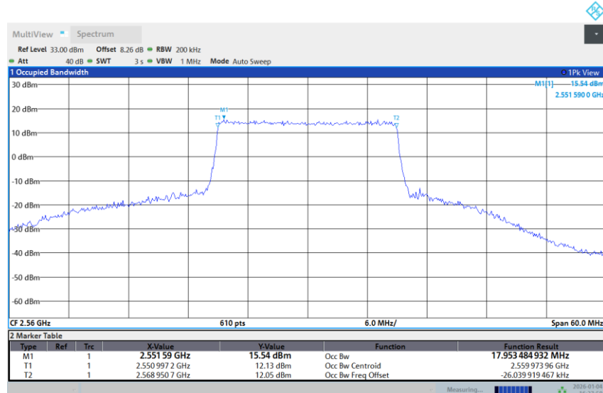
Band 7-20M-HIGH-64QAM-Full RB
