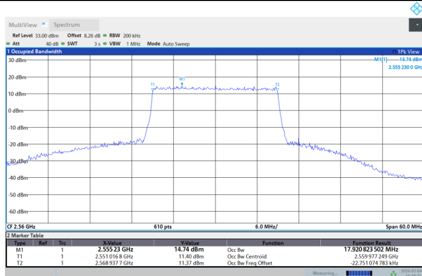
Band 7-20M-HIGH-256QAM-Full RB
