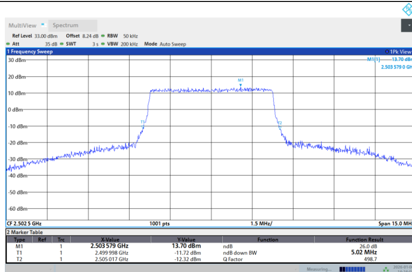
Band 7-5M-LOW-256QAM-Full RB
