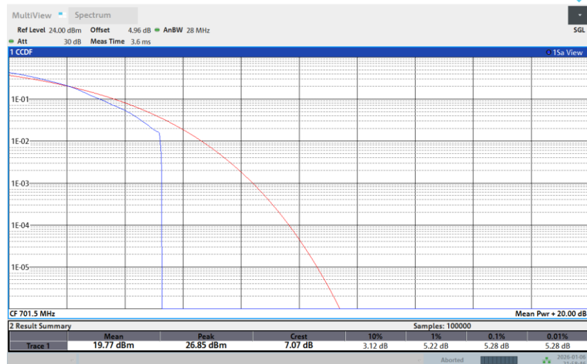
Band 12-5M-LOW-256QAM-Full RB
