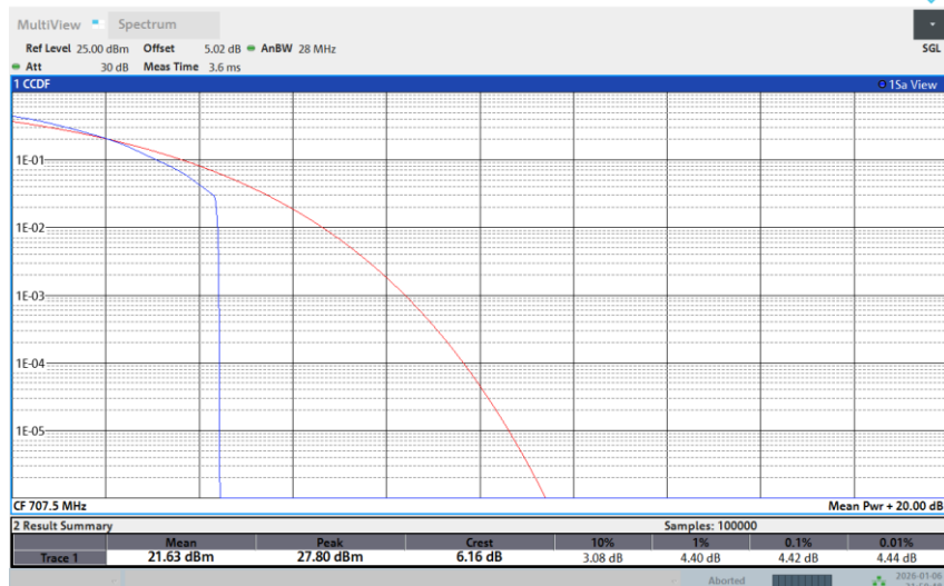
Band 12-5M-MID-256QAM-1RB Low
