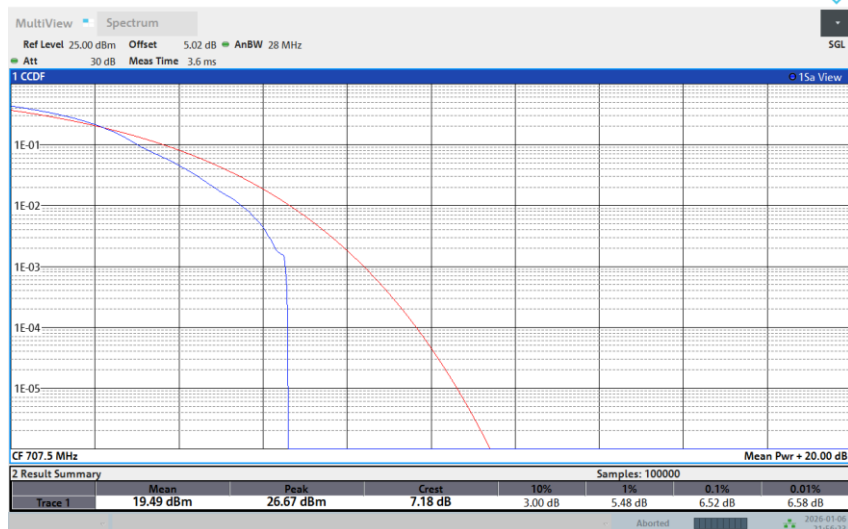
Band 12-3M-MID-256QAM-Full RB
