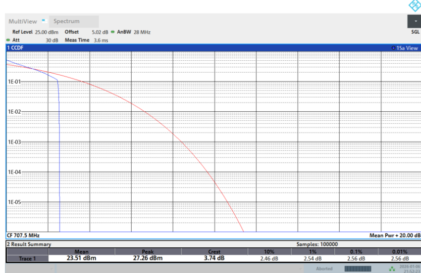
Band 12-1.4M-MID-QPSK-Full RB
