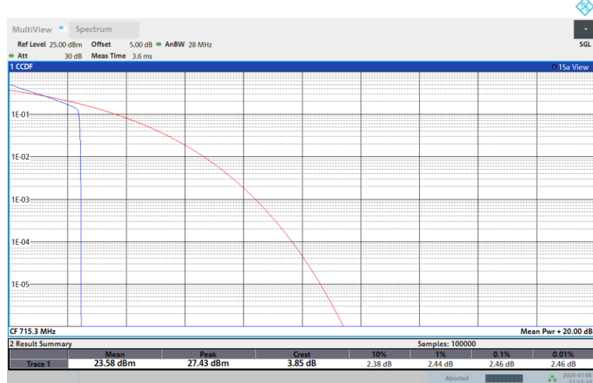
Band 12-1.4M-HIGH-QPSK-Full RB
