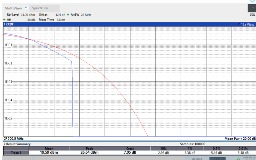
Band 12-3M-LOW-256QAM-Full RB
