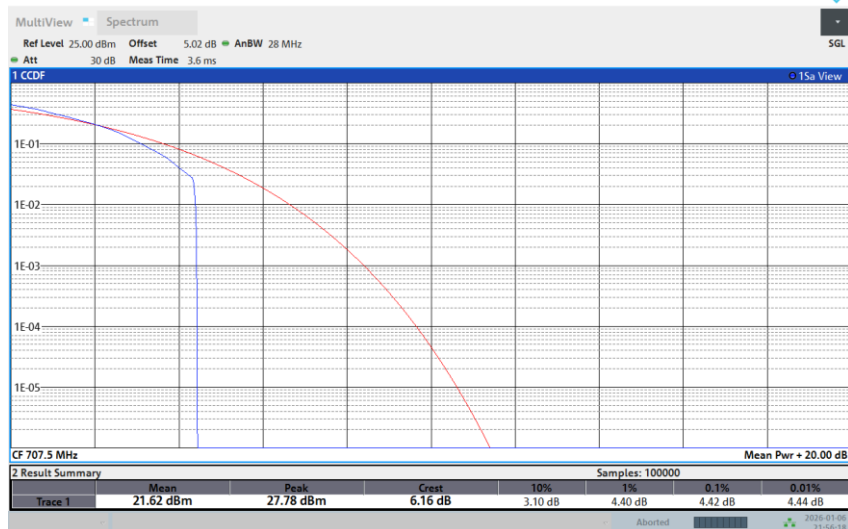
Band 12-3M-MID-256QAM-1RB Low
