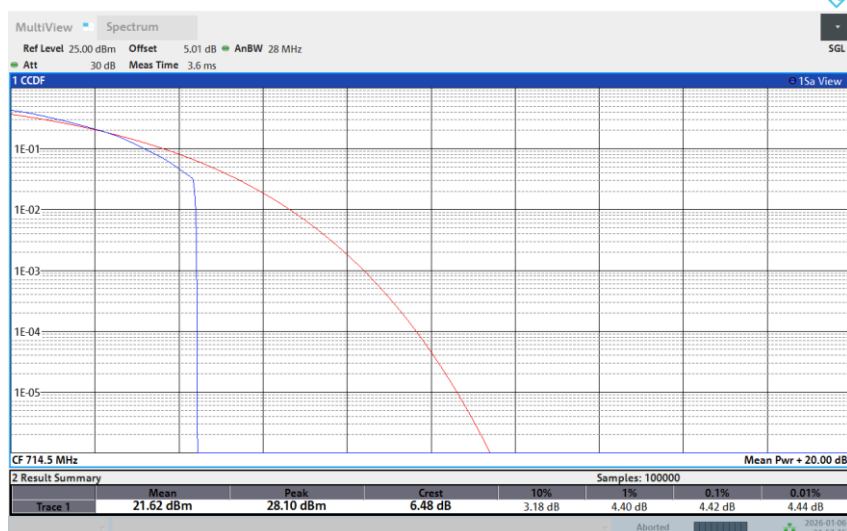
Band 12-3M-HIGH-256QAM-1RB Low
