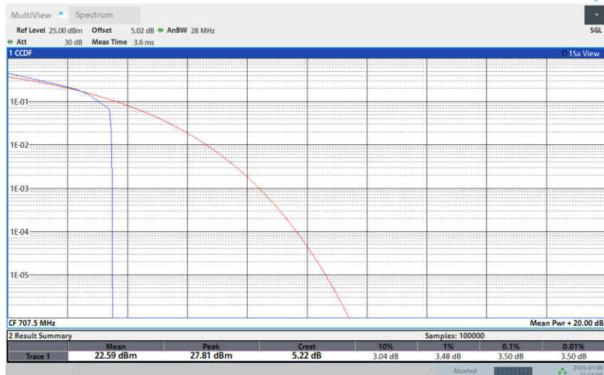
Band 12-3M-MID-64QAM-1RB Low
