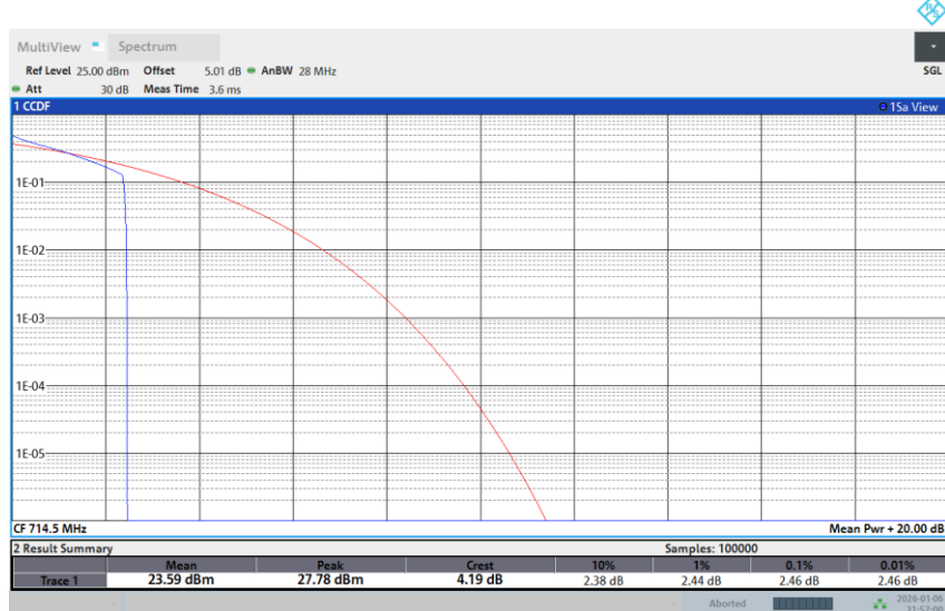
Band 12-3M-HIGH-QPSK-Full RB
