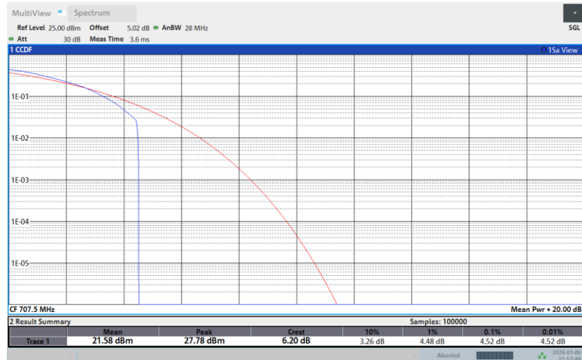
Band 12-1.4M-MID-256QAM-1RB Low
