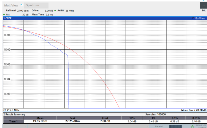
Band 12-1.4M-HIGH-256QAM-Full RB
