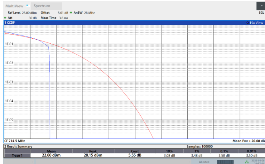
Band 12-3M-HIGH-64QAM-1RB Low
