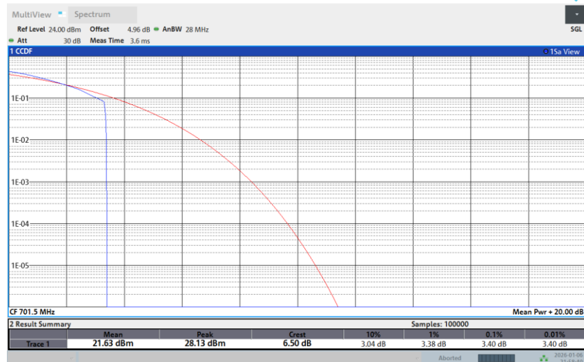
Band 12-5M-LOW-256QAM-1RB Low
