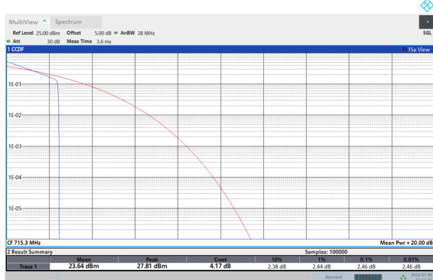
Band 12-1.4M-HIGH-16QAM-1RB Low
