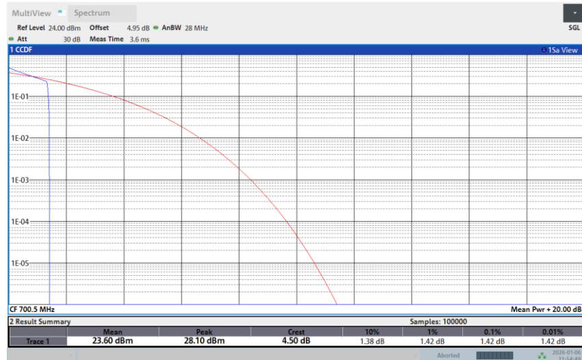
Band 12-3M-LOW-16QAM-1RB Low
