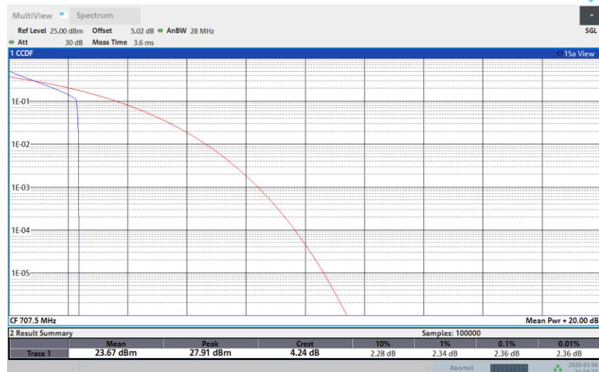
Band 12-5M-MID-16QAM-1RB Low
