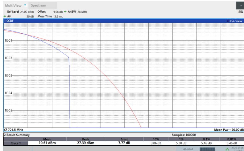
Band 12-5M-MID-QPSK-1RB Low
