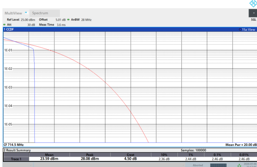
Band 12-3M-HIGH-16QAM-1RB Low
