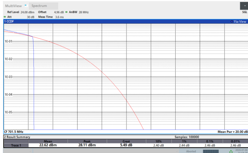
Band 12-5M-LOW-64QAM-1RB Low
