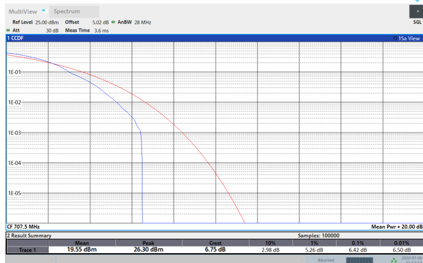
Band 12-1.4M-MID-256QAM-Full RB
