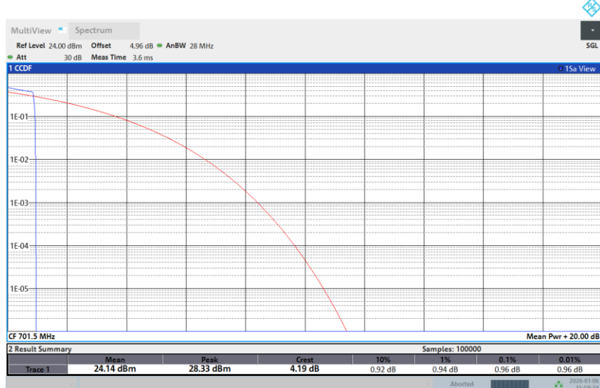
Band 12-5M-LOW-16QAM-Full RB
