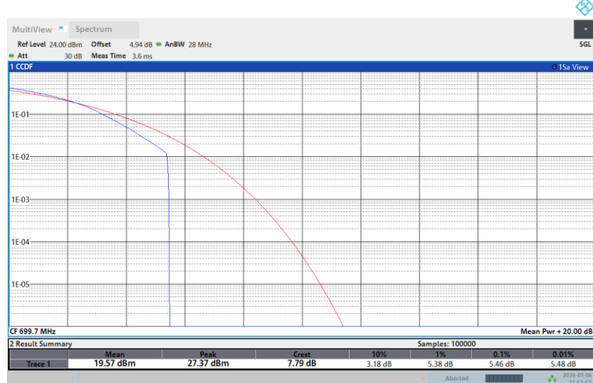
Band 12-1.4M-MID-QPSK-1RB Low
