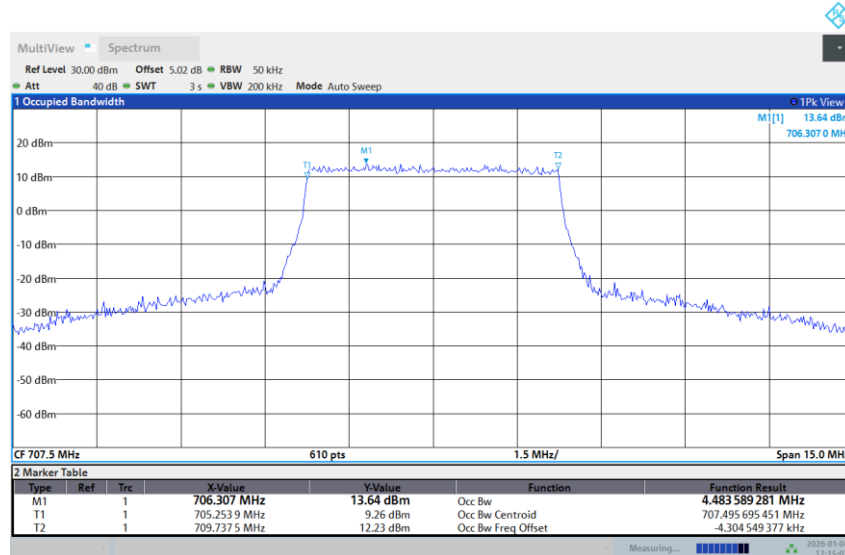
Band 12-5M-MID-256QAM-Full RB
