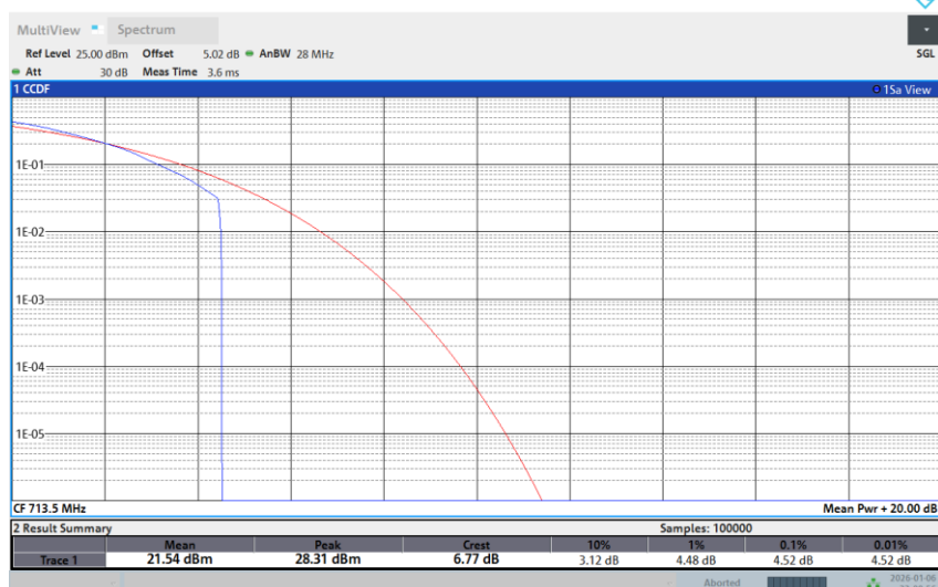
Band 12-5M-HIGH-256QAM-1RB Low
