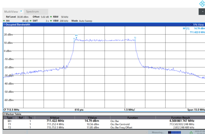
Band 12-5M-HIGH-64QAM-Full RB
