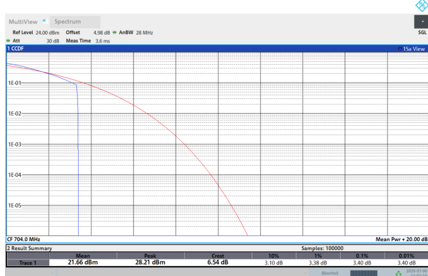
Band 12-10M-LOW-256QAM-1RB Low
