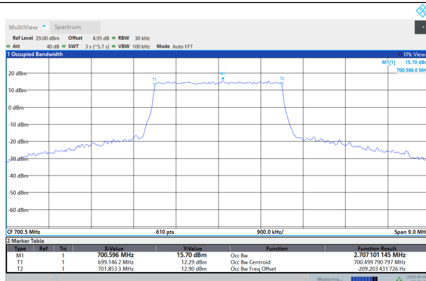
Band 12-3M-LOW-64QAM-Full RB
