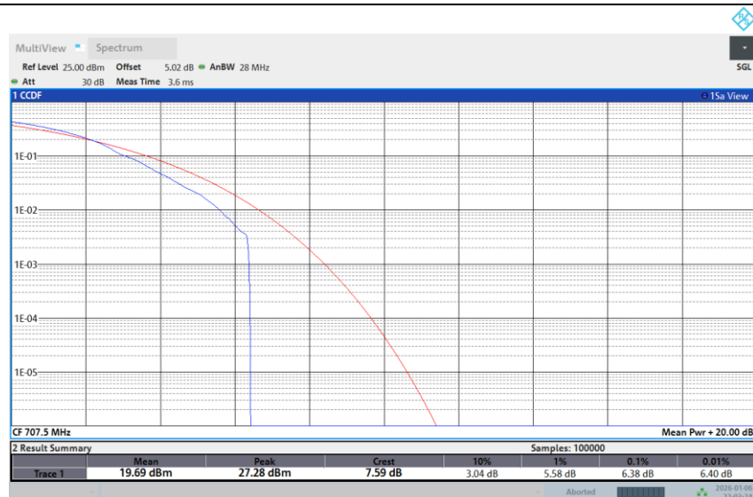
Band 12-10M-MID-256QAM-Full RB
