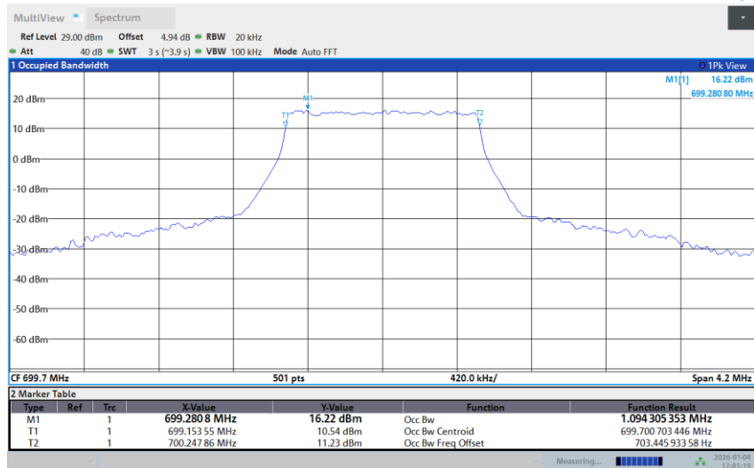
Band 12-1.4M-LOW-256QAM-Full RB
