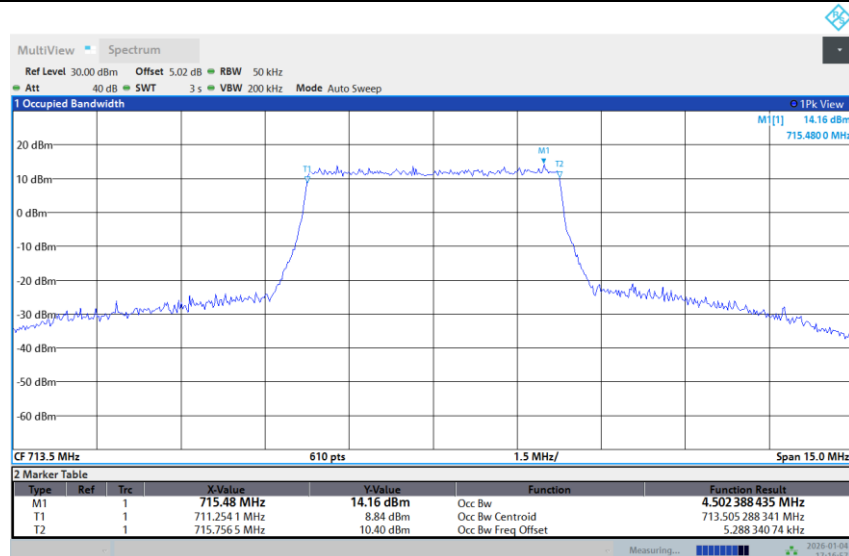
Band 12-5M-HIGH-256QAM-Full RB
