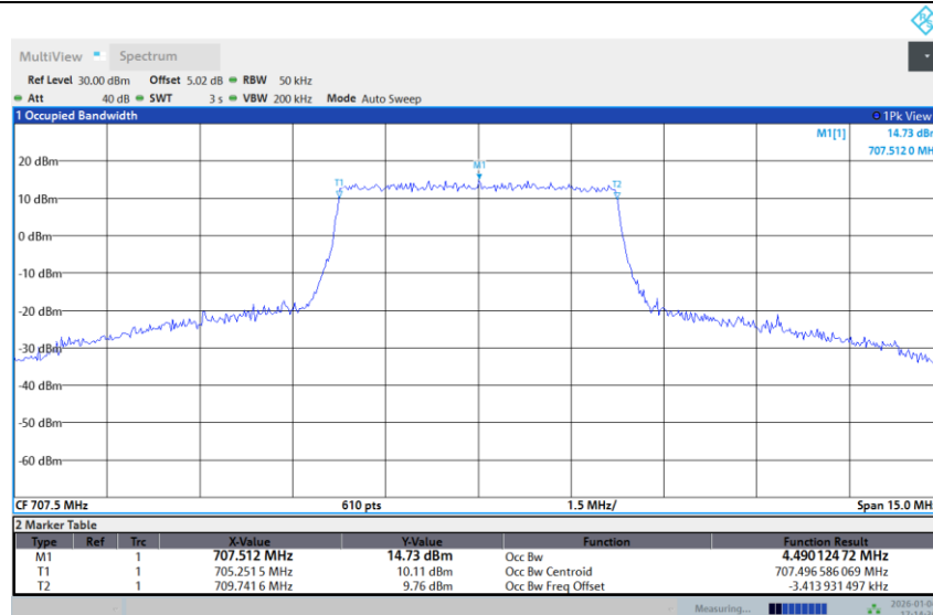
Band 12-5M-MID-64QAM-Full RB
