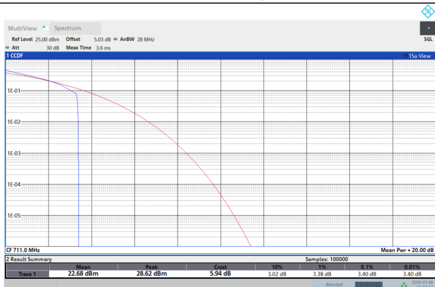
Band 12-10M-HIGH-64QAM-1RB Low
