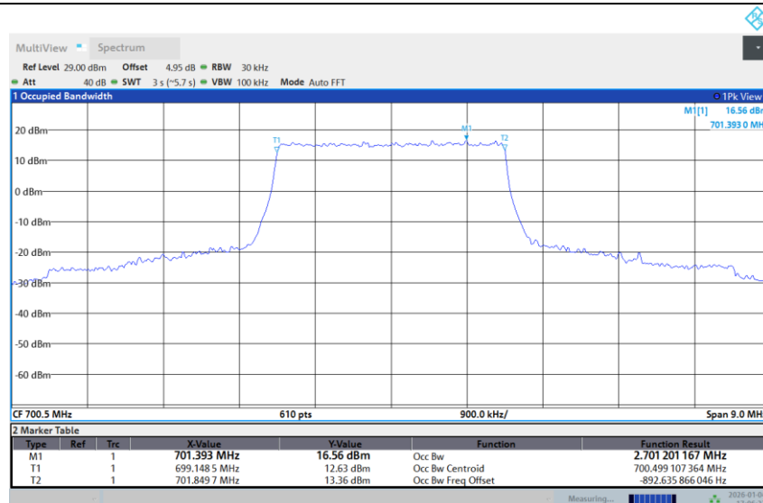
Band 12-3M-LOW-16QAM-Full RB
