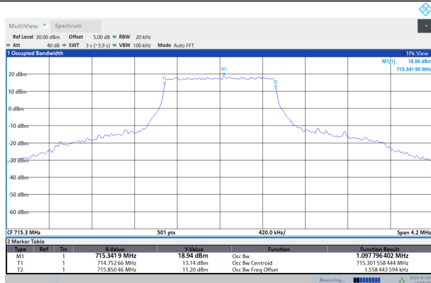
Band 12-1.4M-HIGH-16QAM-Full RB
