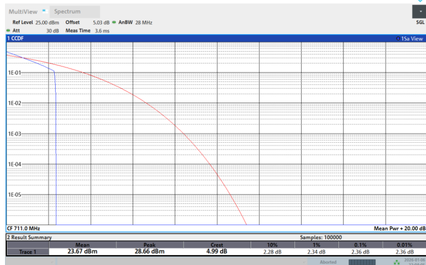
Band 12-10M-HIGH-16QAM-1RB Low
