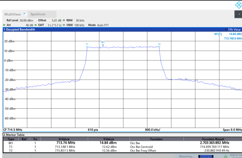
Band 12-3M-HIGH-256QAM-Full RB
