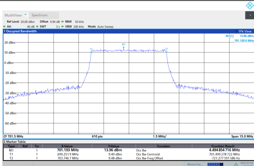
Band 12-5M-LOW-256QAM-Full RB
