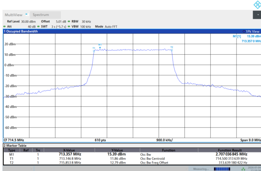
Band 12-3M-HIGH-64QAM-Full RB
