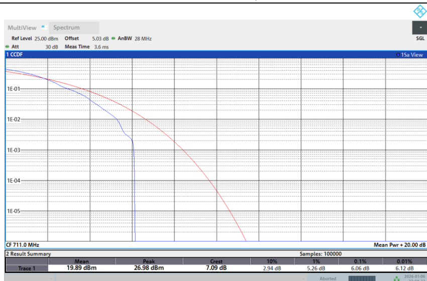
Band 12-10M-HIGH-256QAM-Full RB
