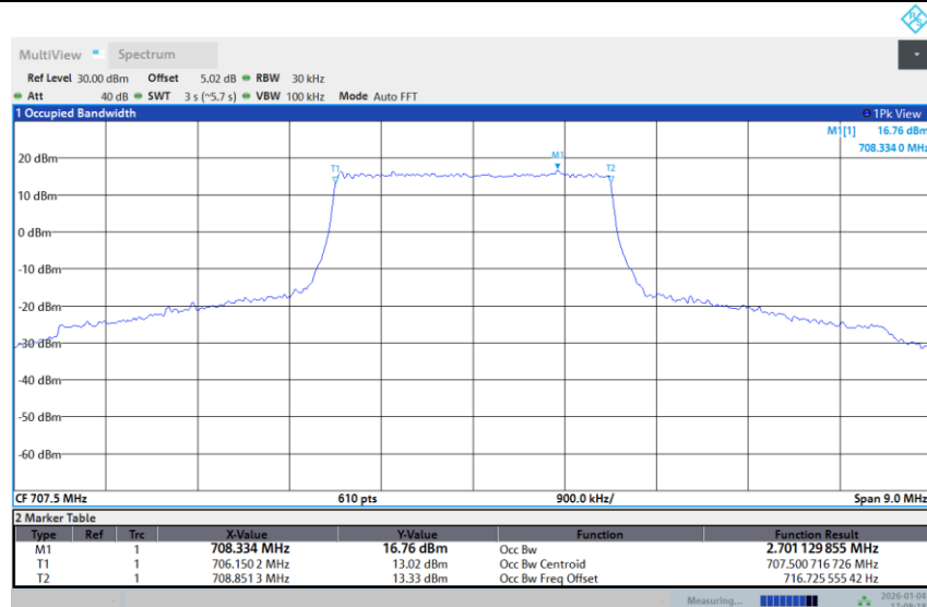
Band 12-3M-MID-16QAM-Full RB
