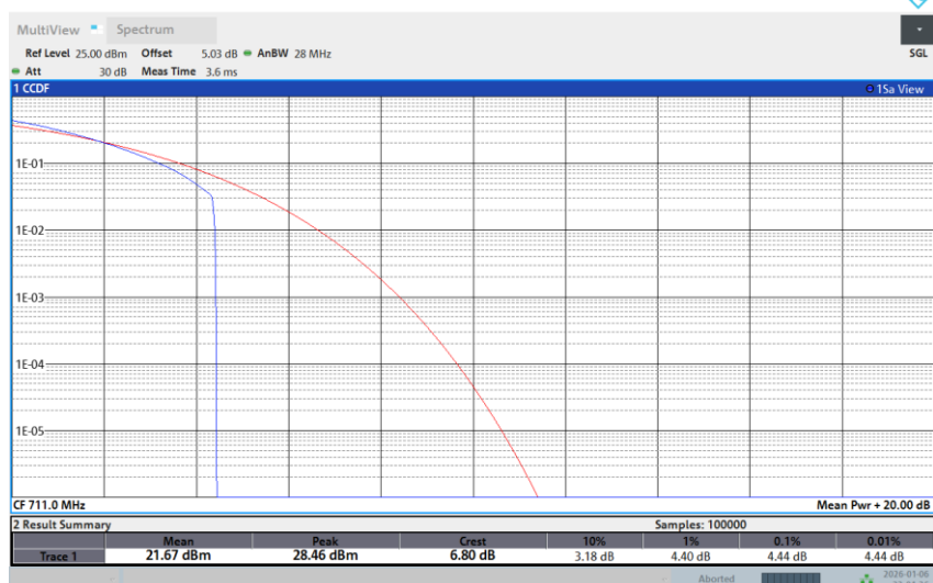
Band 12-10M-HIGH-256QAM-1RB Low
