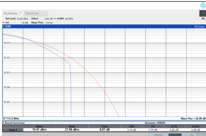
Band 12-5M-HIGH-256QAM-Full RB
