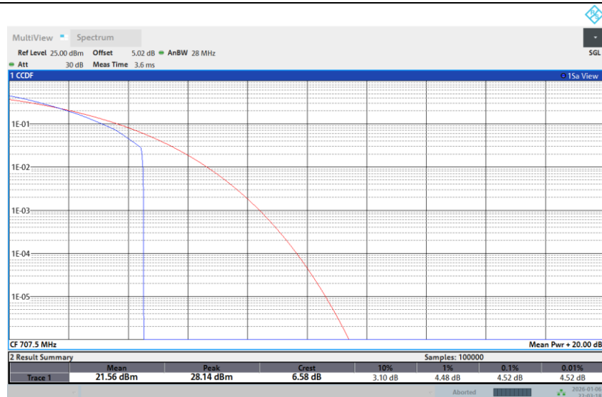
Band 12-10M-MID-256QAM-1RB Low
