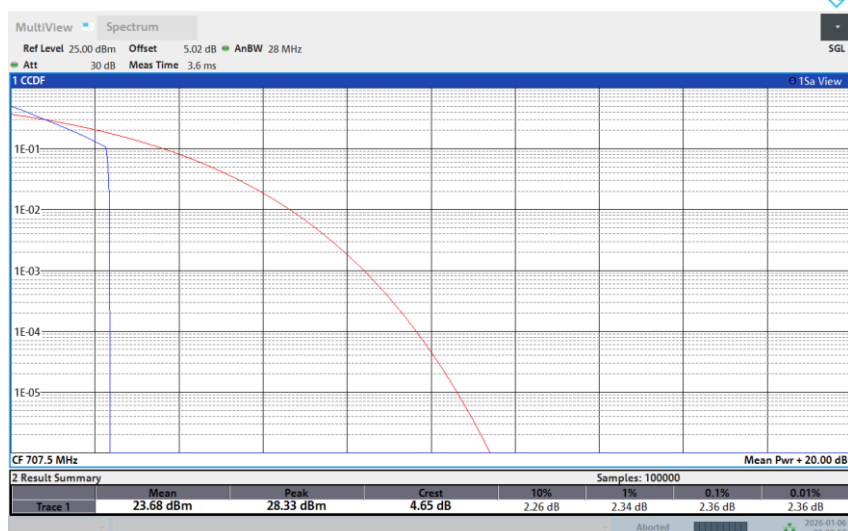
Band 12-10M-MID-16QAM-1RB Low
