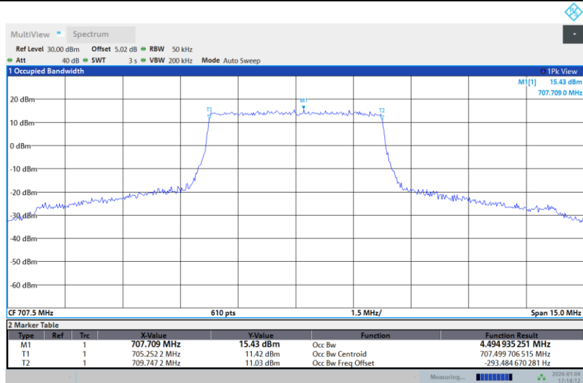
Band 12-5M-MID-16QAM-Full RB
