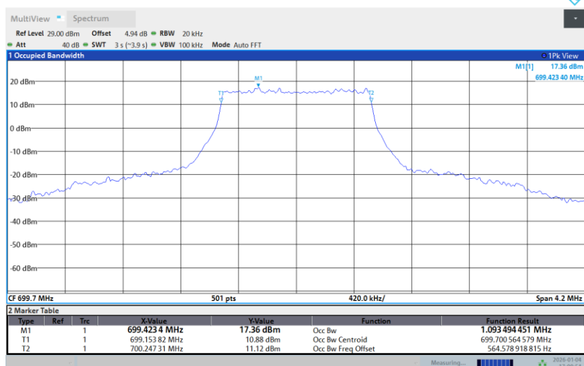
Band 12-1.4M-LOW-64QAM-Full RB
