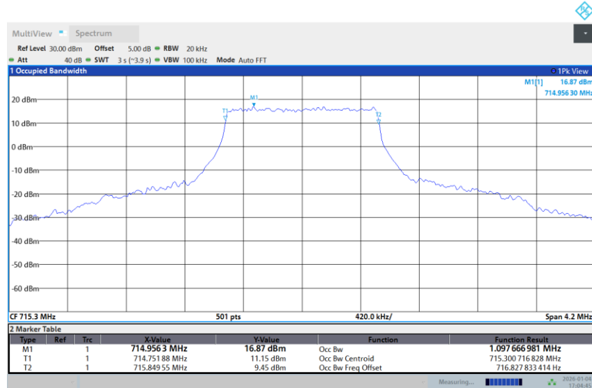
Band 12-1.4M-HIGH-64QAM-Full RB
