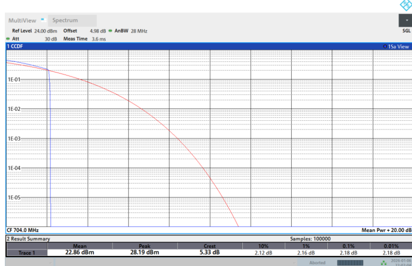
Band 12-10M-LOW-64QAM-Full RB
