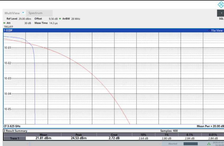
Band 48-20M-MID-QPSK-Full RB
