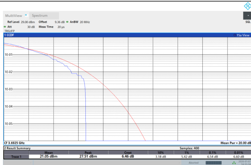
Band 48-15M-HIGH-256QAM-1RB Low
