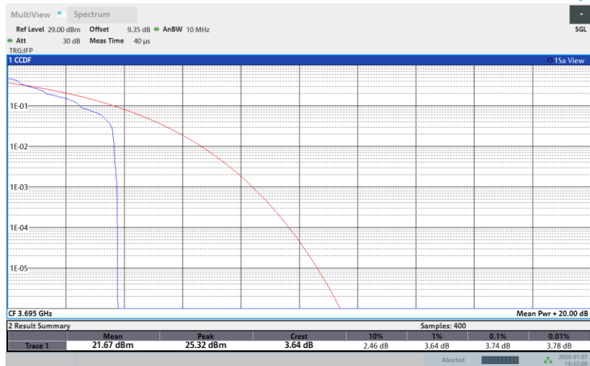
Band 48-10M-HIGH-64QAM-Full RB
