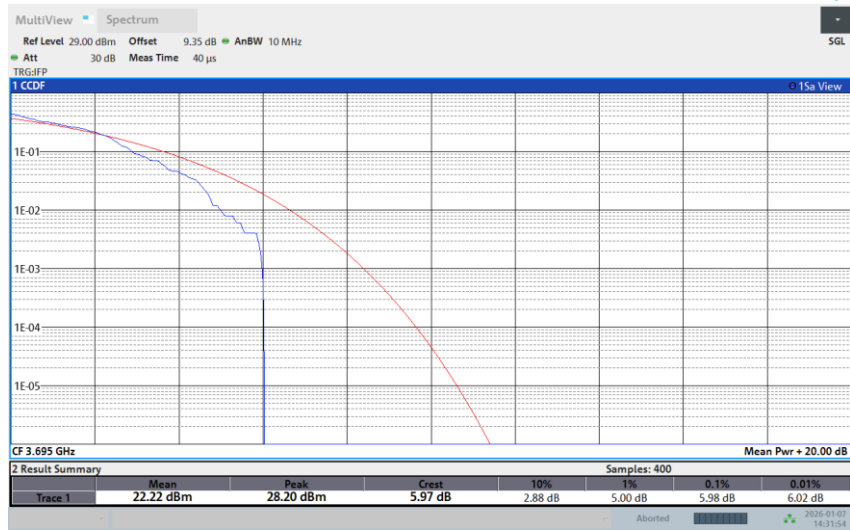
Band 48-10M-HIGH-64QAM-1RB Low
