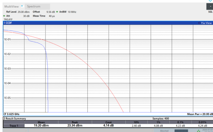
Band 48-10M-MID-256QAM-Full RB
