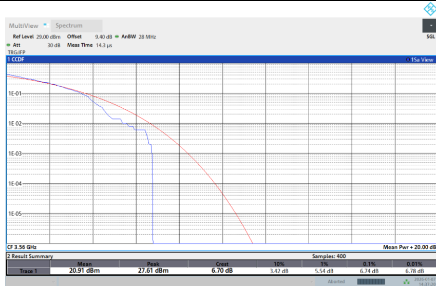
Band 48-20M-LOW-256QAM-1RB Low
