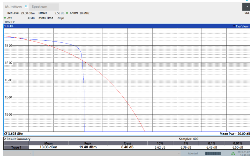
Band 48-15M-MID-256QAM-Full RB
