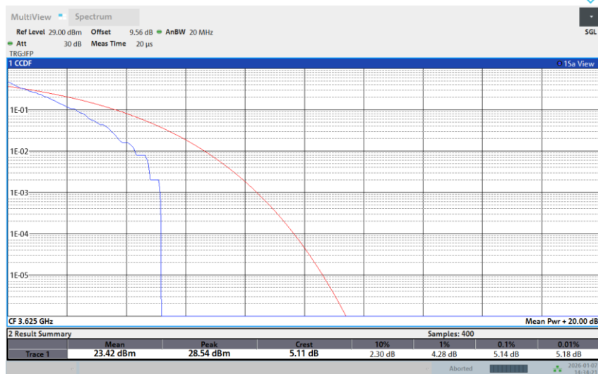
Band 48-15M-MID-16QAM-1RB Low
