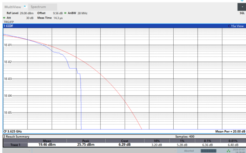
Band 48-20M-HIGH-QPSK-1RB Low
