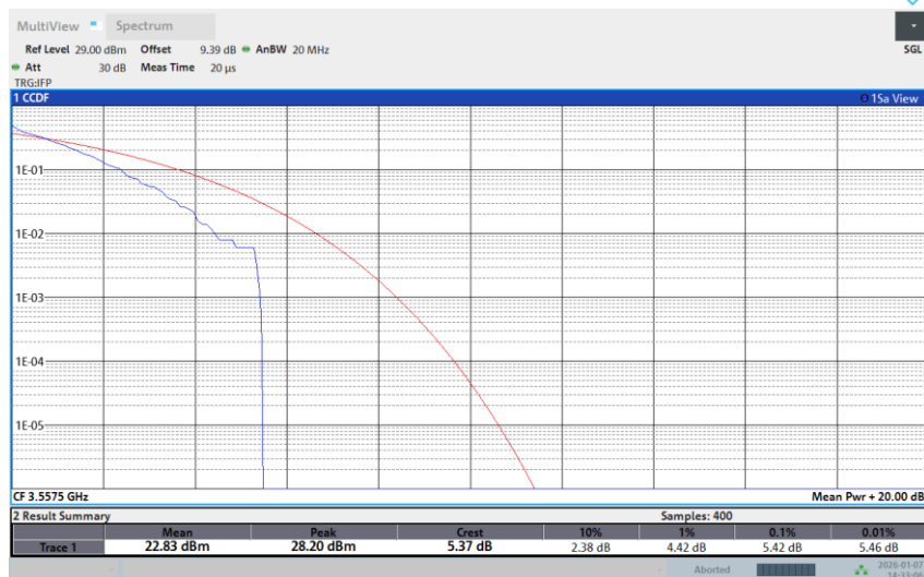
Band 48-15M-LOW-16QAM-1RB Low
