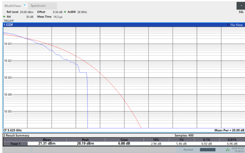
Band 48-20M-MID-256QAM-1RB Low
