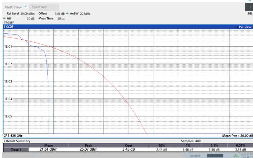
Band 48-15M-MID-64QAM-Full RB
