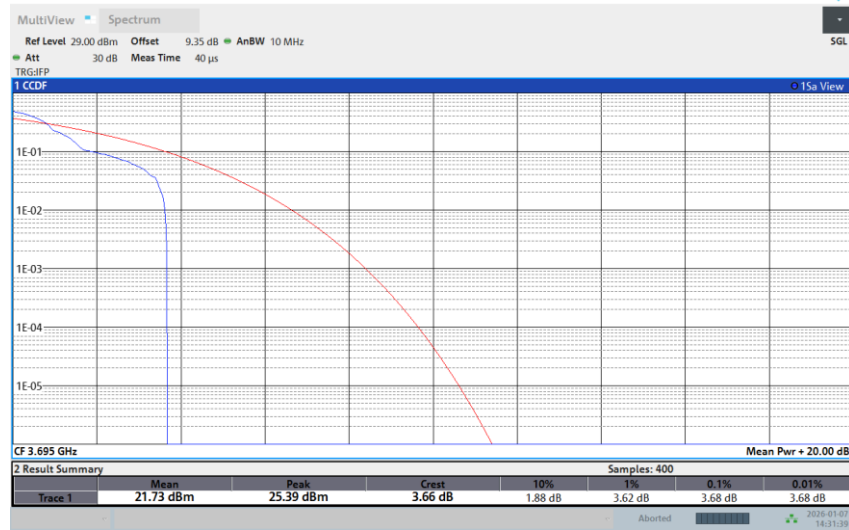
Band 48-10M-HIGH-QPSK-Full RB
