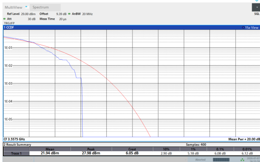
Band 48-15M-LOW-64QAM-1RB Low
