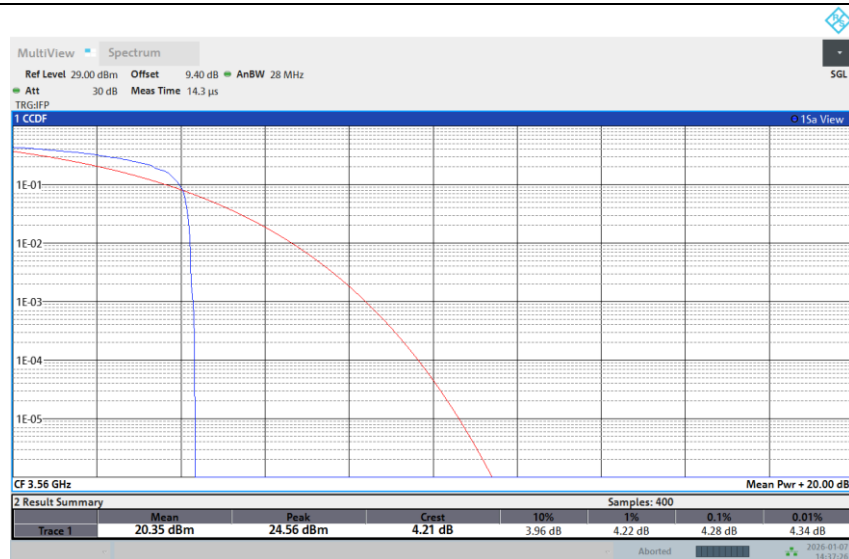
Band 48-20M-LOW-256QAM-Full RB
