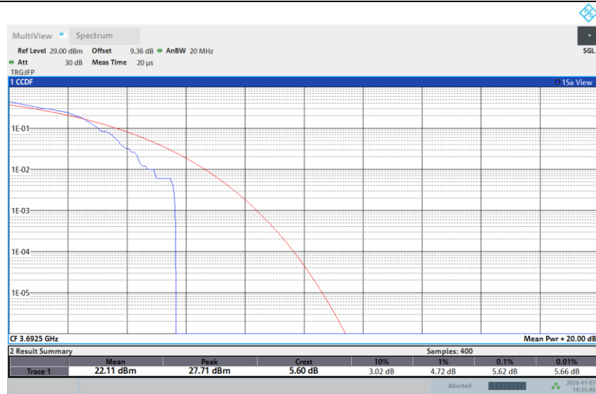
Band 48-15M-HIGH-64QAM-1RB Low
