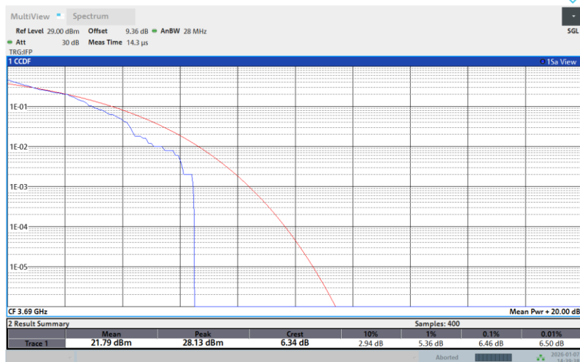
Band 48-20M-HIGH-64QAM-1RB Low
