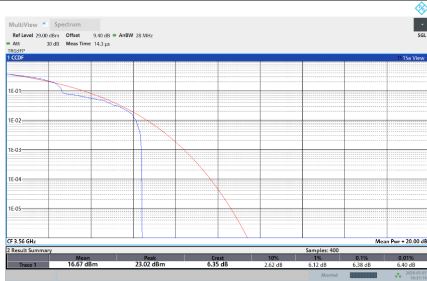
Band 48-20M-LOW-64QAM-Full RB
