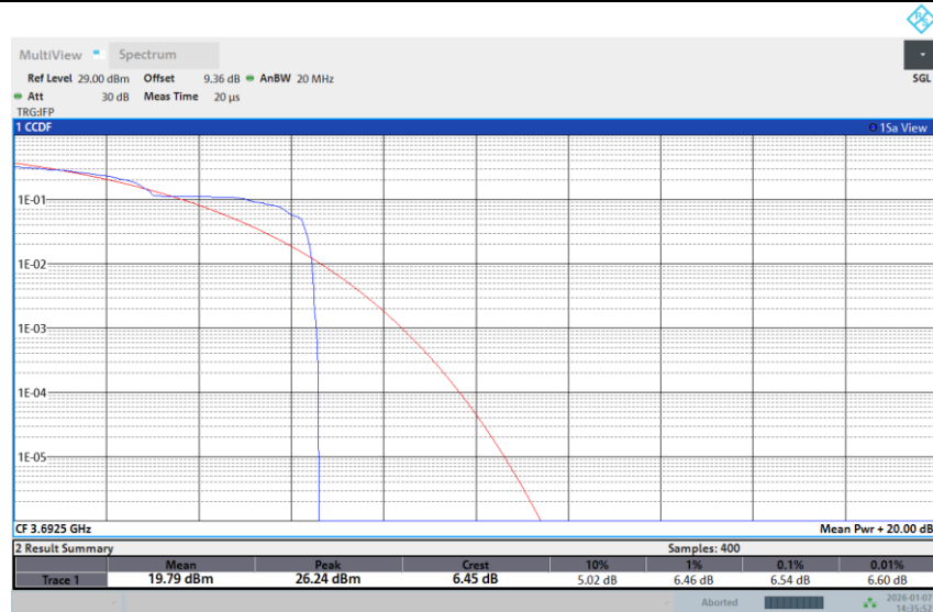
Band 48-15M-HIGH-64QAM-Full RB
