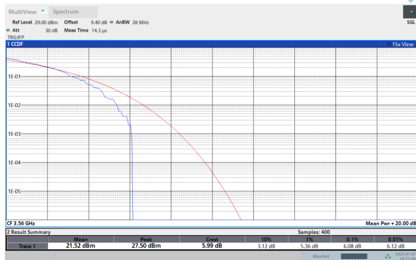
Band 48-20M-LOW-64QAM-1RB Low
