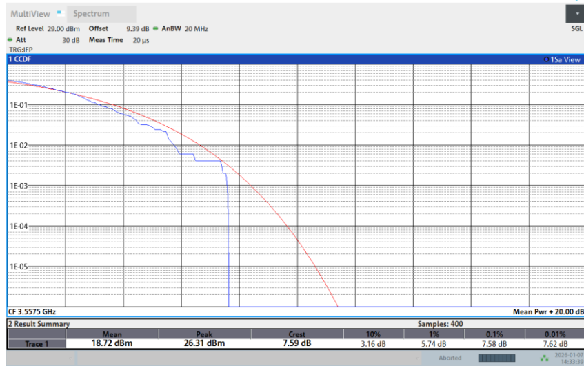
Band 48-15M-MID-QPSK-1RB Low
