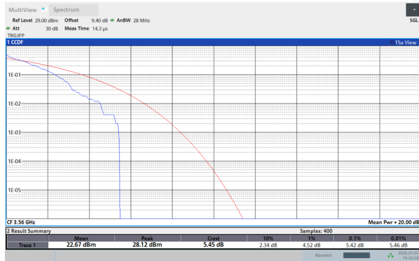
Band 48-20M-LOW-16QAM-1RB Low
