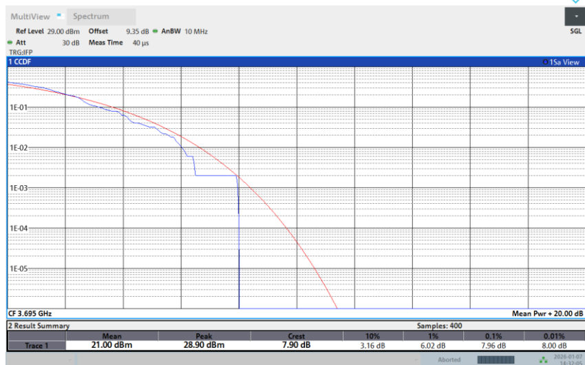
Band 48-10M-HIGH-256QAM-1RB Low
