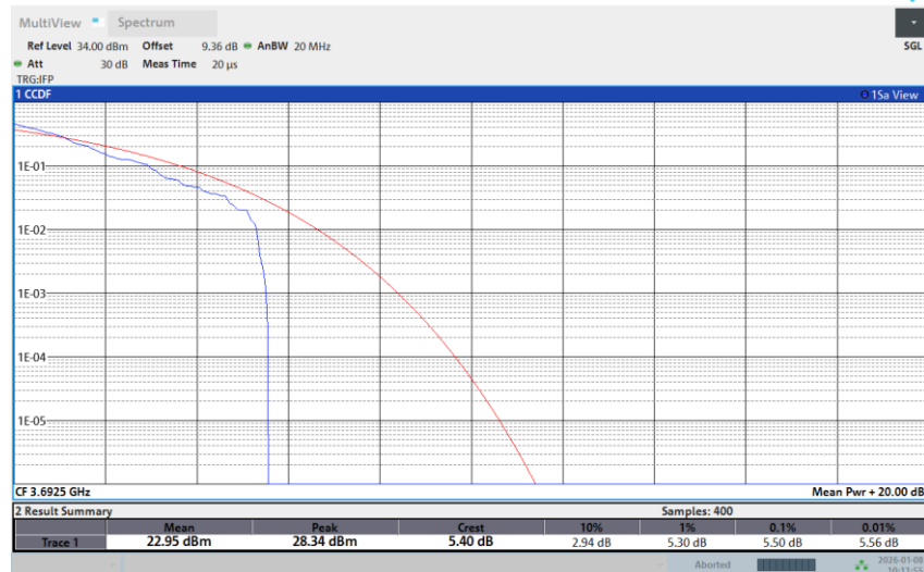
Band 48-15M-HIGH-16QAM-1RB Low
