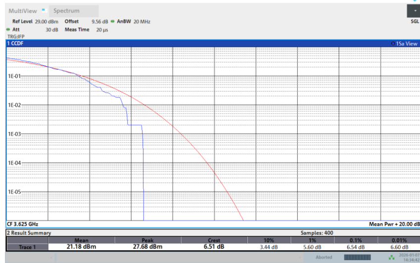
Band 48-15M-MID-256QAM-1RB Low
