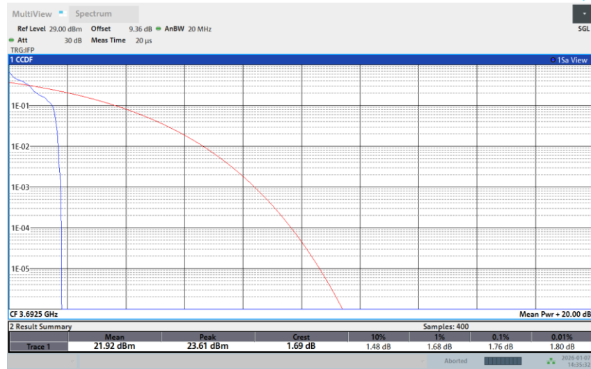
Band 48-15M-HIGH-QPSK-Full RB
