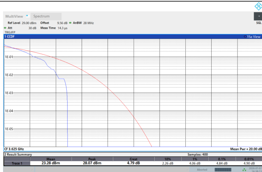
Band 48-20M-MID-16QAM-1RB Low
