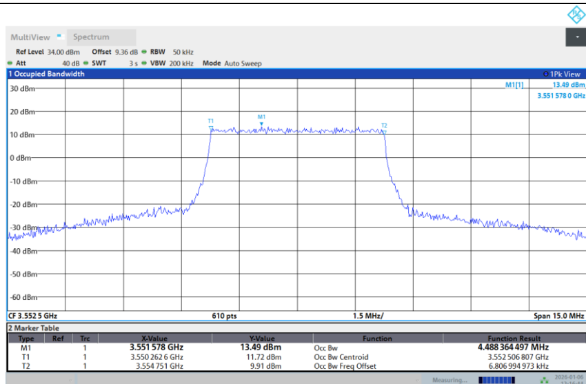
Band 48-5M-LOW-64QAM-Full RB
