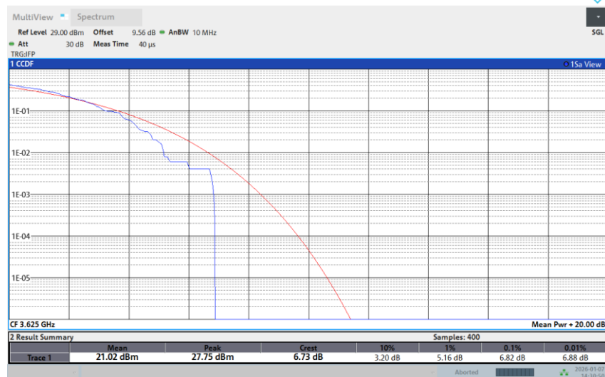
Band 48-10M-MID-256QAM-1RB Low
