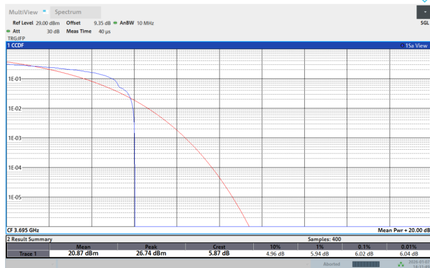
Band 48-10M-HIGH-16QAM-Full RB
