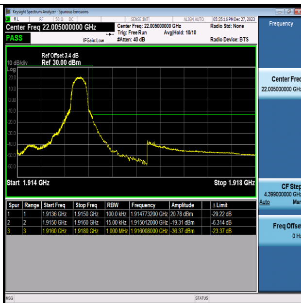
Band25 1.4MHz 16QAM 26683 1RB#5
