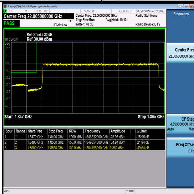
Band25 15MHz 16QAM 26115 75RB#0
