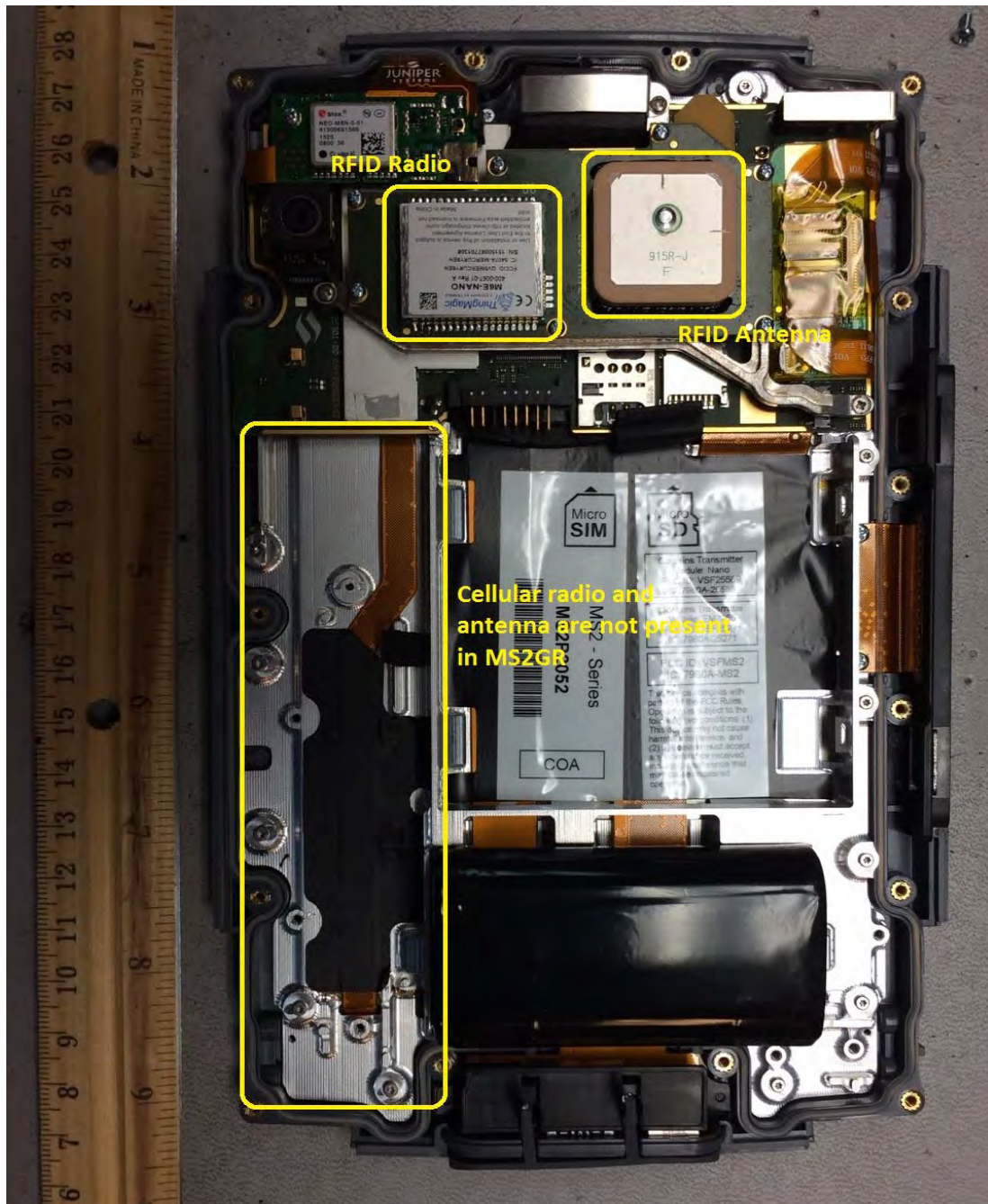
RFID radio and antenna in MS2GR
