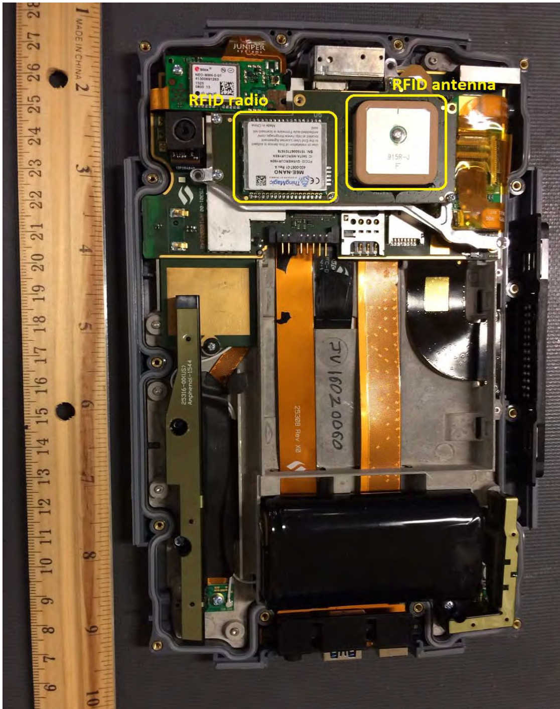
RFID radio and antenna in MS2GCR
