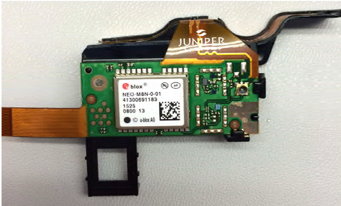
MS2 GNSS flex (front)
