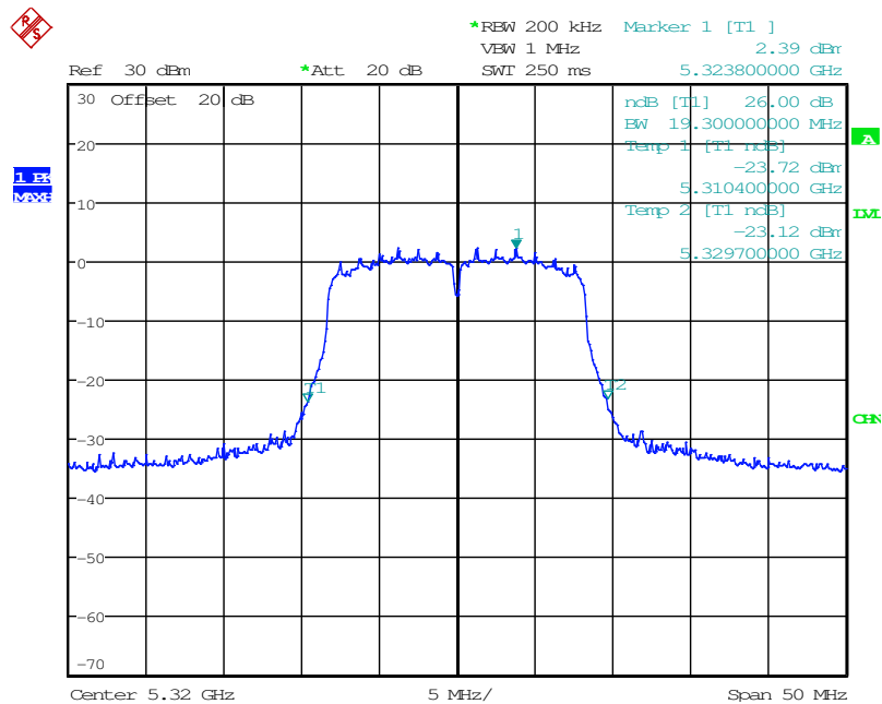
Figure 7.2.2-54: 26 dB EBW - Middle Channel
