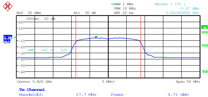
Figure 7.3.2-55: RF Output Power - Middle Channel
