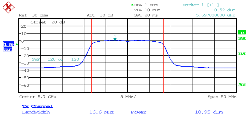
Figure 7.3.2-46: RF Output Power - Middle Channel
