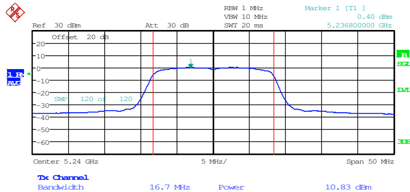
Figure 7.3.2-12: RF Output Power - Middle Channel
