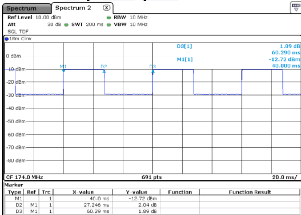
Figure 7-1 VHF Digital Transmission Plot
