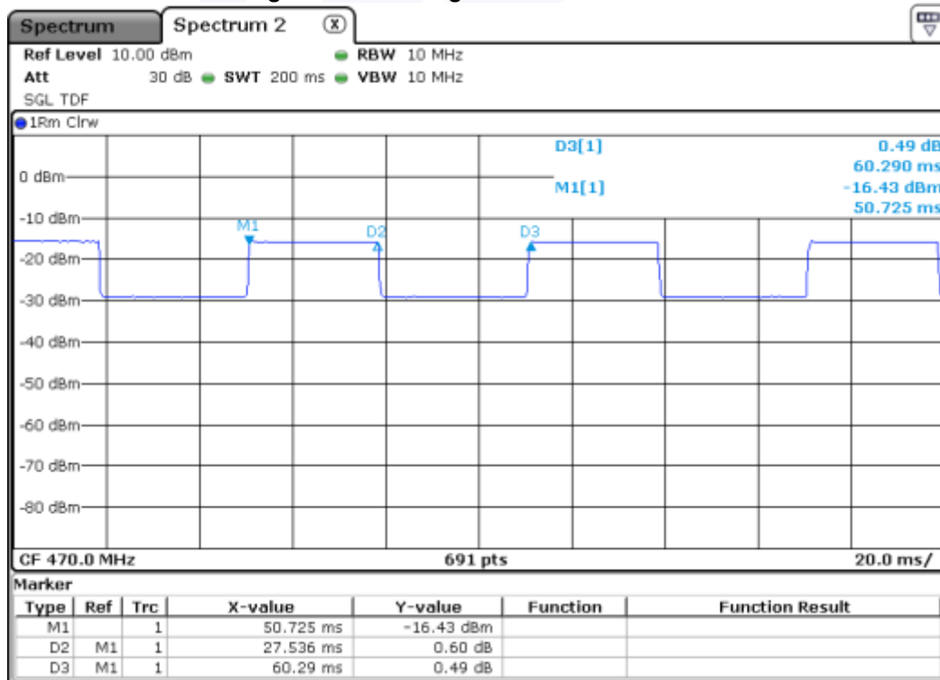
Figure 7-1 UHF Digital Transmission Plot
