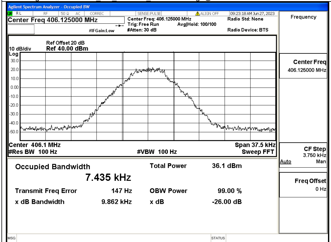
Digital-450.5MHz_1W_12.5KHz_Normal Voltage@OBW and -26dB Bandwidth
