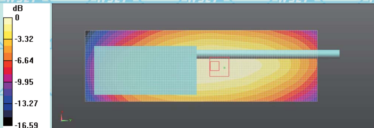
Figure 2: Face held for 4FSK Modulation at 12.5 KHz Channel Separation Front towards Phantom 450.50 MHz
