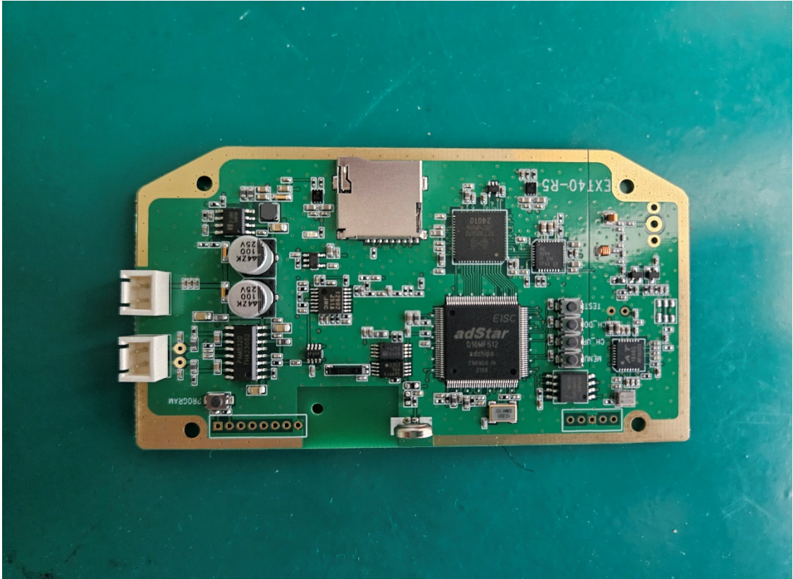
Board-Front
