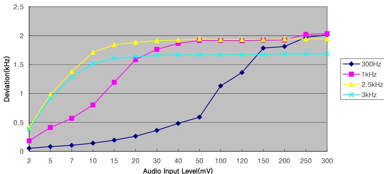
Deviation Limiting
