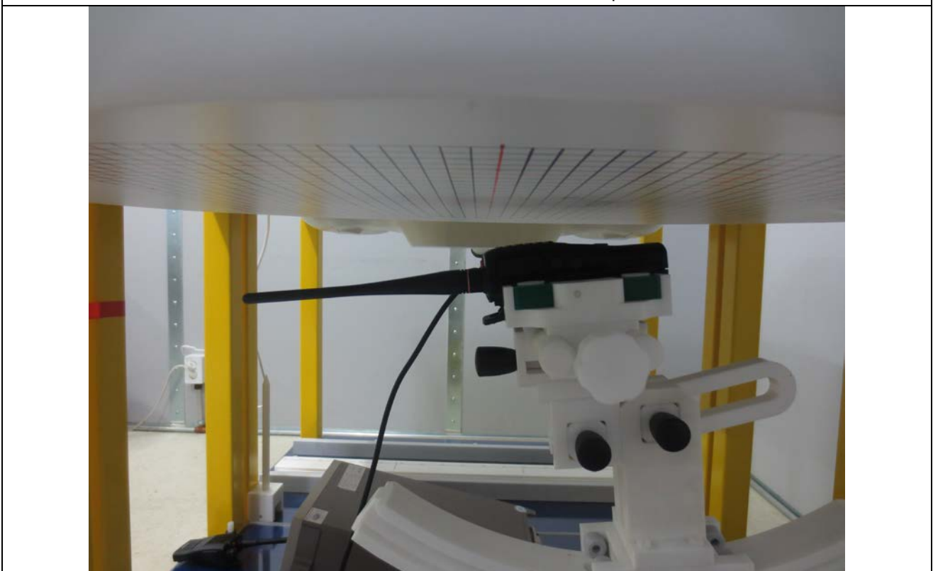
Front of Device 10 mm from Phantom Side view
