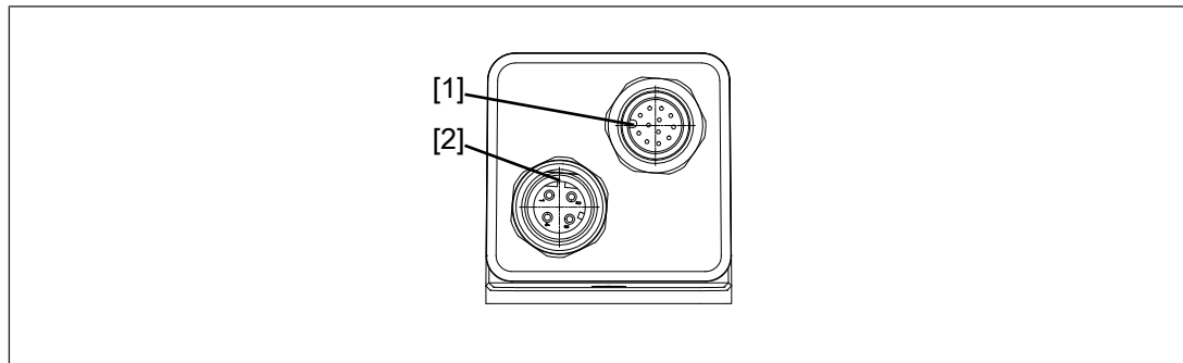
Fig.: View of the PIT gb with PITreader from the connector end: Position of the coding elements on the connectors to protect the cables from twisting.
