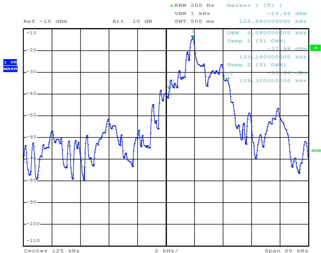
Plot 1: 20dB (99%) – bandwidth
