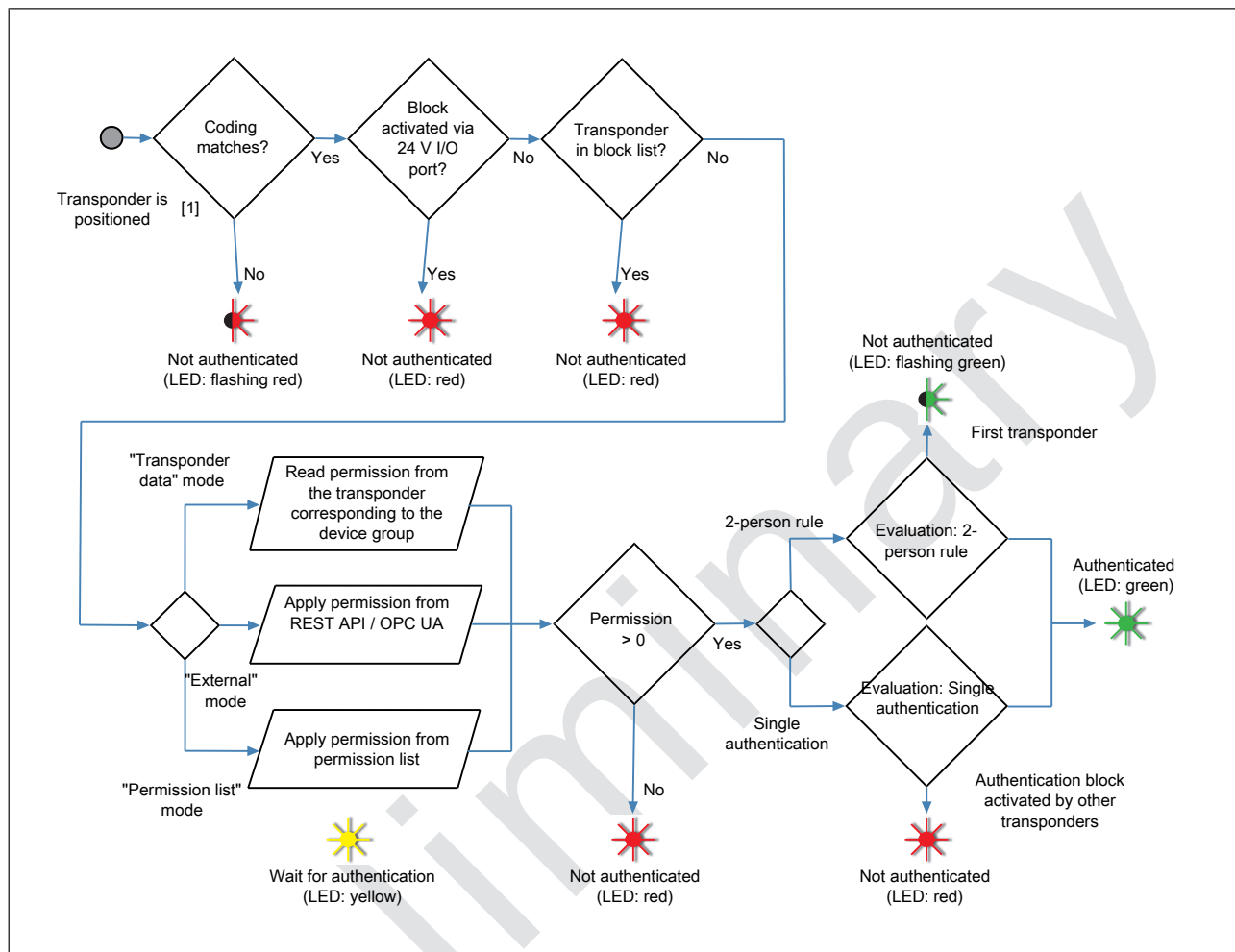
Fig.: Authentication procedure
