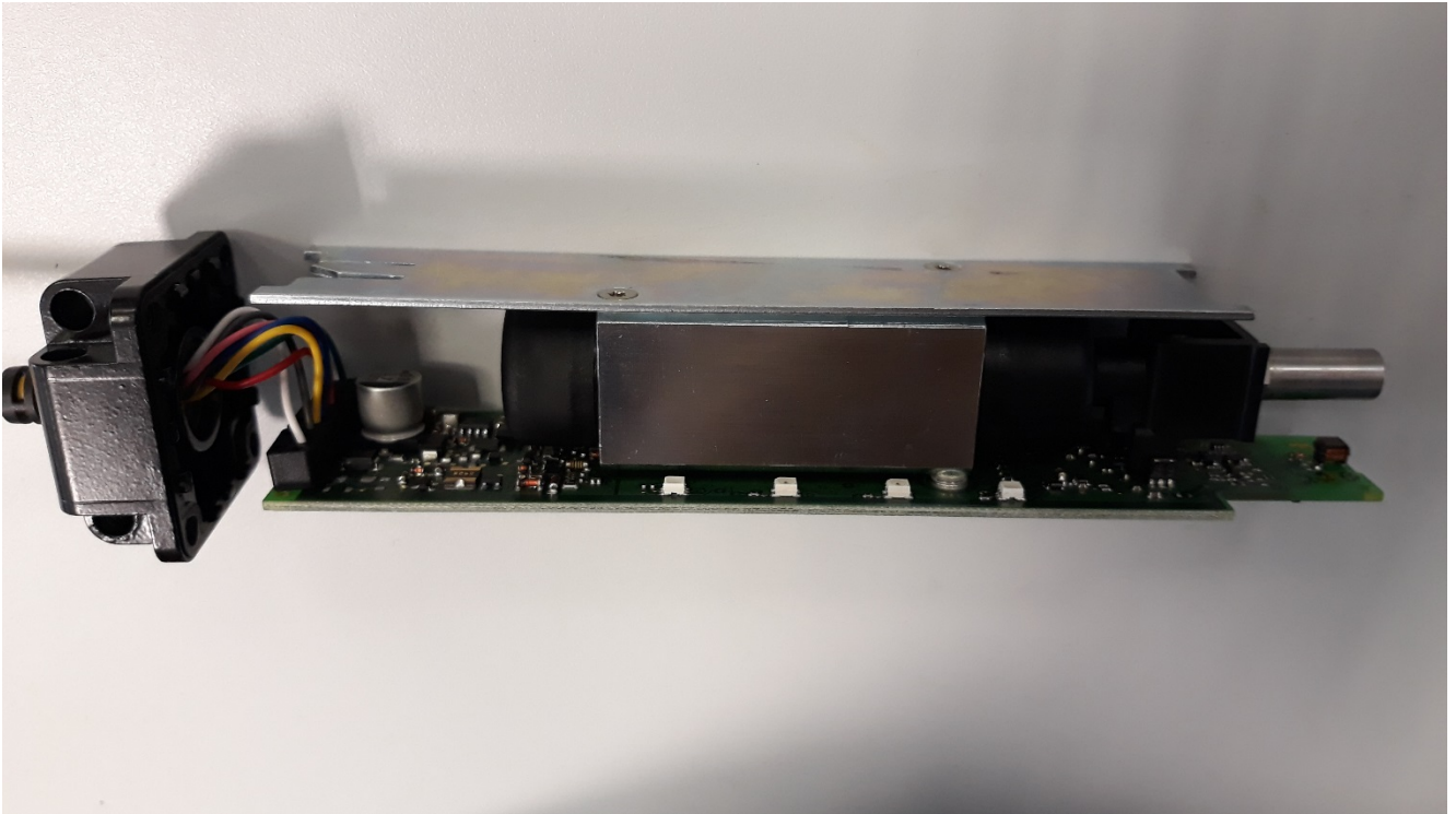
Photo 5: PCB with lifting magnet
