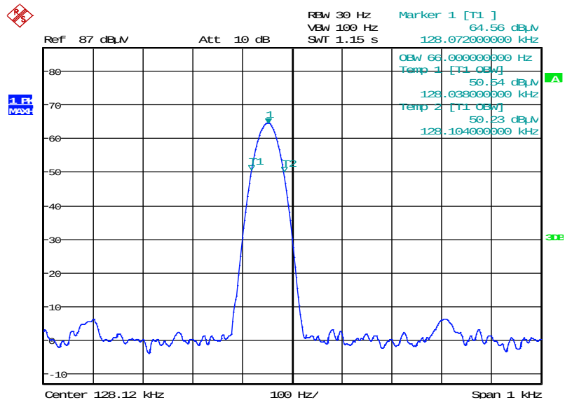
Plot 1: 99 % emission bandwidth zoomed
