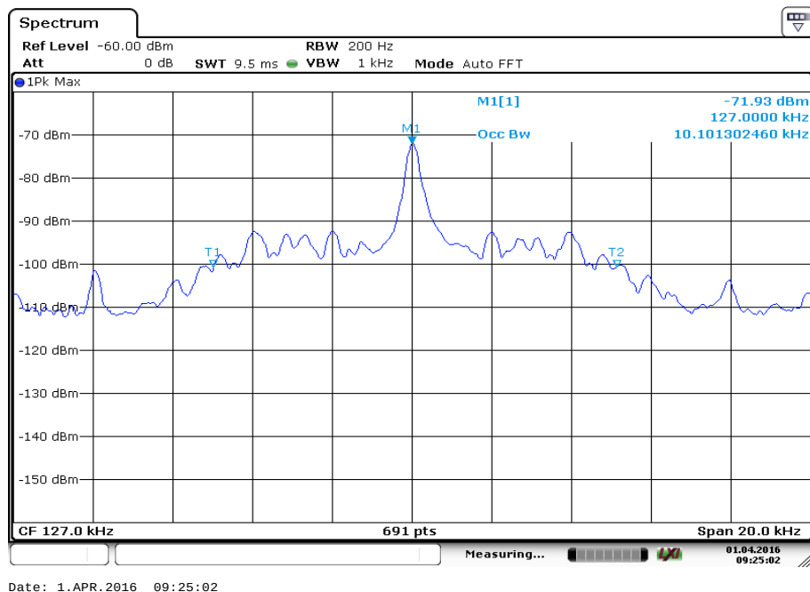
Plot 1: 99% – bandwidth
