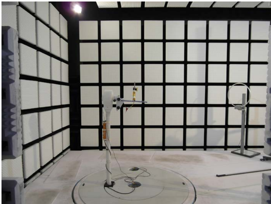
Photo 1: Test setup for radiated emissions
