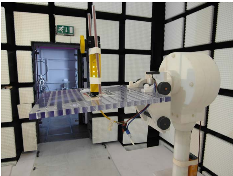
Photo 6: Test setup for radiated emissions
