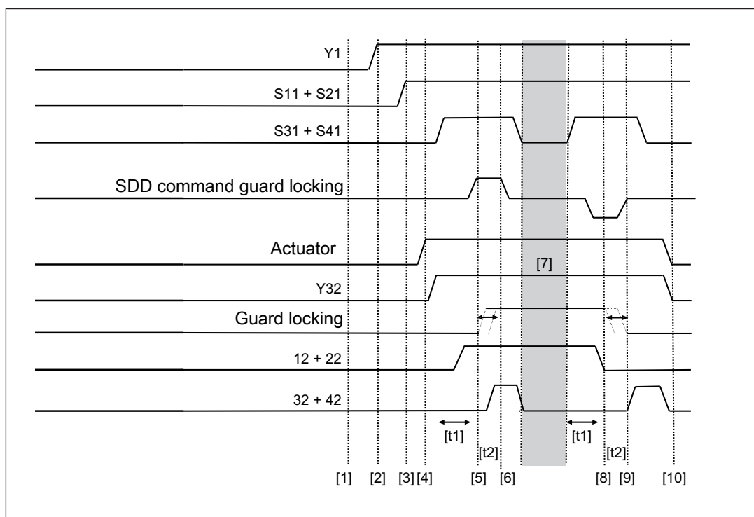
Fig.: Active use of Safety Device Diagnostics
