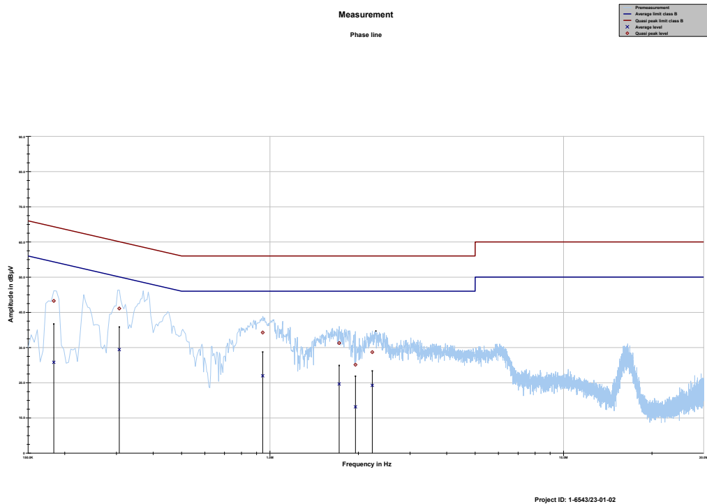
Plot 1: 150 kHz to 30 MHz, phase line
