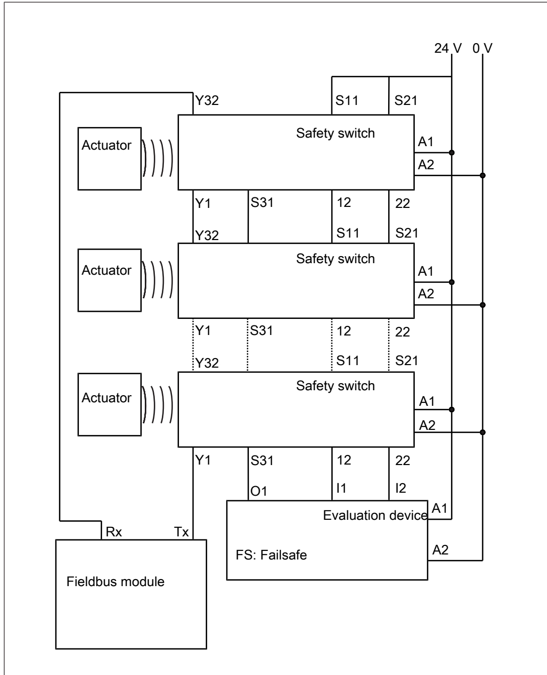
Connection diagram, series connection with SDD (IP67)
