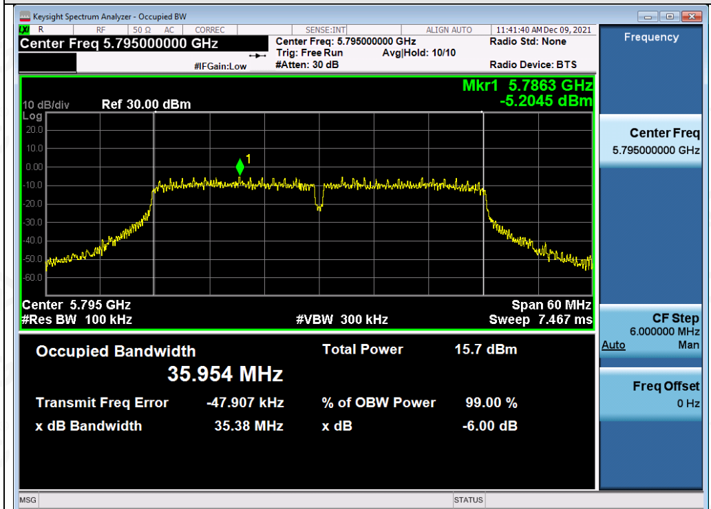
Test_Graph_802.11n40_ANT1_5795_MCS0_DTSBW
