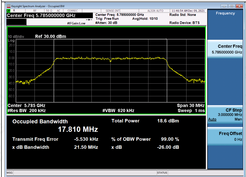
Test_Graph_802.11ac20_ANT1_5785_MCS0_OBW
