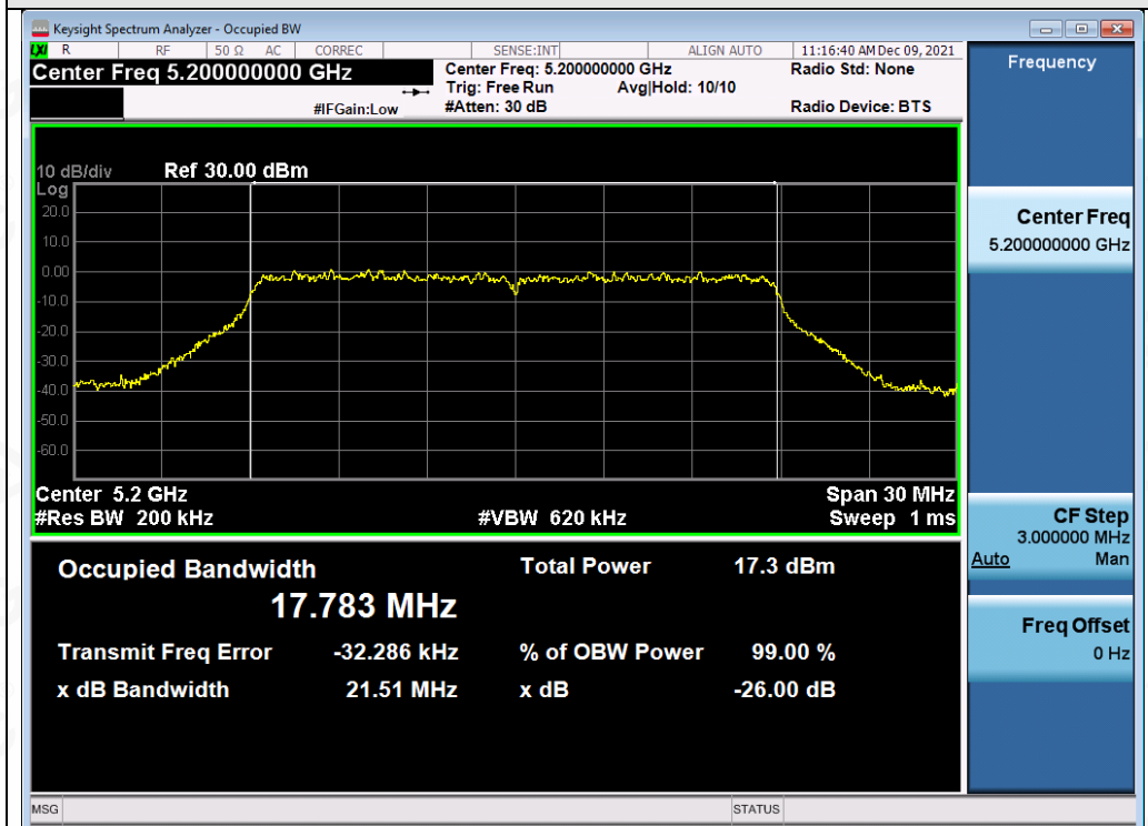
Test_Graph_802.11ac20_ANT1_5200_MCS0_OBW
