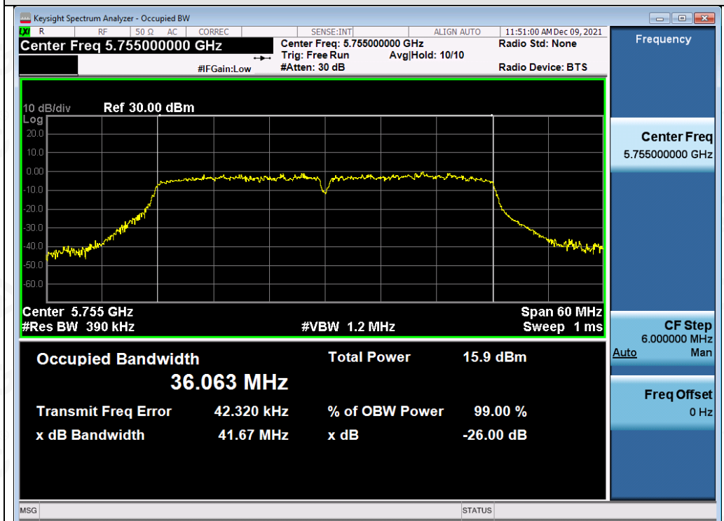
Test_Graph_802.11ac40_ANT1_5755_MCS9_OBW
