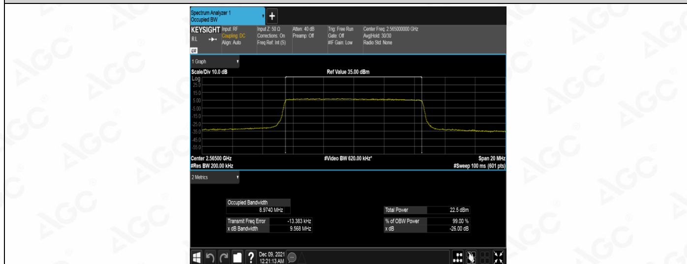
Band7-10MHz-16QAM-20800-50RB#0
