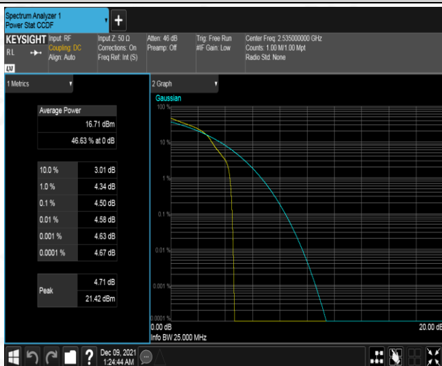
Band7-20MHz-16QAM-21100-1RB#0
