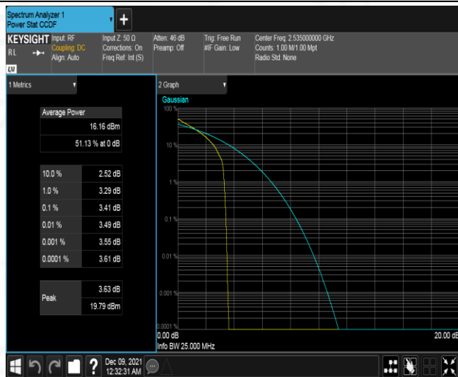
Band7-10MHz-QPSK-21100-1RB#0
