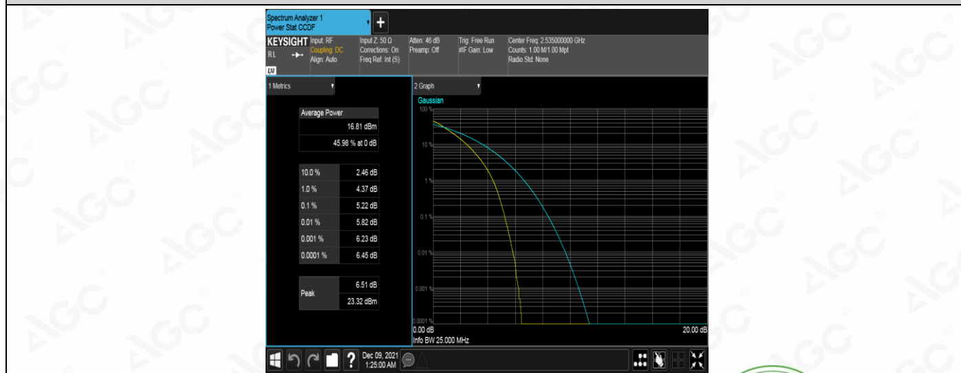
Band7-20MHz-QPSK-21100-100RB#0
