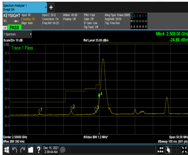
Band7-20MHz-16QAM-20850-1RB#99
