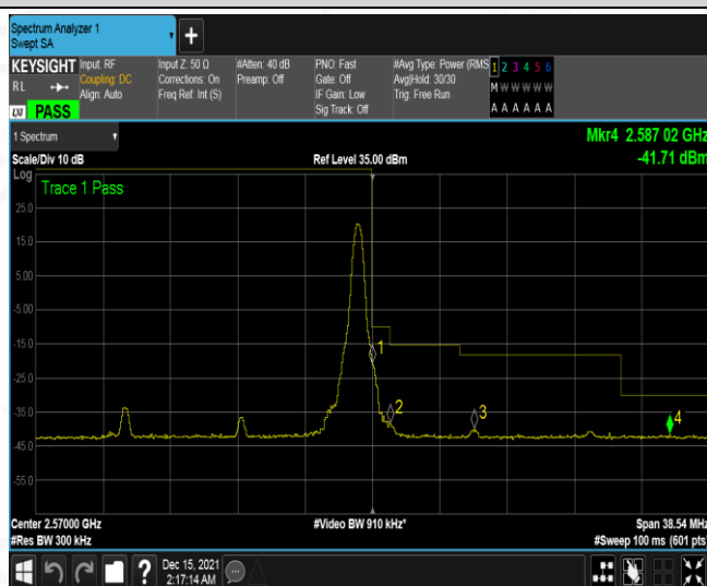
Band7-15MHz-16QAM-21375-1RB#74
