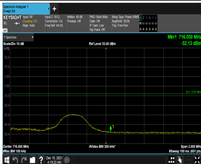
Band17-5MHz-QPSK-23825-1RB#24
