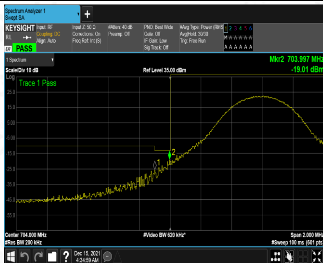
Band17-10MHz-16QAM-23780-1RB#49
