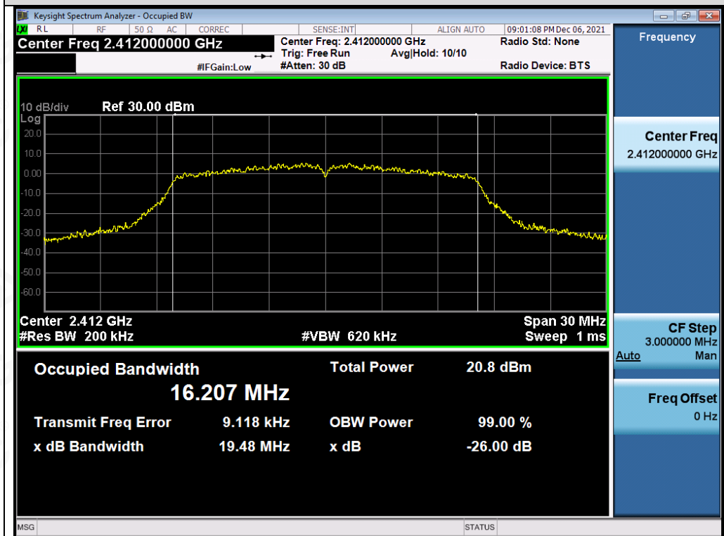
Test Graph 802.11g ANT1 2412 6Mbps OBW
