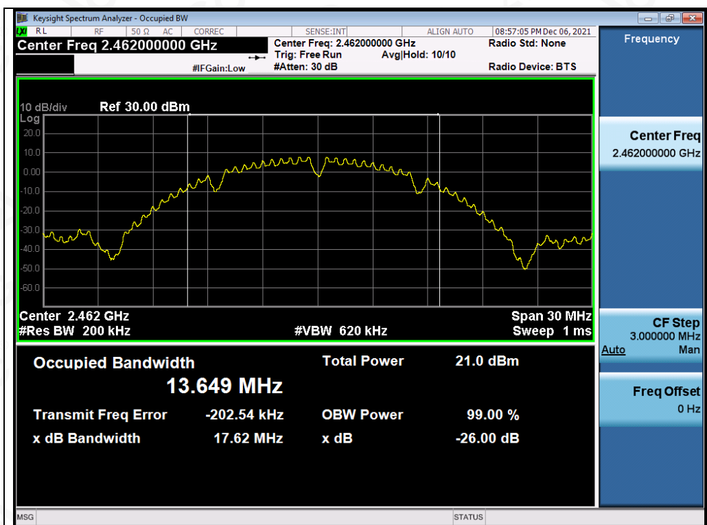
Test Graph 802.11b ANT1 2462 1Mbps OBW
