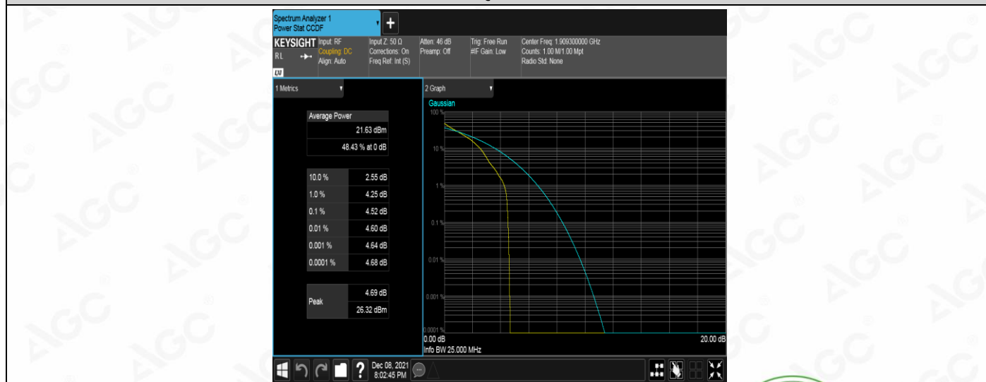
Band2-1.4MHz-QPSK-19193-1RB#0
