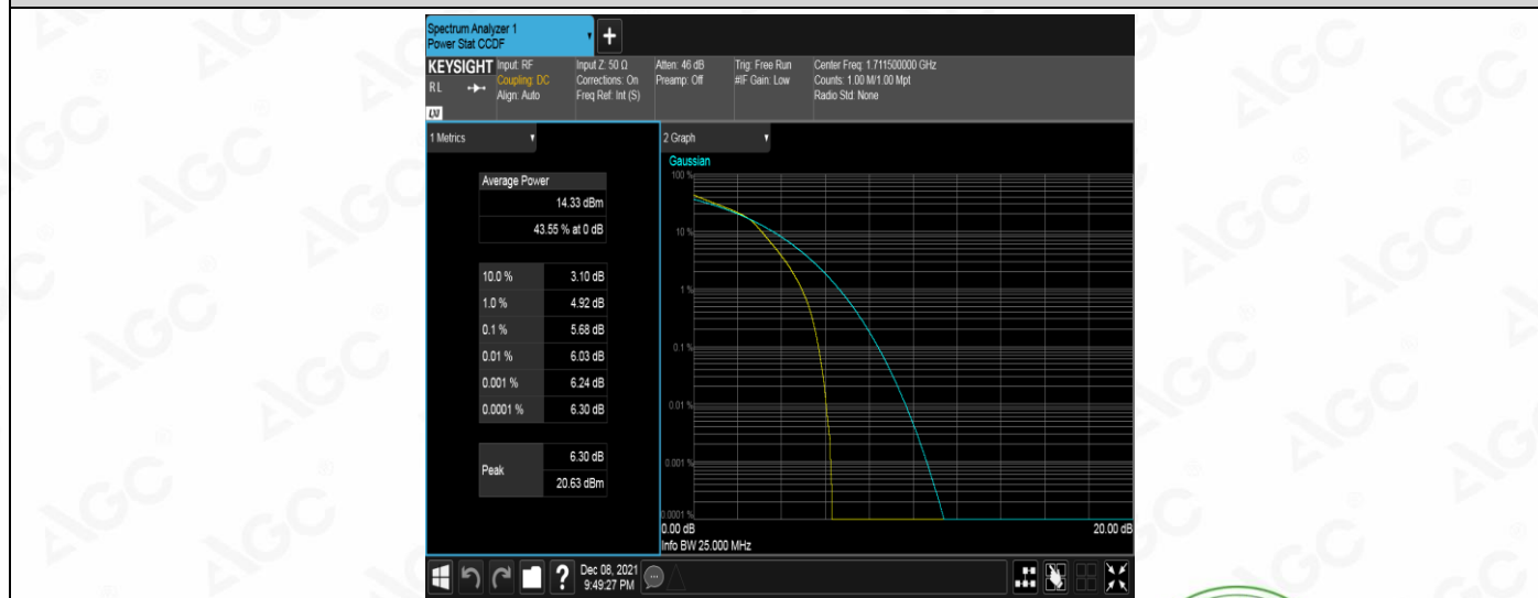
Band4-3MHz-16QAM-19965-15RB#0
