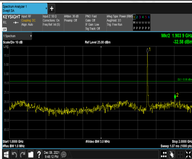
Band4-3MHz-16QAM-20385-1RB#0-Range2:1000~2000MHz
