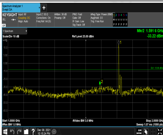
Band4-10MHz-16QAM-20000-1RB#0-Range2:1000~2000MHz
