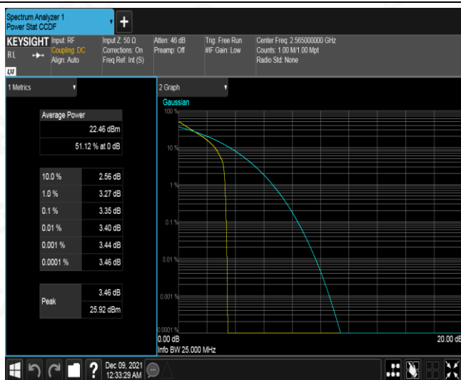
Band7-10MHz-QPSK-21400-50RB#0
