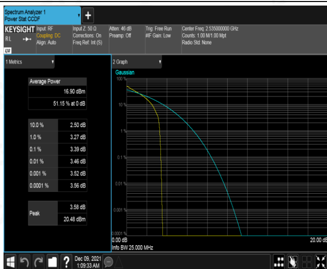
Band7-15MHz-QPSK-21100-75RB#0
